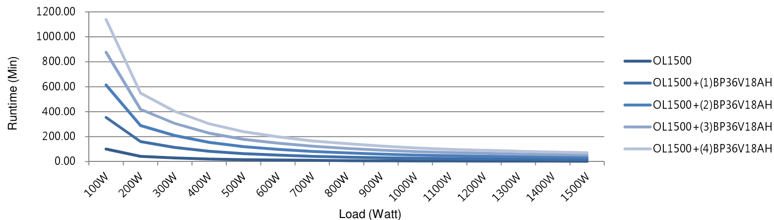
OL1500 Runtime Chart
