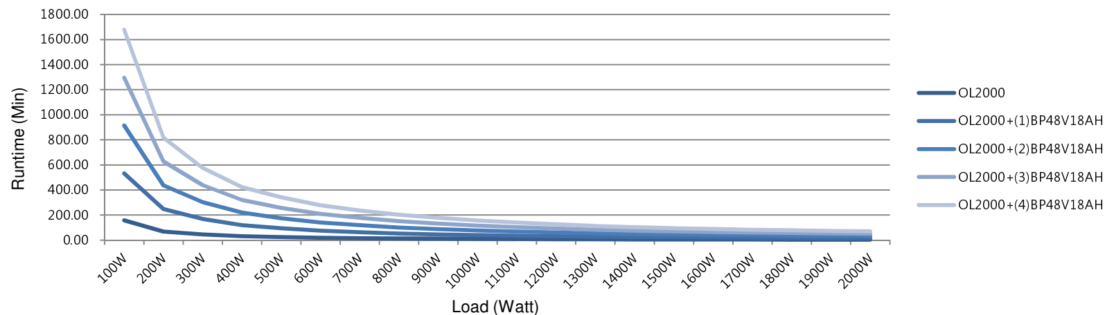
OL2000 Runtime Chart
