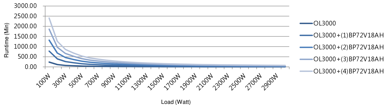
OL3000 Runtime Chart
