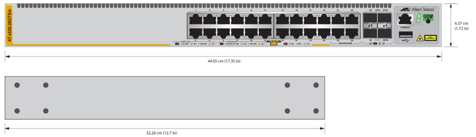
Figure 59. x530-28GTXm Dimensions
