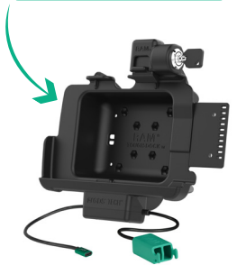
RAM-GDS-DOCKKL-ZE20PD2U GDS® Vehicle Dock Locking Power + Dual USB
