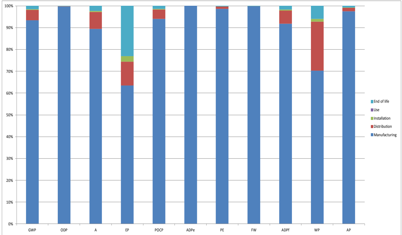
% ENVIRONMENTAL IMPACT PER LIFE CYCLE STAGE OF REFERENCE PRODUCT
