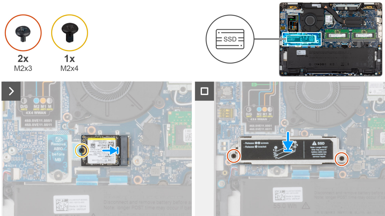
Figure 36. Installing the M.2 2230 SSD
