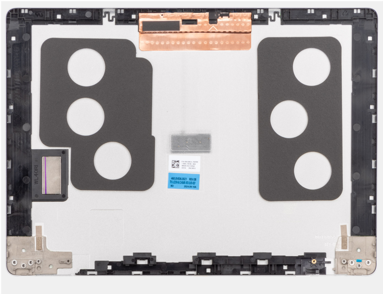
Figure 85. Installing the display back cover
