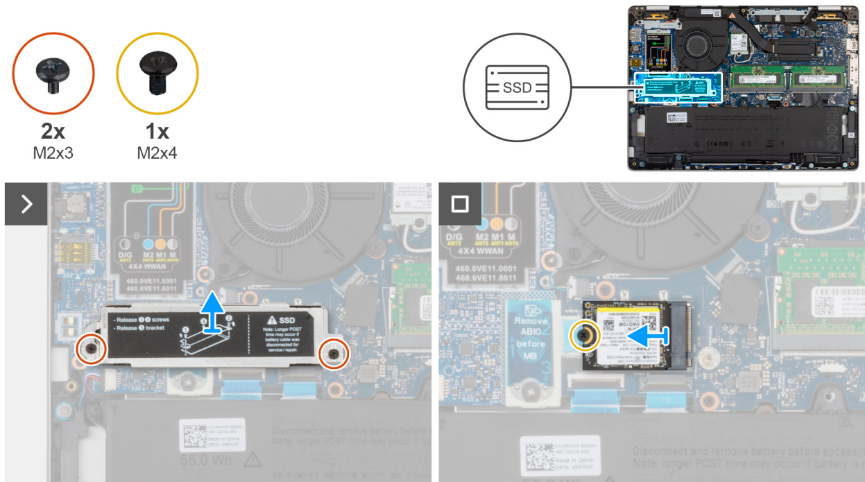
Figure 35. Removing the M.2 2230 SSD
