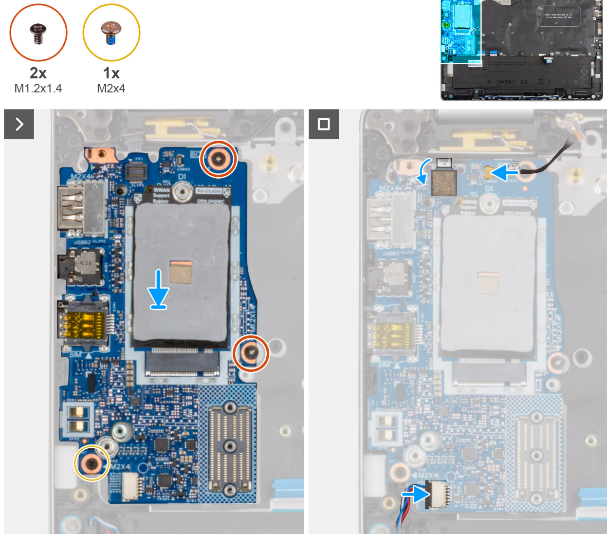
Figure 63. Installing the I/O board
