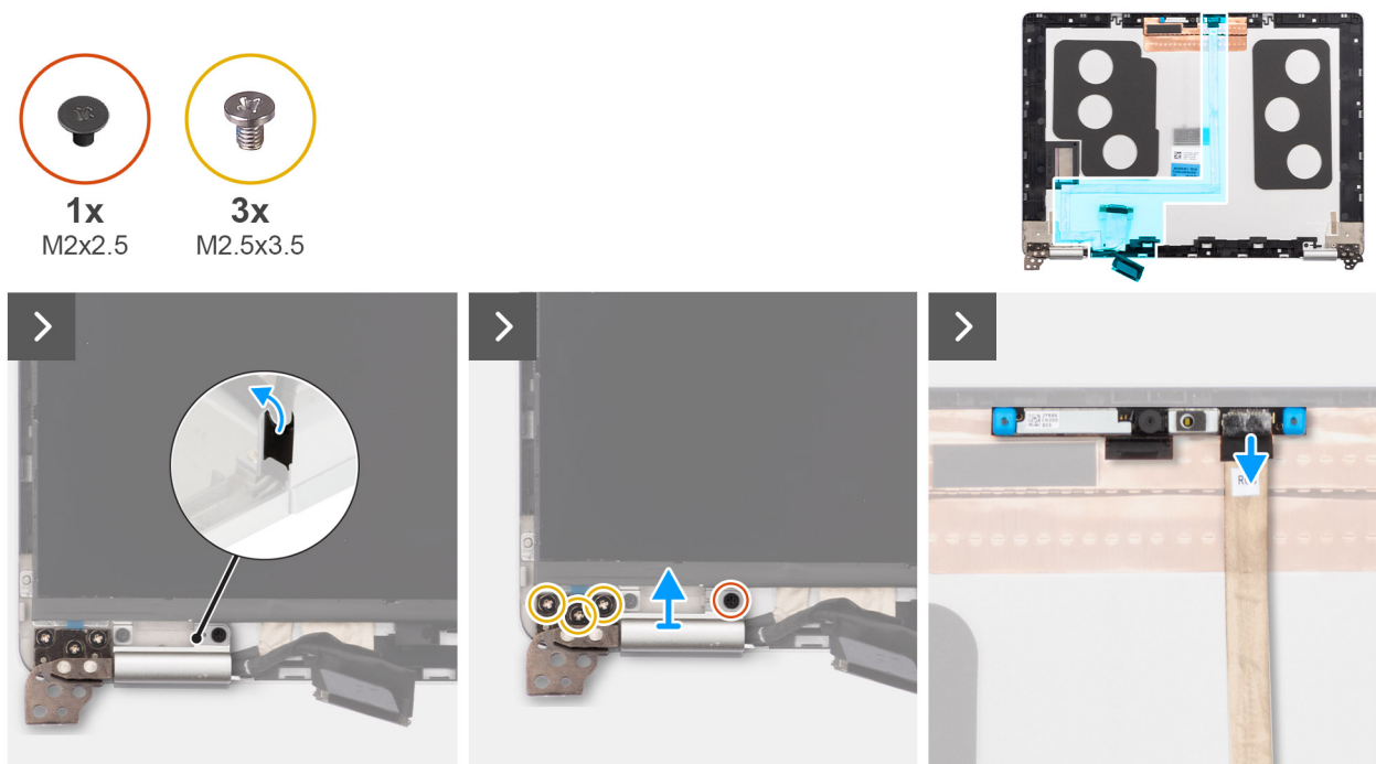
Figure 80. Removing the display cable
