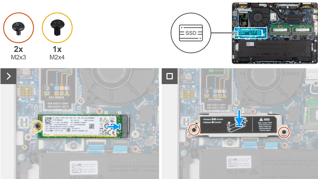
Figure 38. Installing the M.2 2280 SSD
