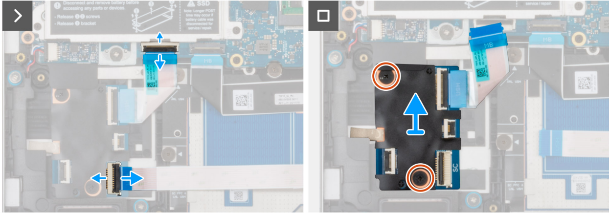
Figure 43. Removing the USH board
