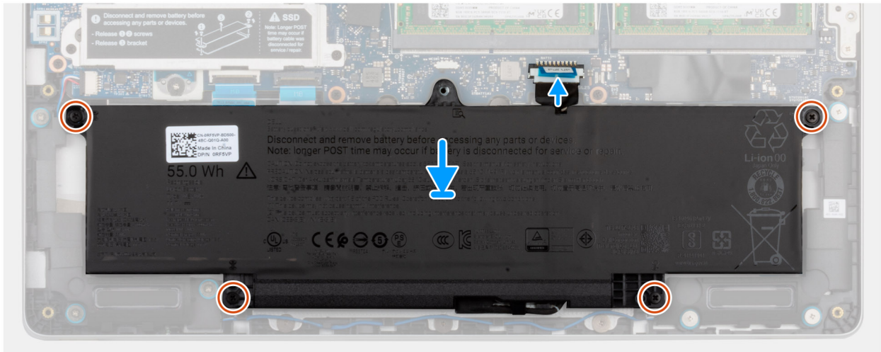
Figure 24. Installing the battery
