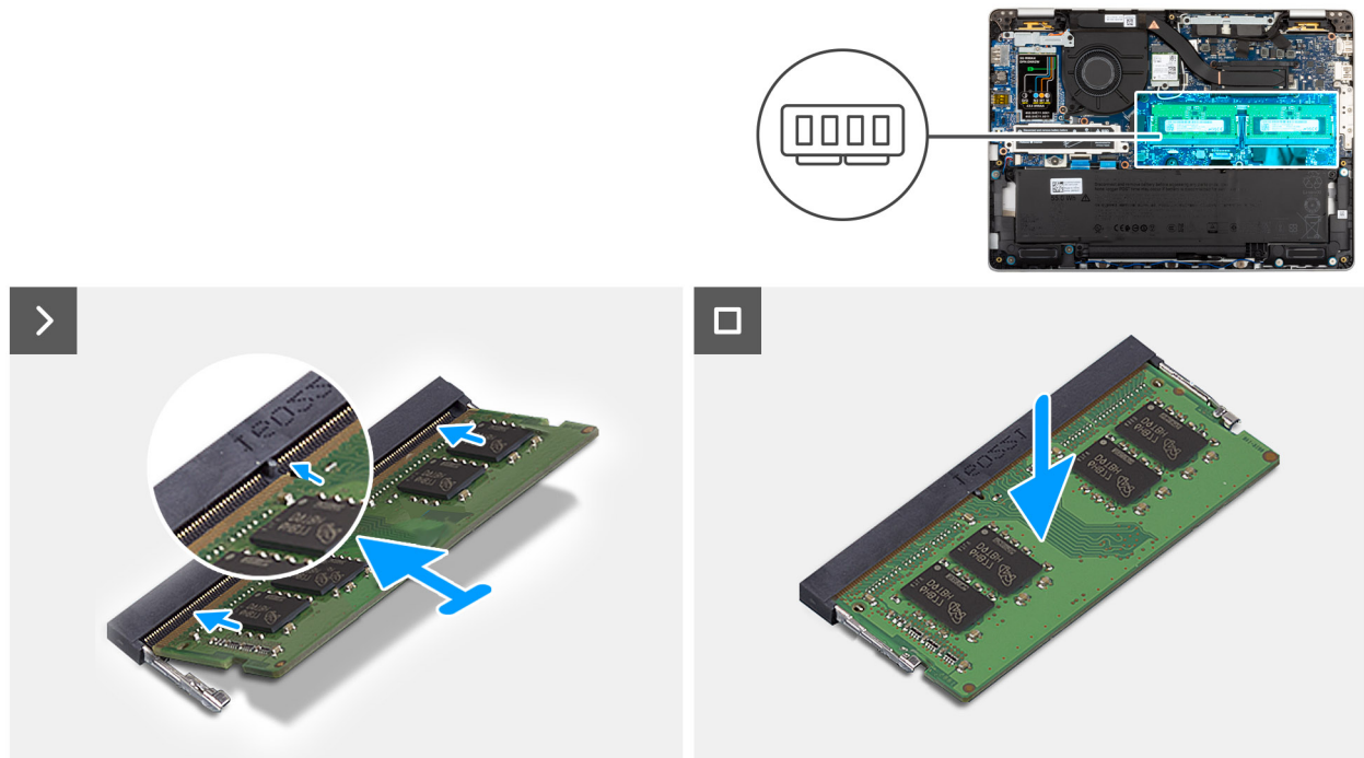
Figure 28. Installing the memory modules
