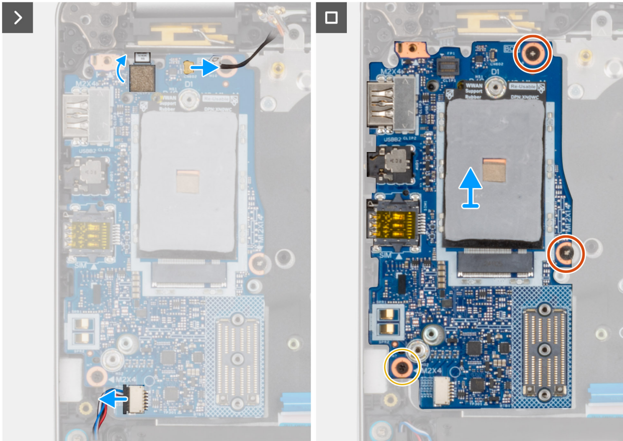
Figure 62. Image: Removing the I/O board
