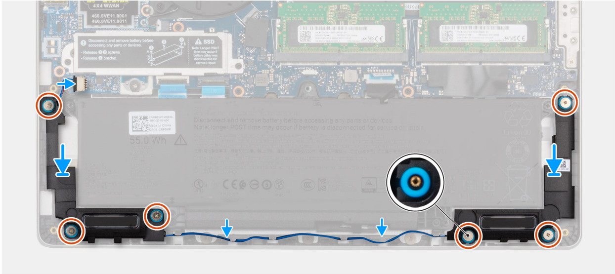
Figure 40. Installing the speakers
