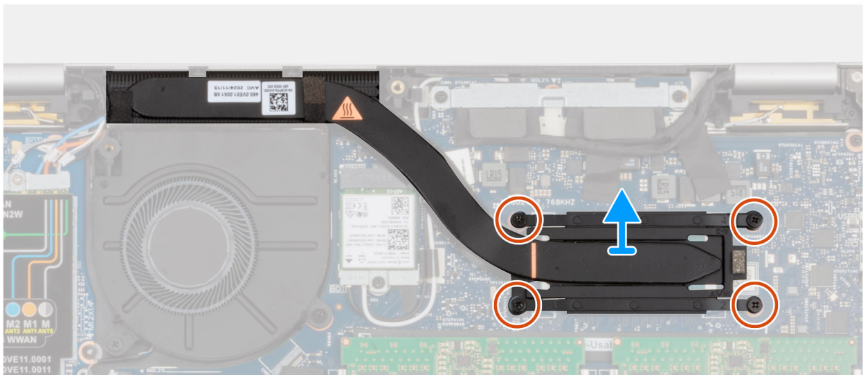
Figure 48. Removing the heat sink
