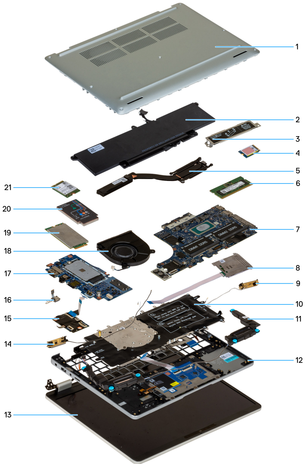
Figure 14. Major Components of your Dell Pro 13 Plus
