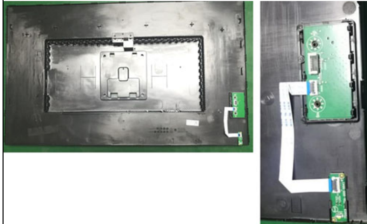
Disconnect the pins to remove the key board and the LED board
