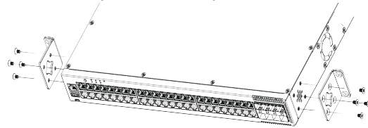
Figure 3 5320-16P Flush-Mount
