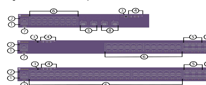
Figure 10 5320 Series: Sample Front Panels
