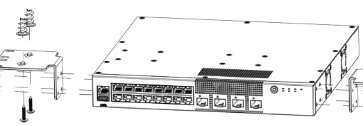
Figure 7 5320-16P Table Mount
