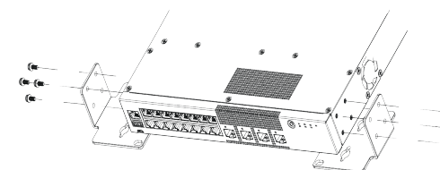
Figure 9 5320-16P Alternate Mount Ear Attachment
