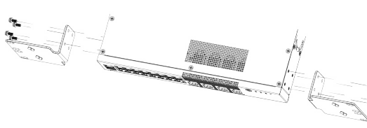
Figure 4 5320-16P Mid-Mount
