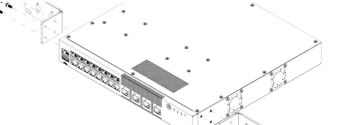
Figure 6 5320-16P 1U Mid-Mount
