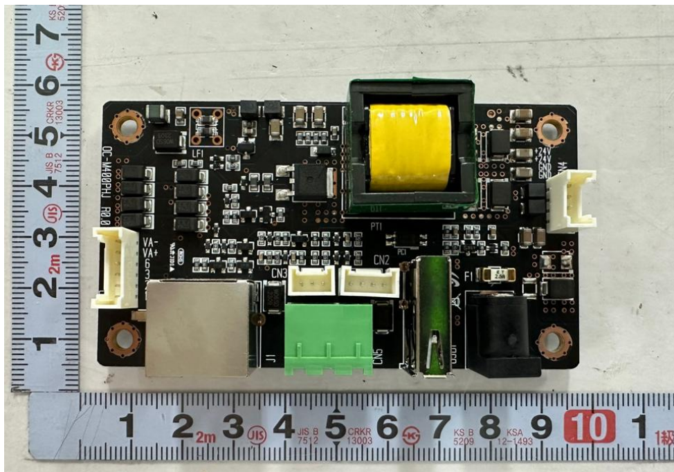
<Photo 6 > PoE board
