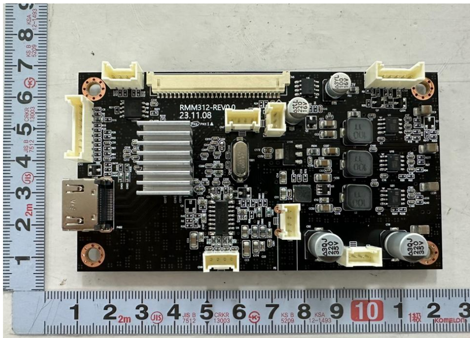
<Photo 8 > RMM312 board
