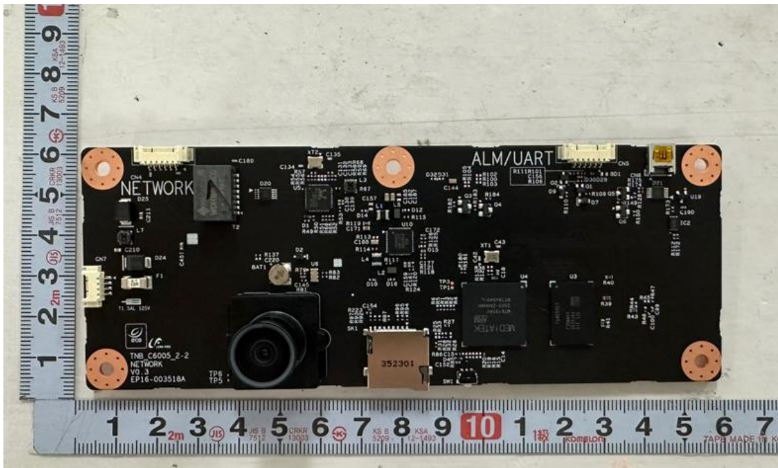
<Photo 4 > Network board
