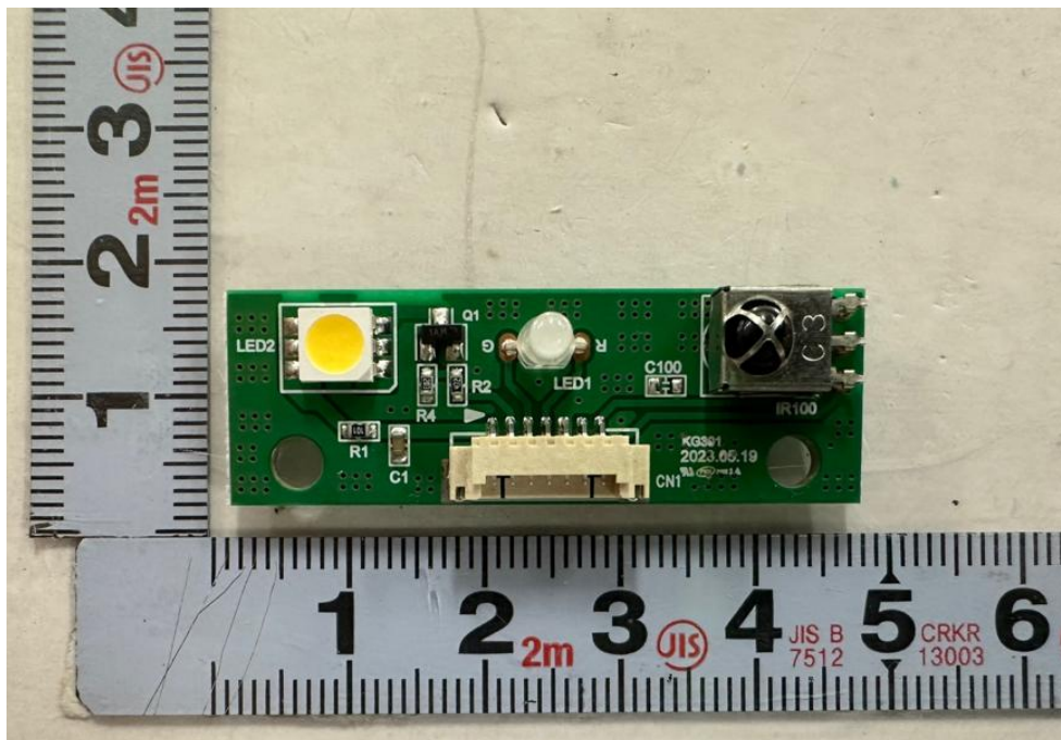
<Photo 10 > KG301 board
