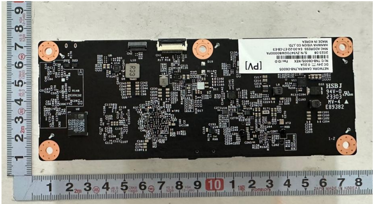
<Photo 5 > Network board
