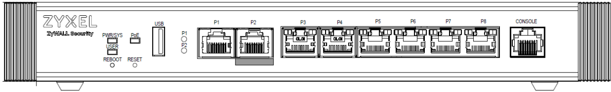
Figure 36 USG FLEX 500H Front Panel
