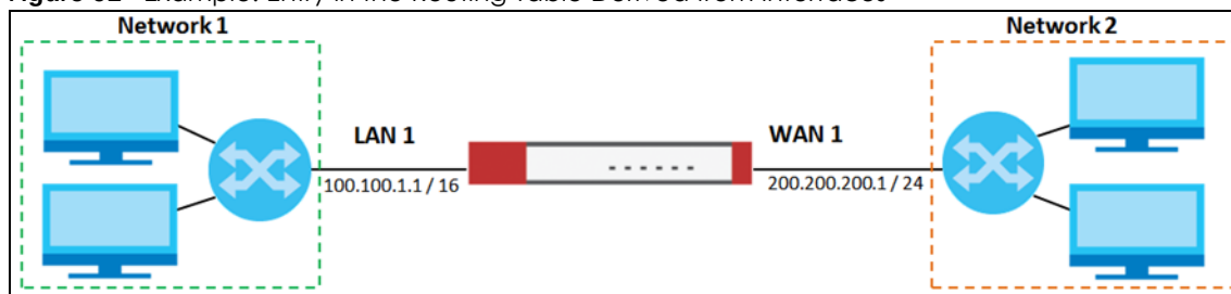
Figure 91 Example: Entry in the Routing Table Derived from Interfaces
