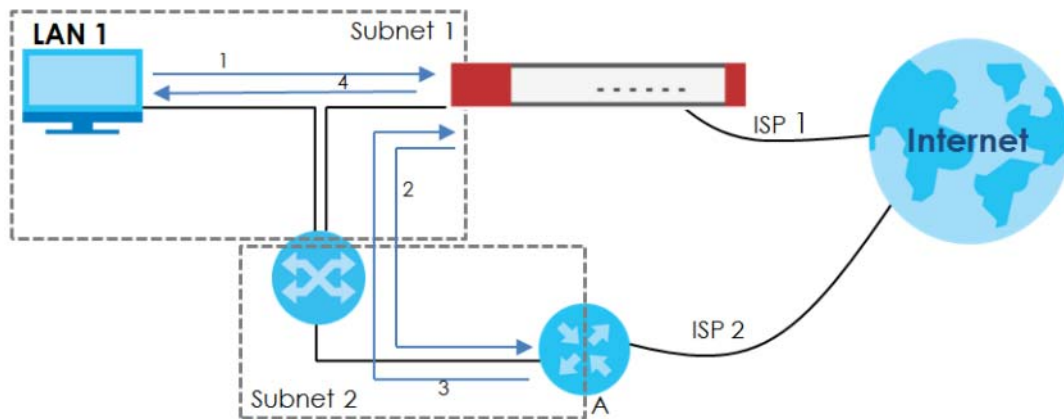
Figure 152 Using Virtual Interfaces to Avoid Asymmetrical Routes
