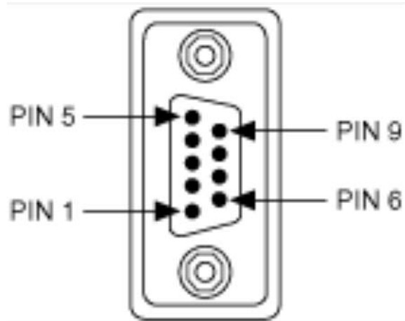
Figure 47 DB-9 Connector Pins
