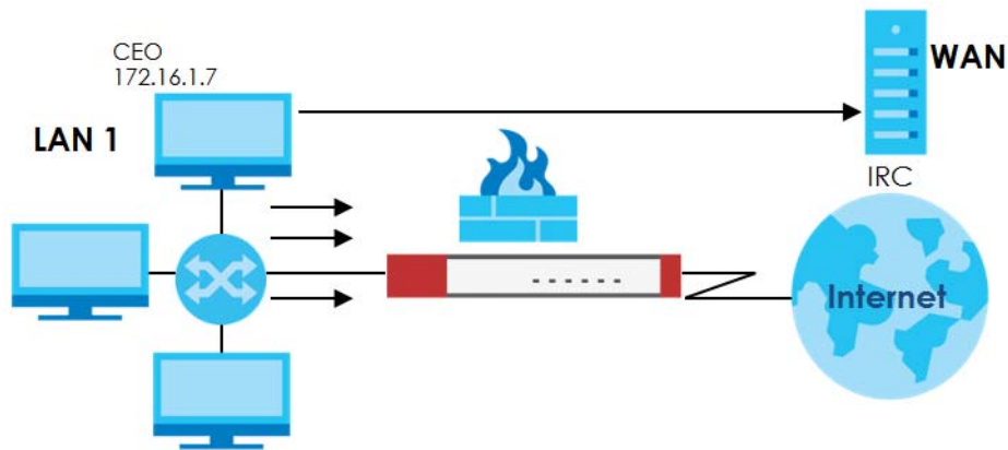
Figure 164 Limited LAN to WAN IRC Traffic Example
