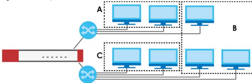
Figure 92 Example: Before VLAN
