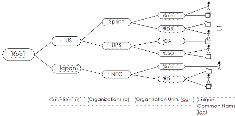
Figure 240 Basic Directory Structure
