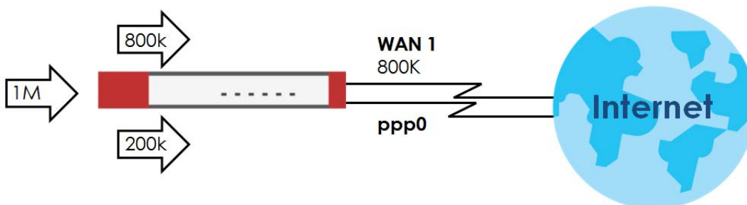
Figure 105 Spillover Algorithm Example
