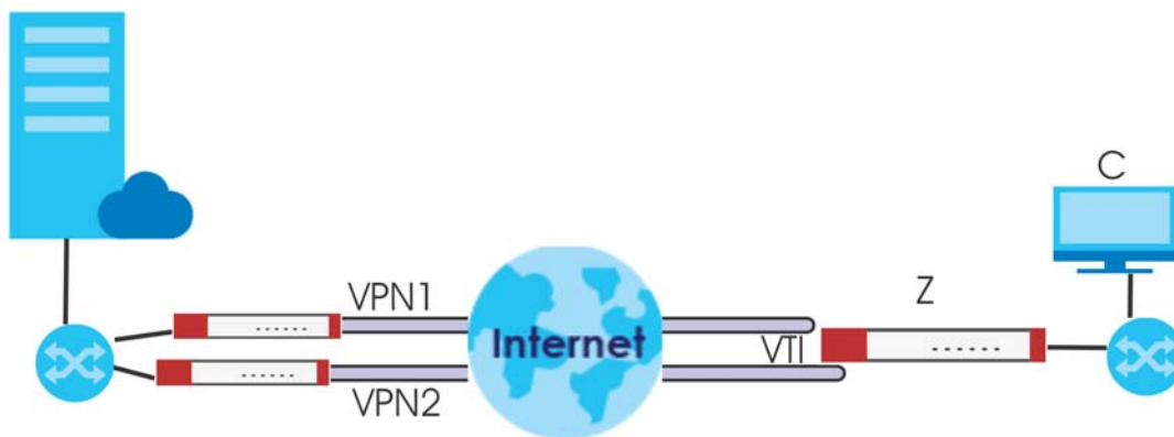
Figure 101 VTI and Trunk for VPN Load Balancing
