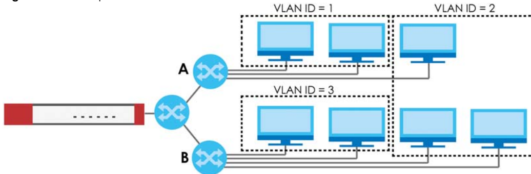
Figure 93 Example: After VLAN
