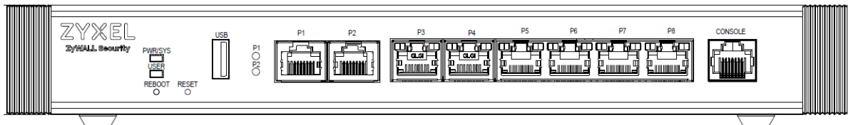
Figure 34 USG FLEX 200H Front Panel
