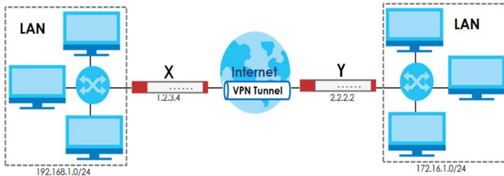
Figure 137 Site-to-site IPSec VPN Example
