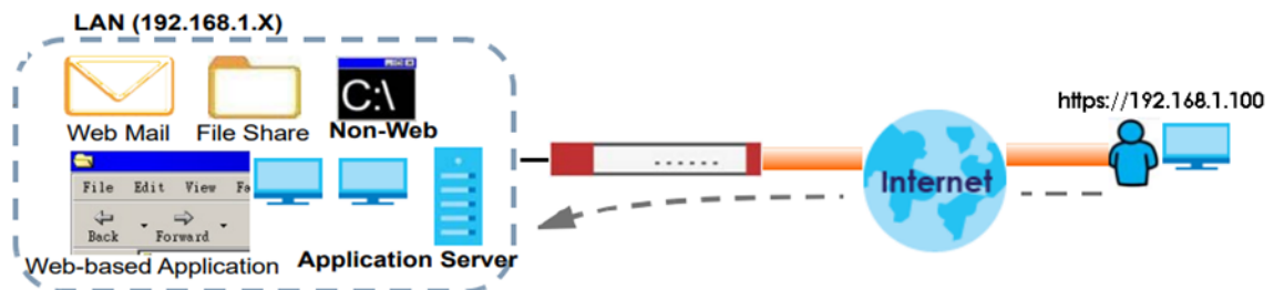
Figure 148 Network Access Mode: Full Tunnel Mode
