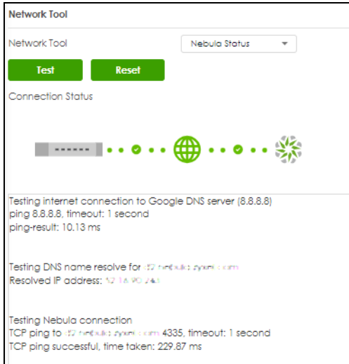
Figure 293 Maintenance > Diagnostics > Network Tool > Nebula Status
