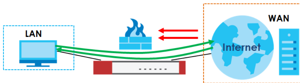
Figure 151 Default Directional Security Policy Example
