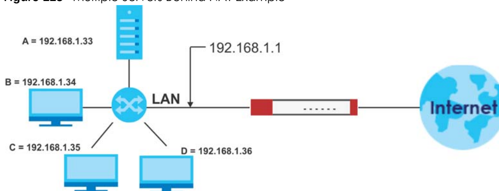
Figure 115 Multiple Servers Behind NAT Example
