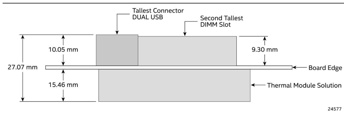
Figure 16. Board Height Dimensions
