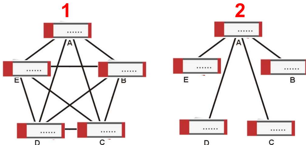
Figure 355 VPN Topologies (Fully Meshed and Hub and Spoke)
