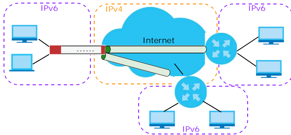
Figure 259 6to4 Tunnel
