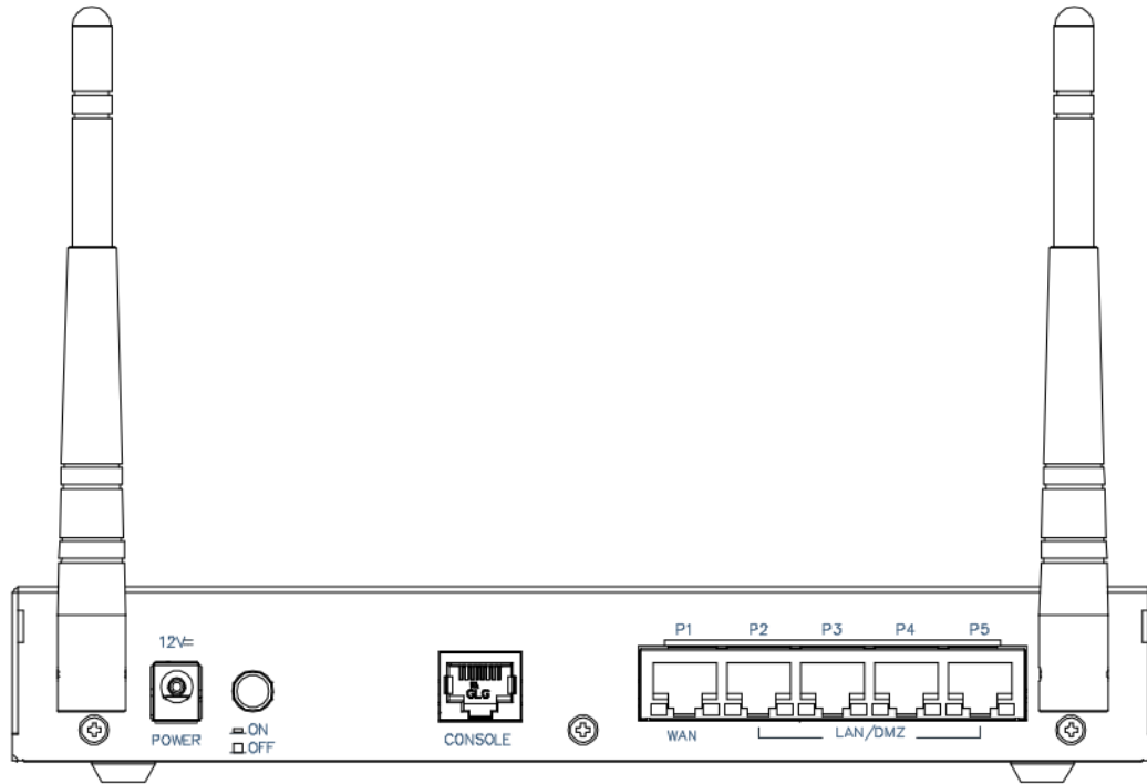
Figure 65 USG FLEX 50AX Rear Panel
