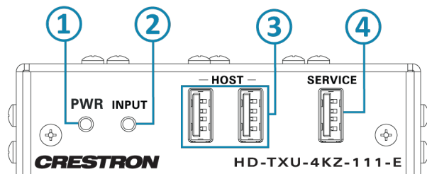
HD-TXU-4KZ-111-E Transmitter, Front Panel
