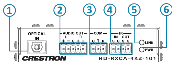
HD-RXCA-4KZ-101 Front Panel
