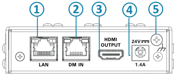
HD-RXU-4KZ-101-E Receiver, Rear Panel
