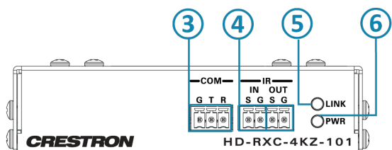
HD-RXC-4KZ-101 Front Panel
