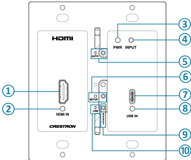
HD-TX-4KZ-211-2G, Front
