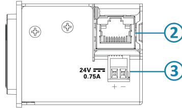
1G Wall Plate Transmitter, Rear, Top View
