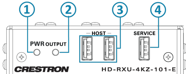
HD-RXU-4KZ-101-E Receiver, Front Panel
