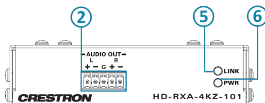
HD-RXA-4KZ-101 Front Panel
