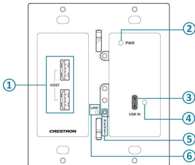
HD-TXU-4KZ-111-2G, Front
