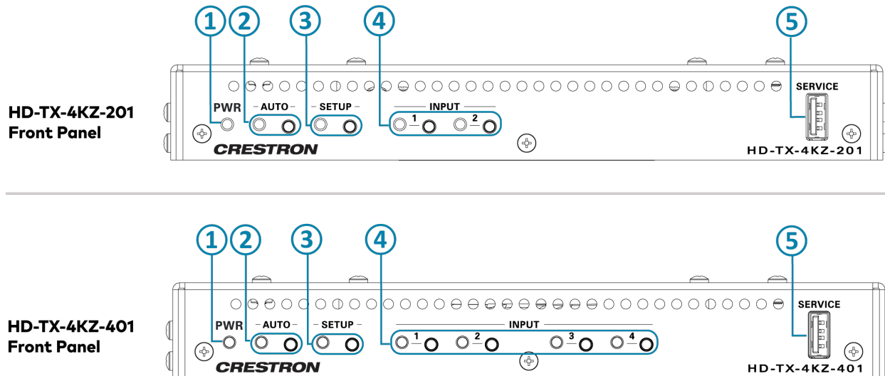
HD-TX-4KZ-201 and HD-TX-4KZ-401 Transmitters, Front Panel
