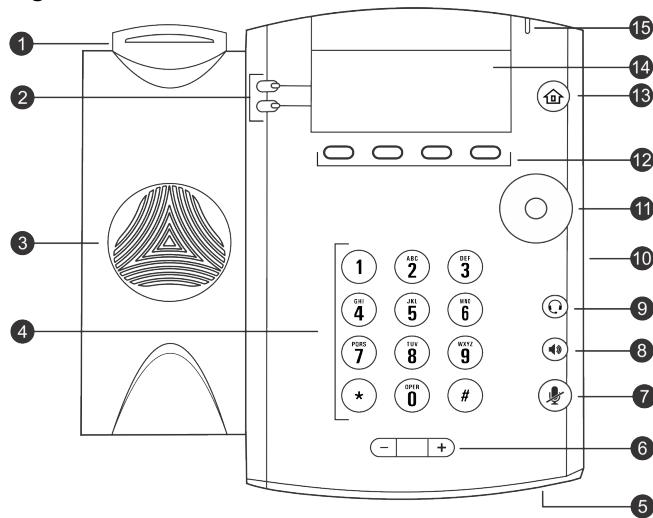
Figure 1: VVX 101 and 201 hardware features
