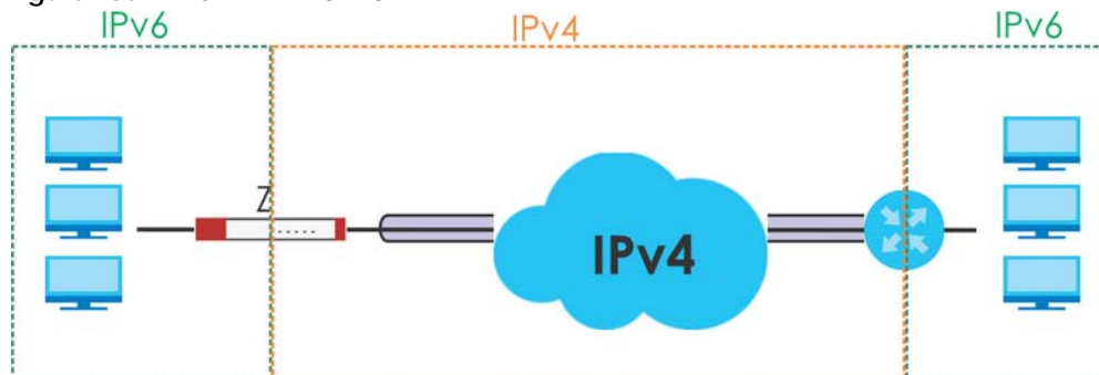
Figure 280 IPv6-in-IPv4 Tunnel
