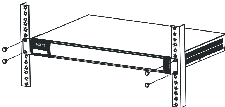
Figure 77 Mount on Rack
