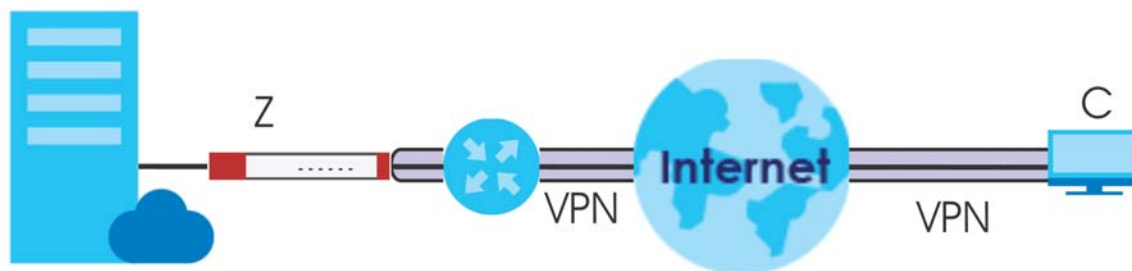
Figure 402 L2TP and Zyxel Device Behind a NAT Router
