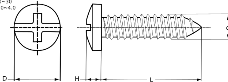
Figure 78 Wall Mounting Screw Specifications
