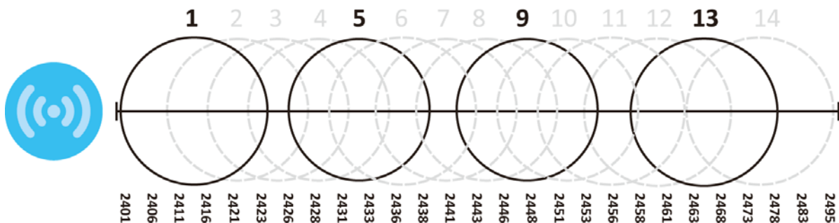
Figure 256 An Alternative Four-Channel Deployment
