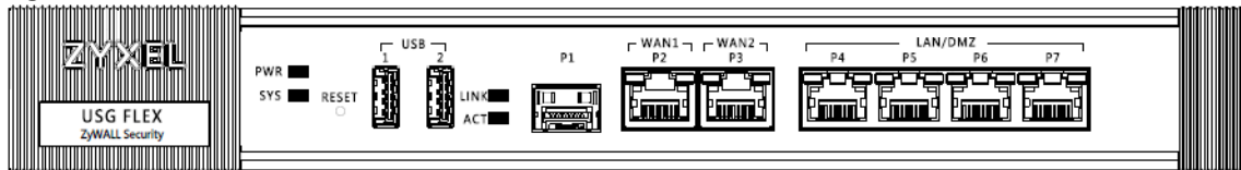
Figure 65 USG FLEX 500 Front Panel
