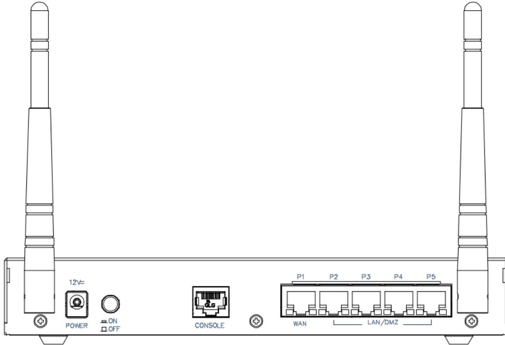
Figure 69 USG FLEX 100W Rear Panel
