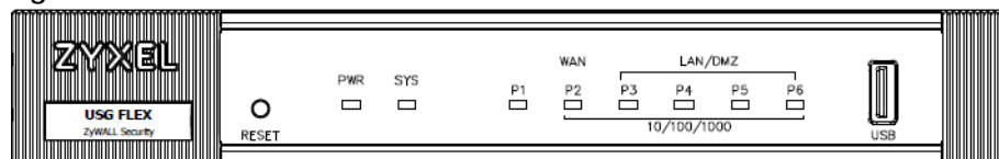
Figure 61 USG FLEX 100 Front Panel
