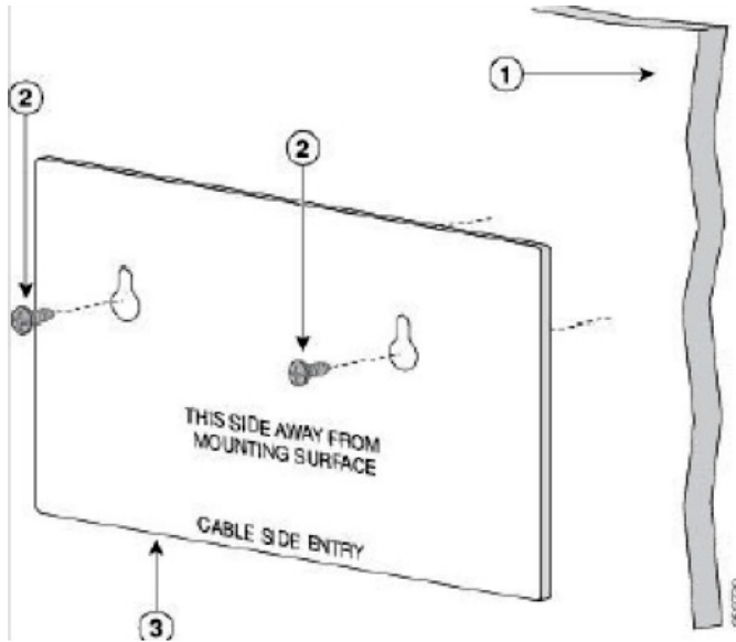
Figure 3 Installing the mounting screws on the wall
