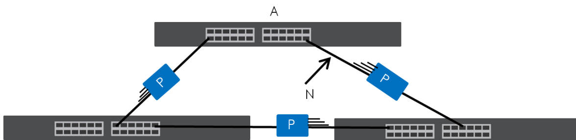
Figure 134 Loop Guard – Network Loop
