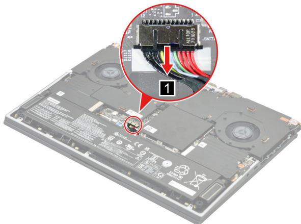
Figure 7. Disconnect the battery pack cable
