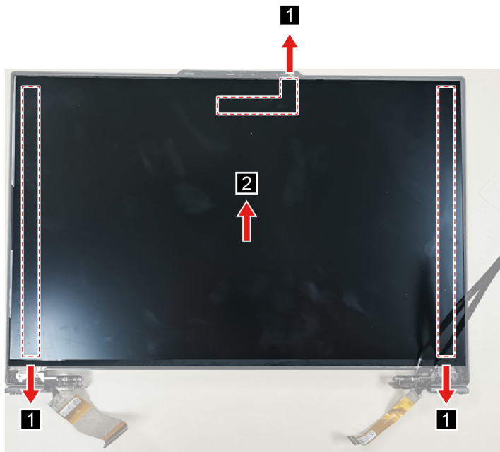
Figure 43. Remove the LCD panel
