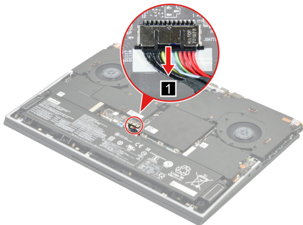
Figure 5. Disconnect the battery pack cable
