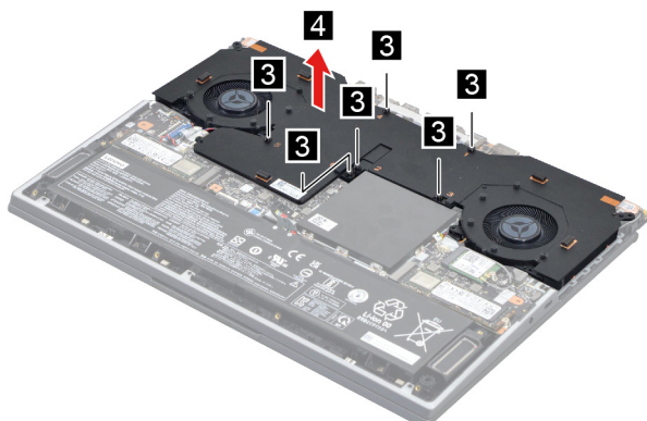
Figure 22. Loosen six screws and then remove the thermal module
