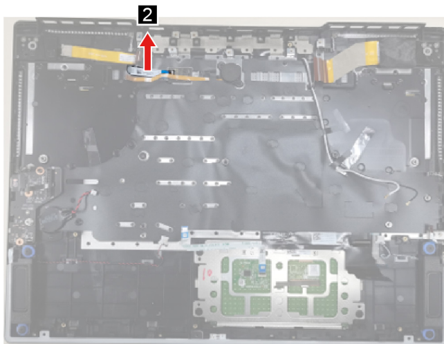
Figure 29. Remove the fingerprint board cable
