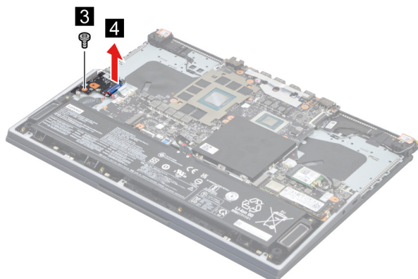
Figure 24. Remove the I/O board
