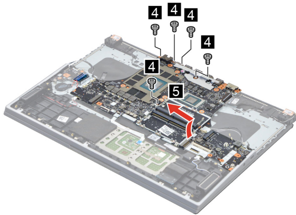
Figure 26. Remove seven screws and then lift the system board
