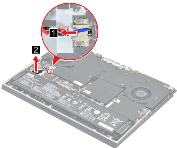
Figure 16. Remove the CMOS battery
