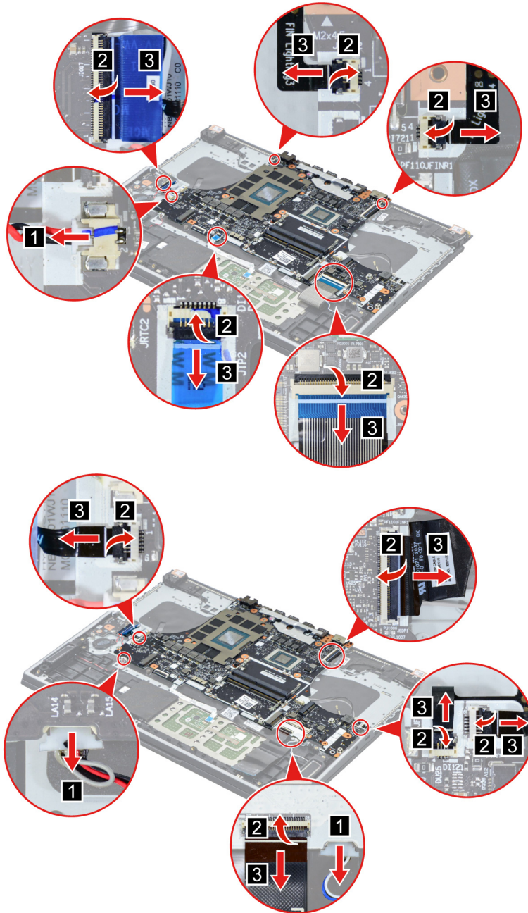
Figure 25. Disconnect cables connected to the system board
