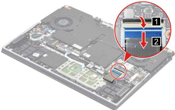
Figure 19. Disconnect the keyboard cable
