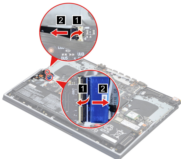
Figure 23. Disconnect the cables
