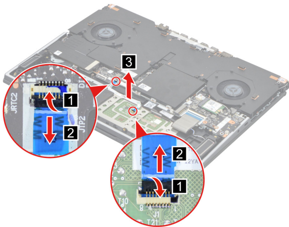
Figure 17. Remove the touchpad board cable
