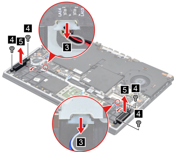
Figure 20. Remove the speakers
