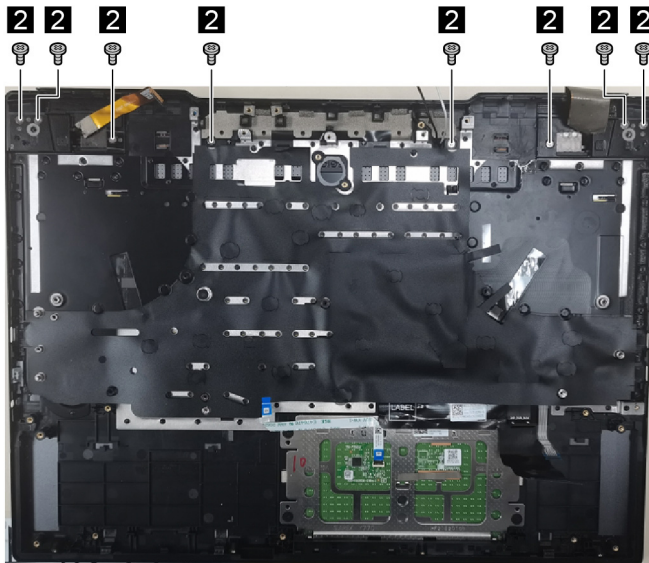
Figure 32. Remove two screws
