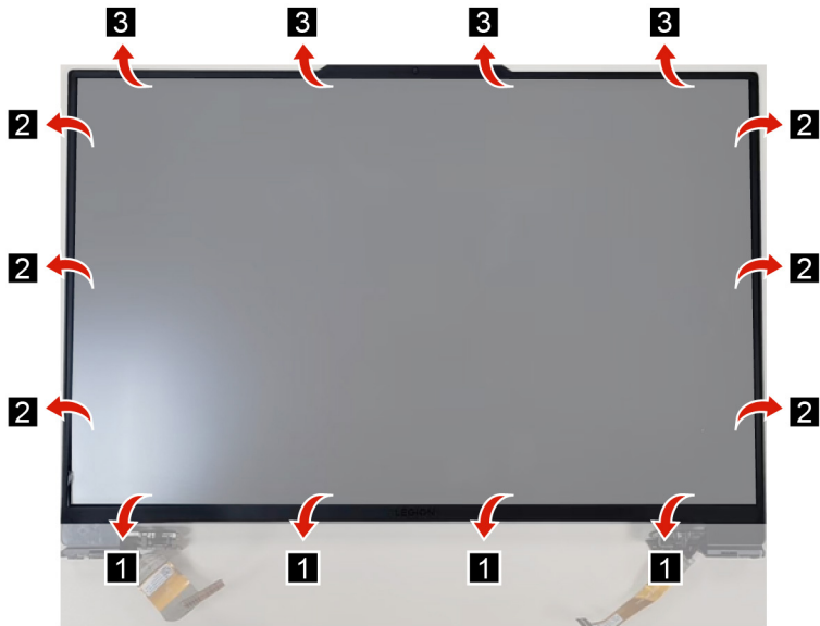
Figure 41. Remove the LCD bezel
