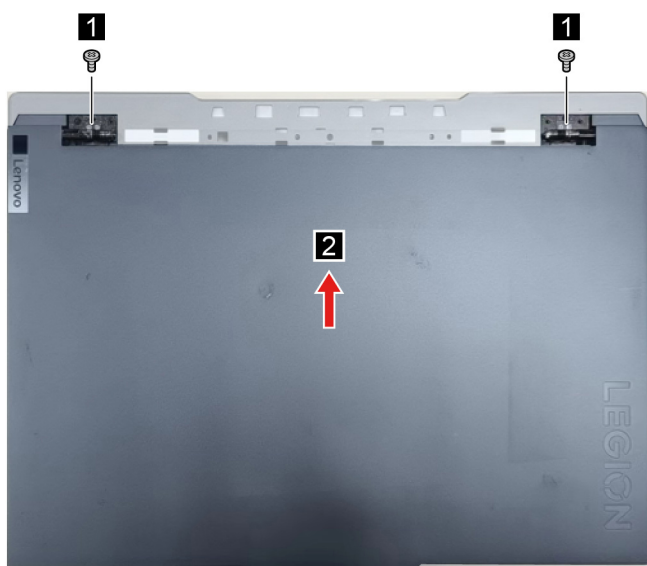
Figure 35. Remove two screws and then remove the LCD module
