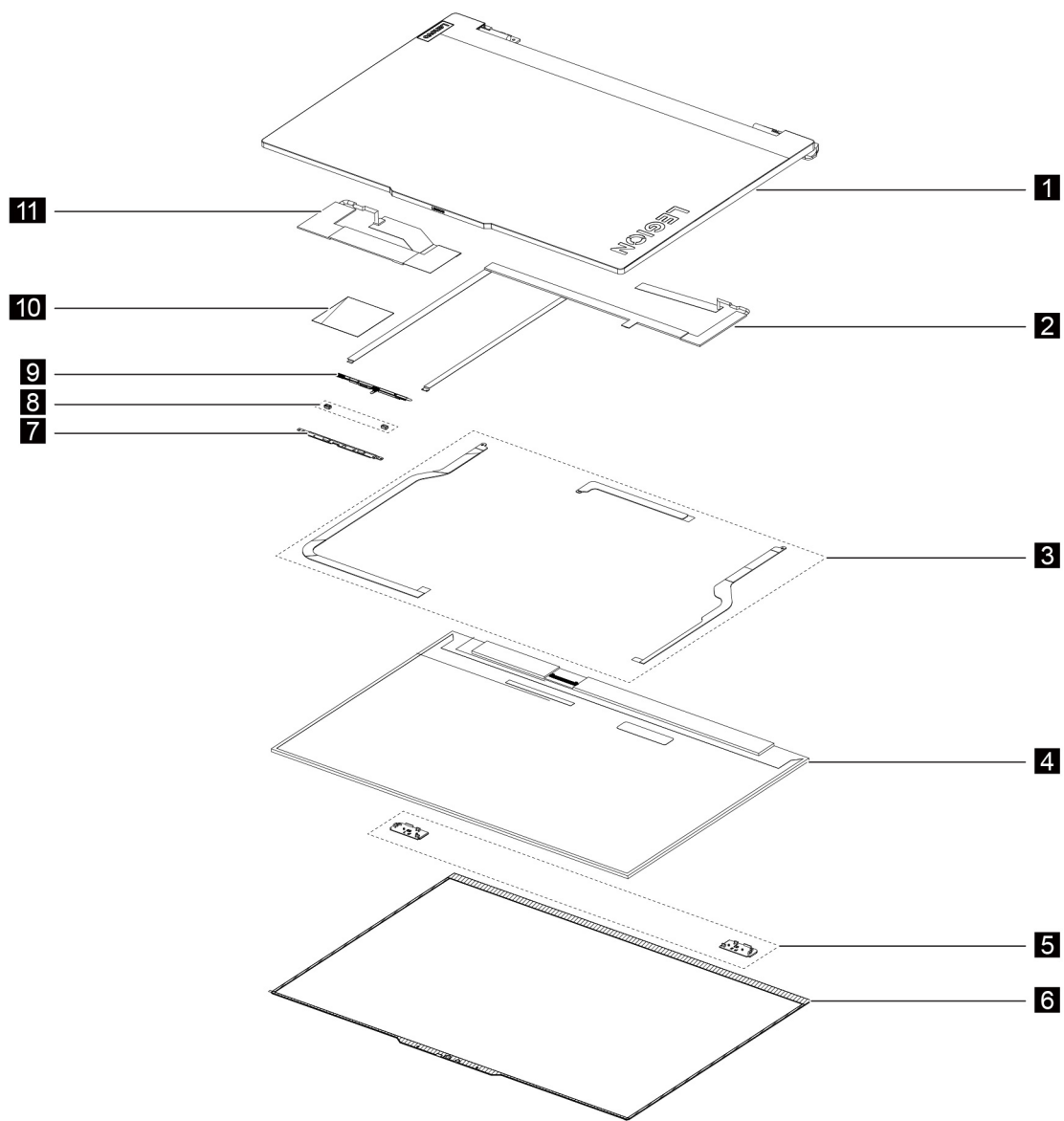
Figure 2. Lenovo Legion 7 (16", 7) LCD module — exploded view
