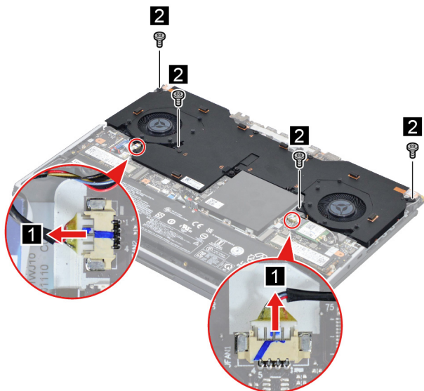
Figure 21. Disconnect the thermal module cable and remove four screws
