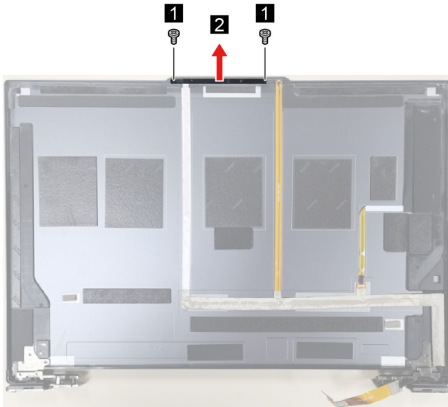
Figure 45. Remove two screws and then remove the camera bracket
