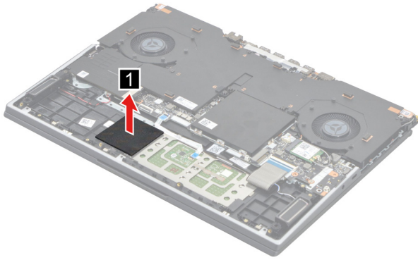
Figure 18. Remove the C cover shield mylar
