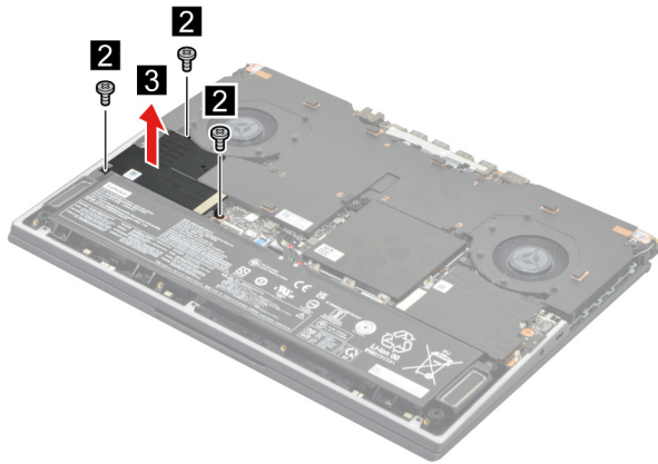
Figure 6. Remove the left SSD plate
