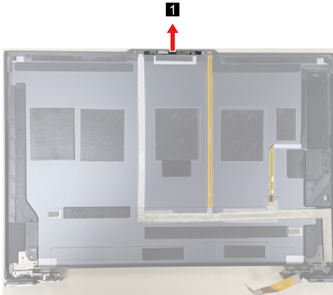
Figure 47. Remove the camera
