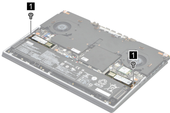
Figure 9. Remove two screws
