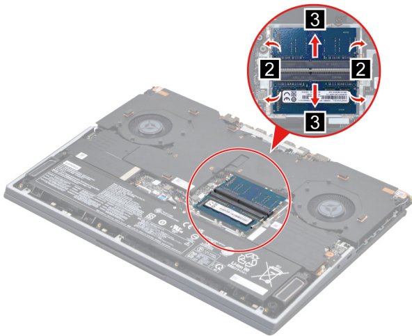
Figure 13. Remove the memory
