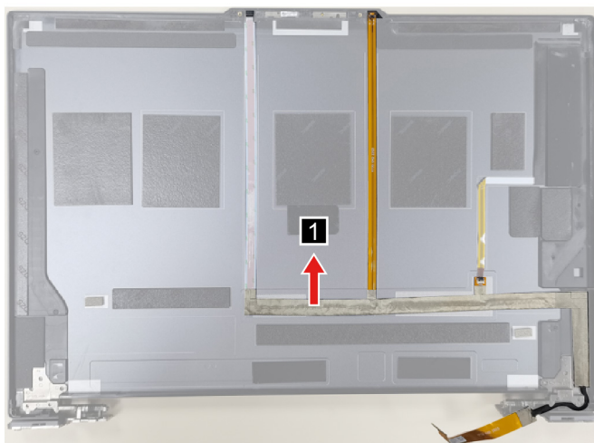
Figure 48. Remove the camera cable
