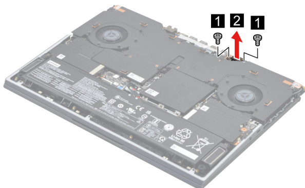
Figure 14. Remove the two screws then remove the DC-in bracket
