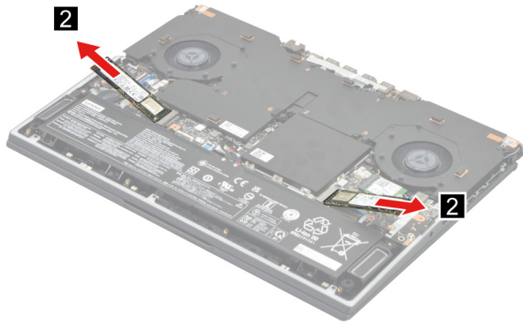
Figure 10. Remove two SSDs
