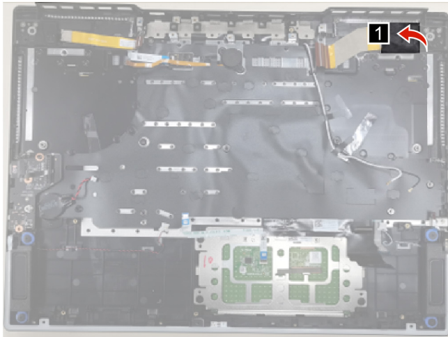
Figure 31. Peel off the tape
