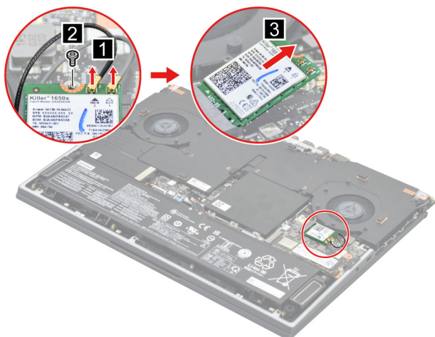
Figure 15. Remove the Wi-Fi card
