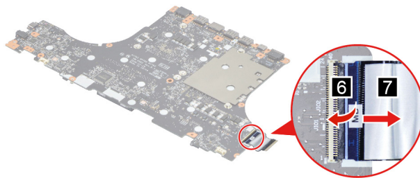
Figure 27. Remove the I/O board cable
