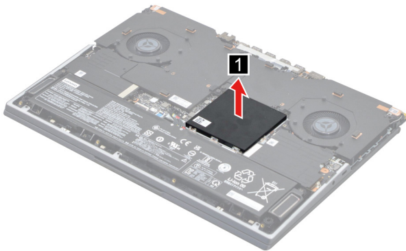
Figure 12. Remove the memory shielding
