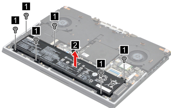
Figure 11. Remove the battery pack
