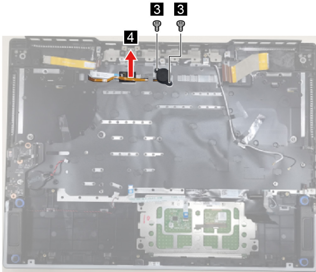
Figure 30. Remove the I/O board cable
