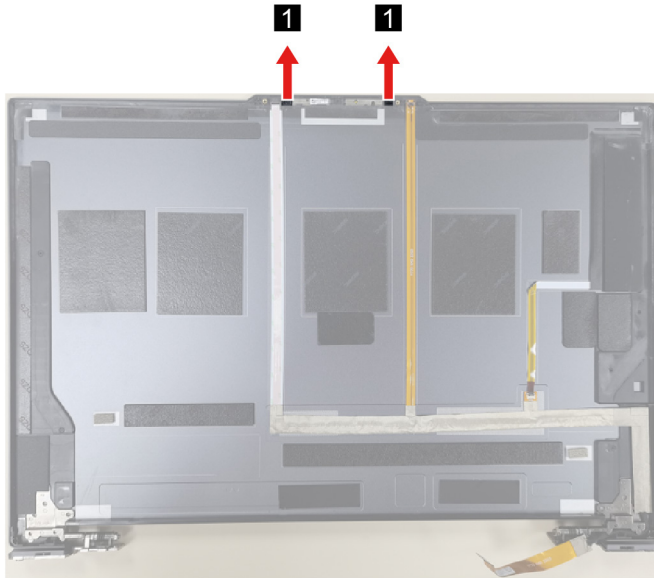
Figure 46. Remove the microphone rubbers
