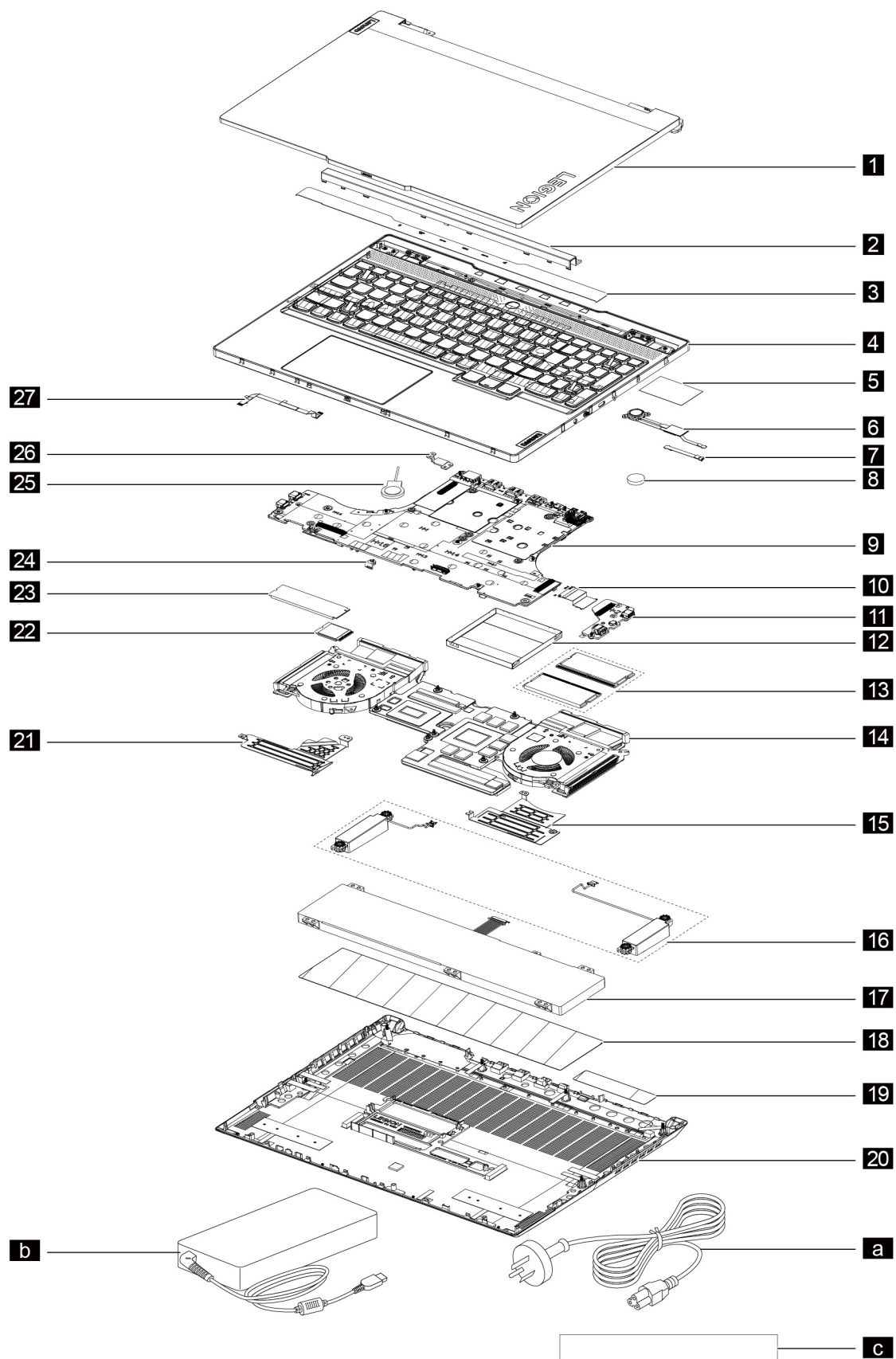
Figure 1. Lenovo Legion 7 (16", 7) exploded view
