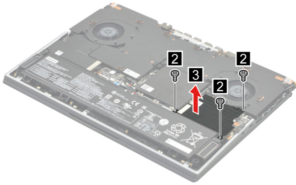
Figure 8. Remove the right SSD plate
