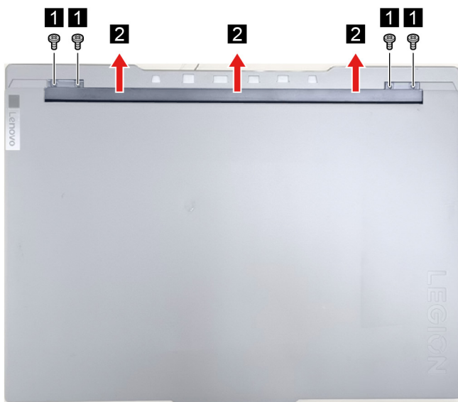
Figure 34. Remove the hinge cap
