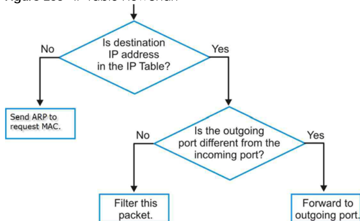
Figure 253 IP Table Flowchart
