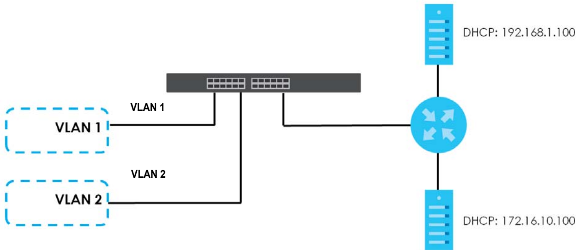
Figure 205 DHCP Relay for Two VLANs
