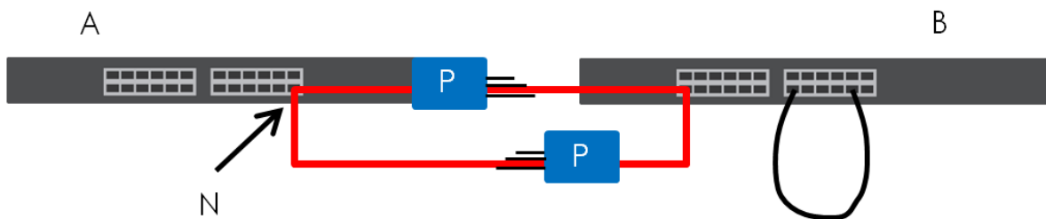
Figure 159 Loop Guard – Probe Packet
