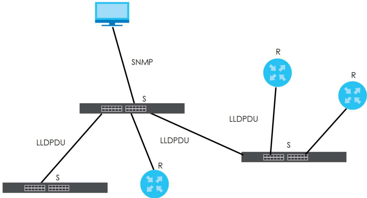
Figure 176 LLDP Overview
