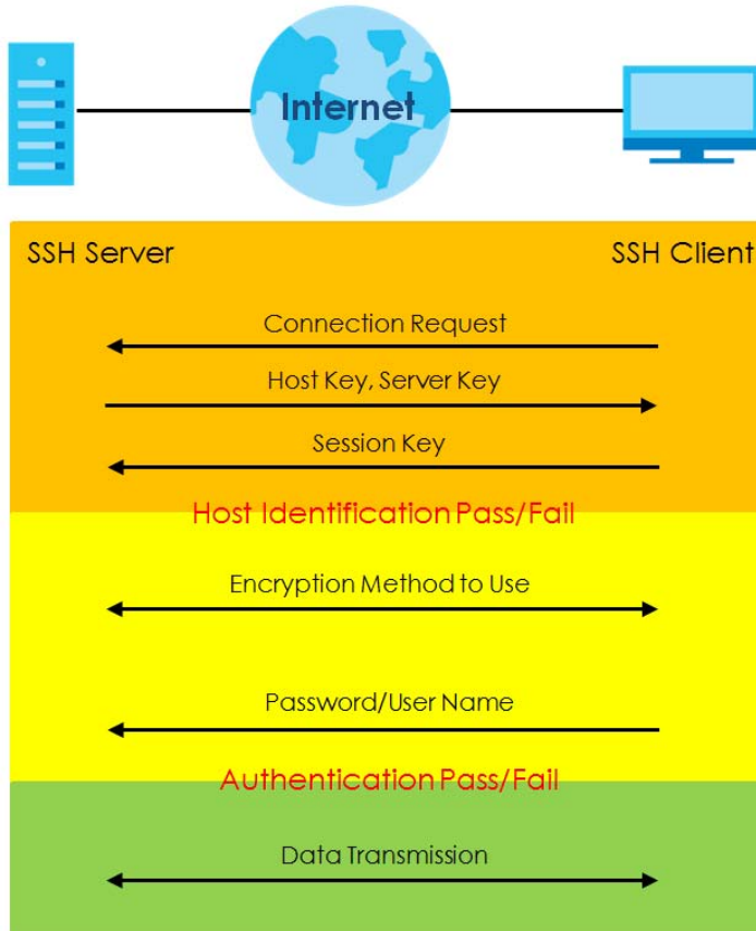
Figure 233 How SSH Works
