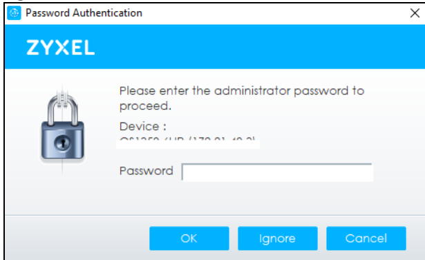
Figure 34 Password Prompt
