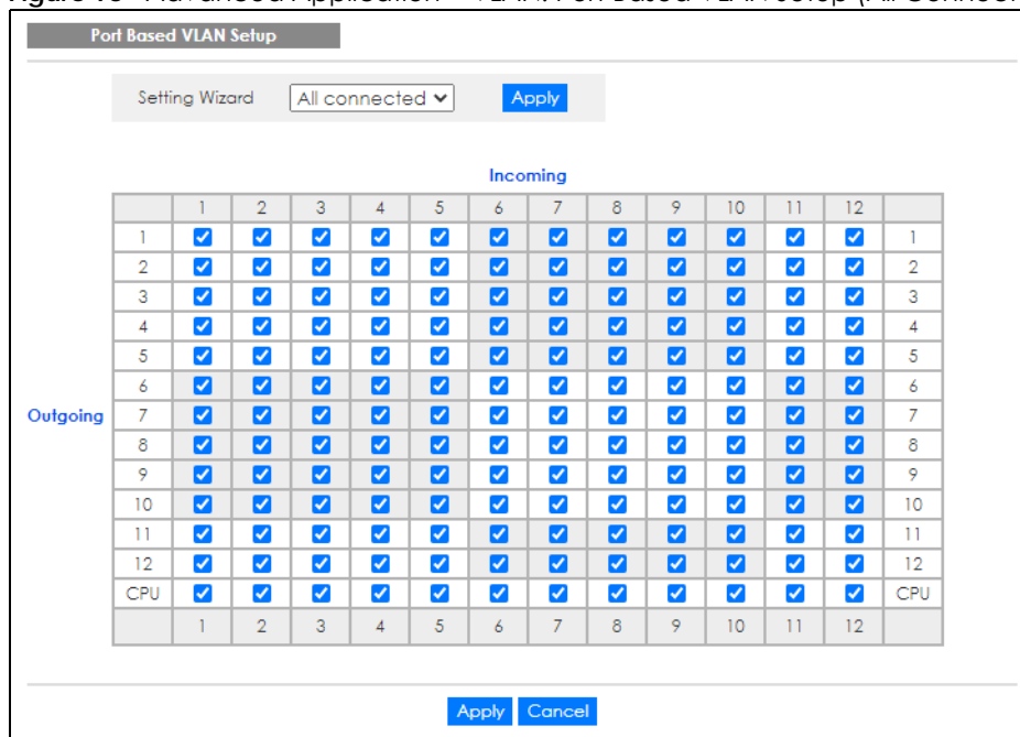
Figure 98 Advanced Application > VLAN: Port Based VLAN Setup (All Connected)
