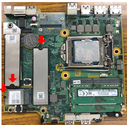
SSD PCB
