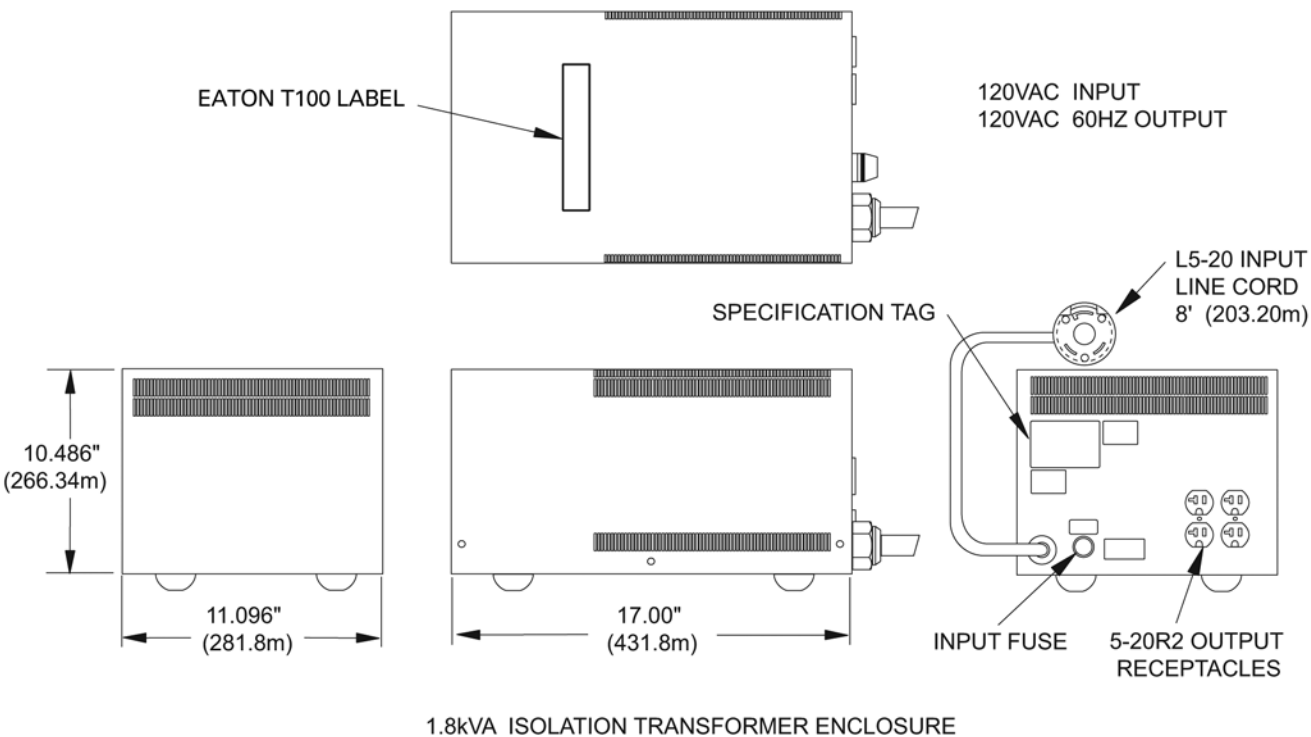
Figure 1-4: 1.8 kVA isolation transformer enclosure, line cord model
