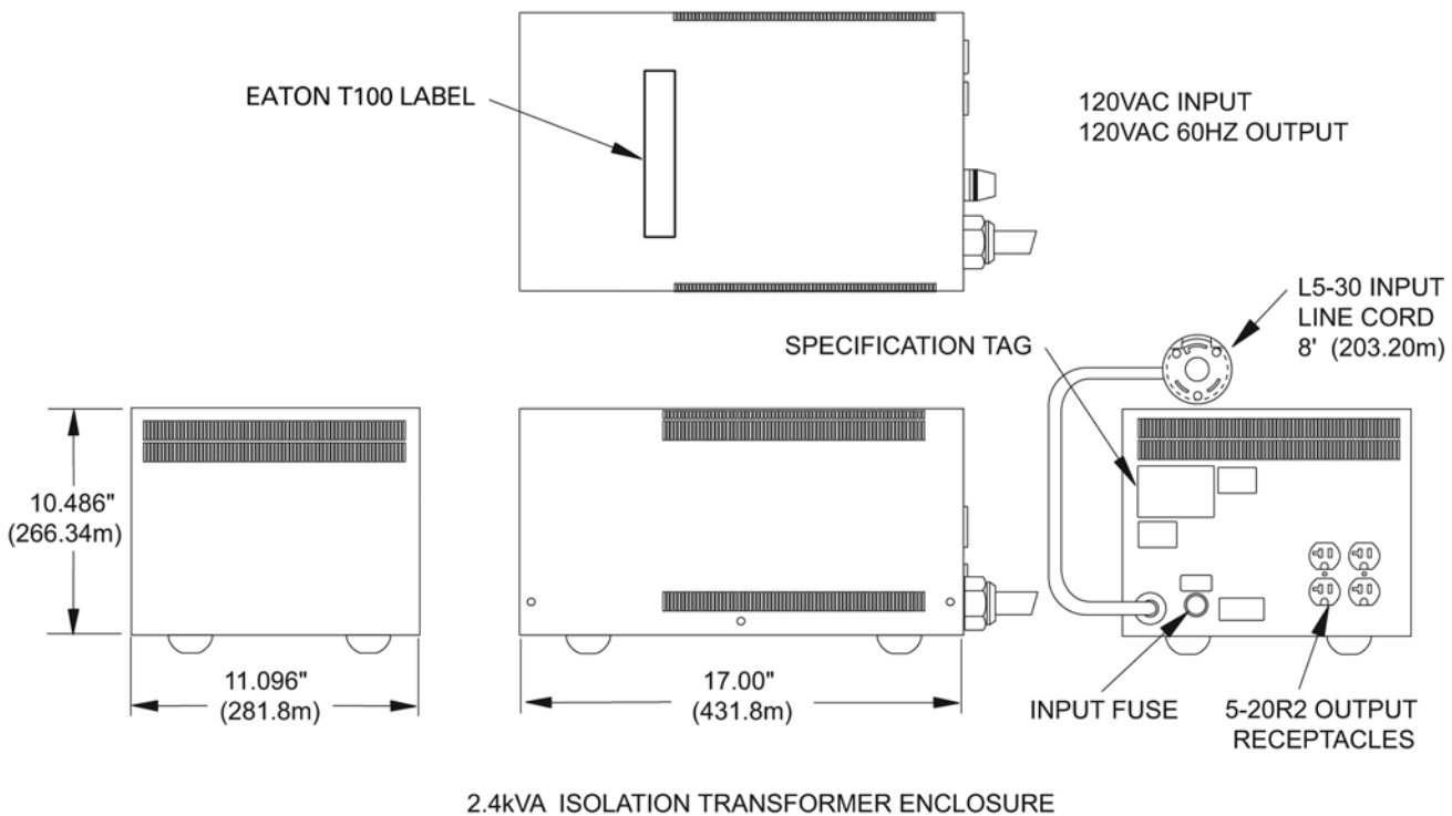
Figure 1-5: 2.4 kVA isolation transformer enclosure, line cord model
