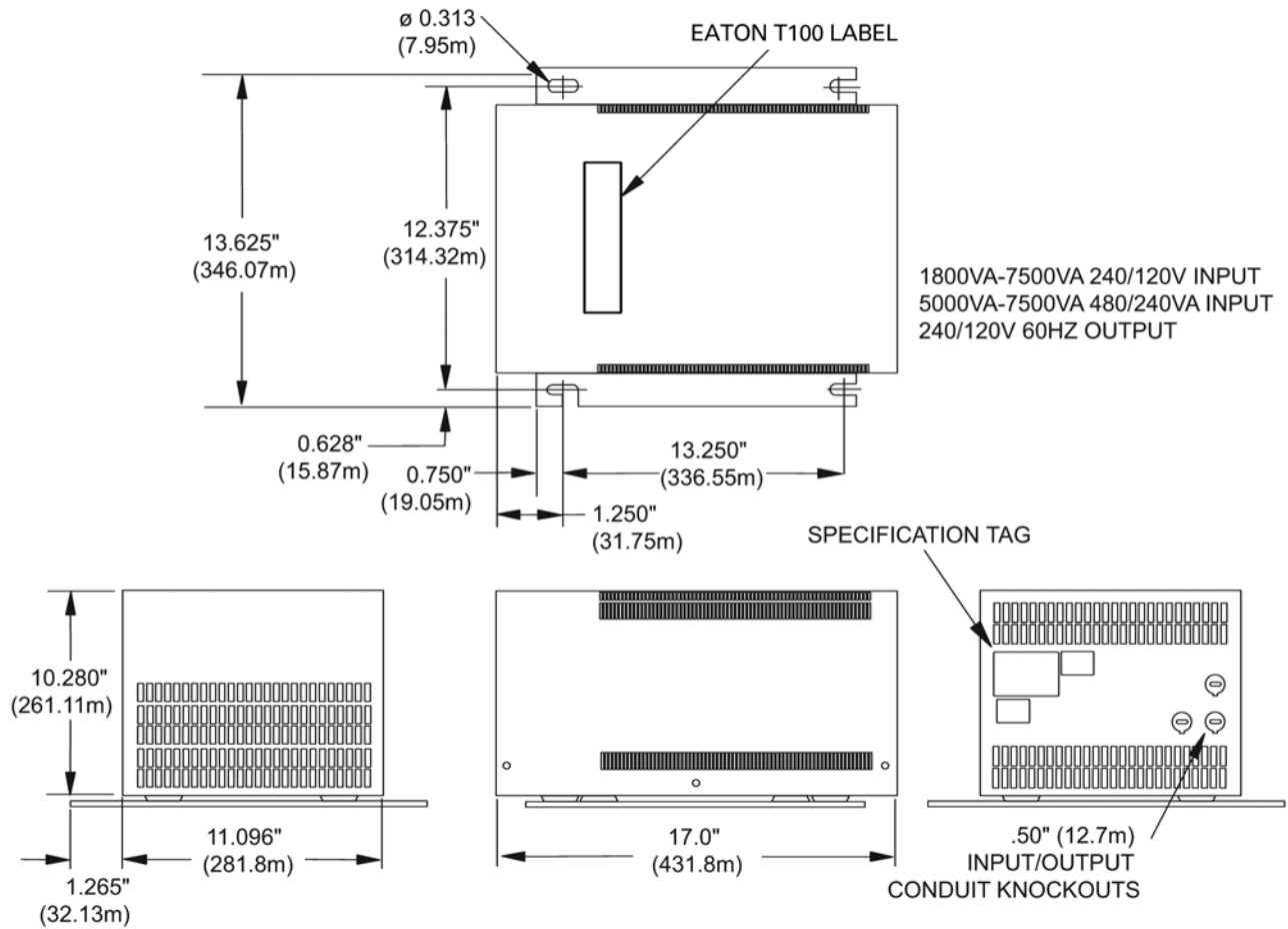
1.8 kVA- 7.5 kVA ISOLATION TRANSFORMER HARDWIRED ENCLOSURE
