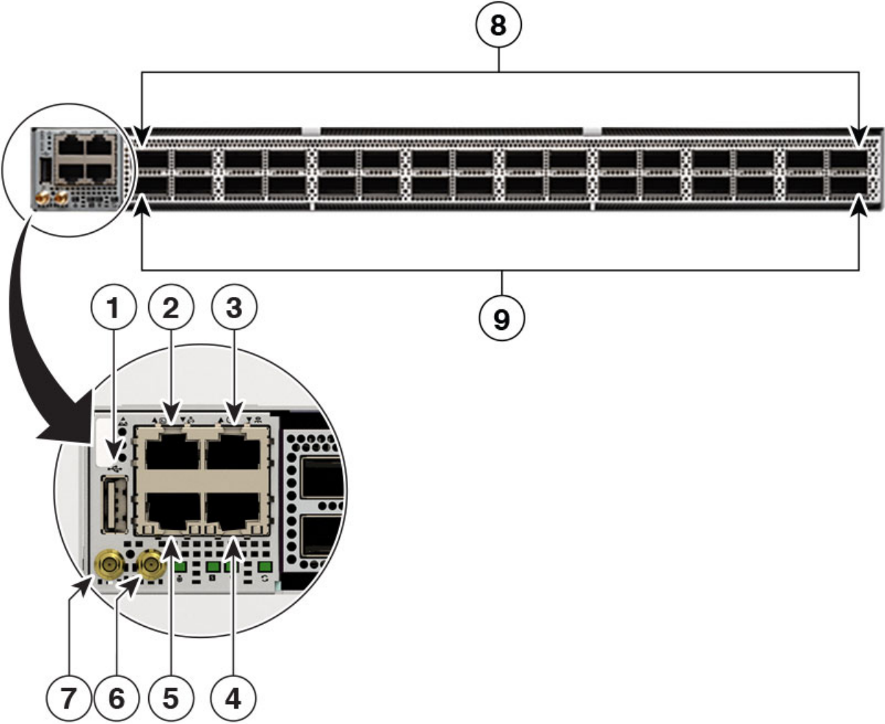
Figure 2: Front panel of HF6100-32D
