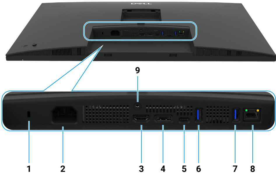
Figure 4. Bottom view of the monitor
