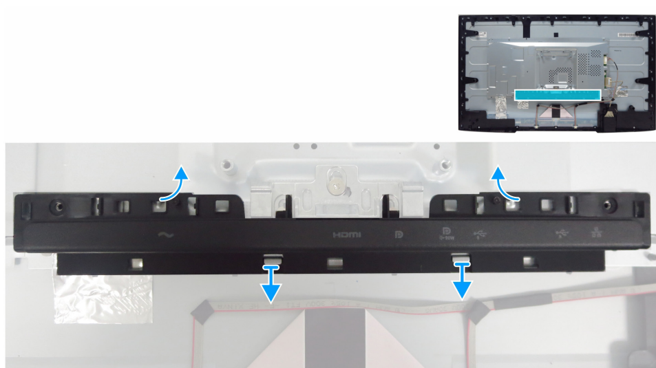
Figure 19. Removing the I/O cover
