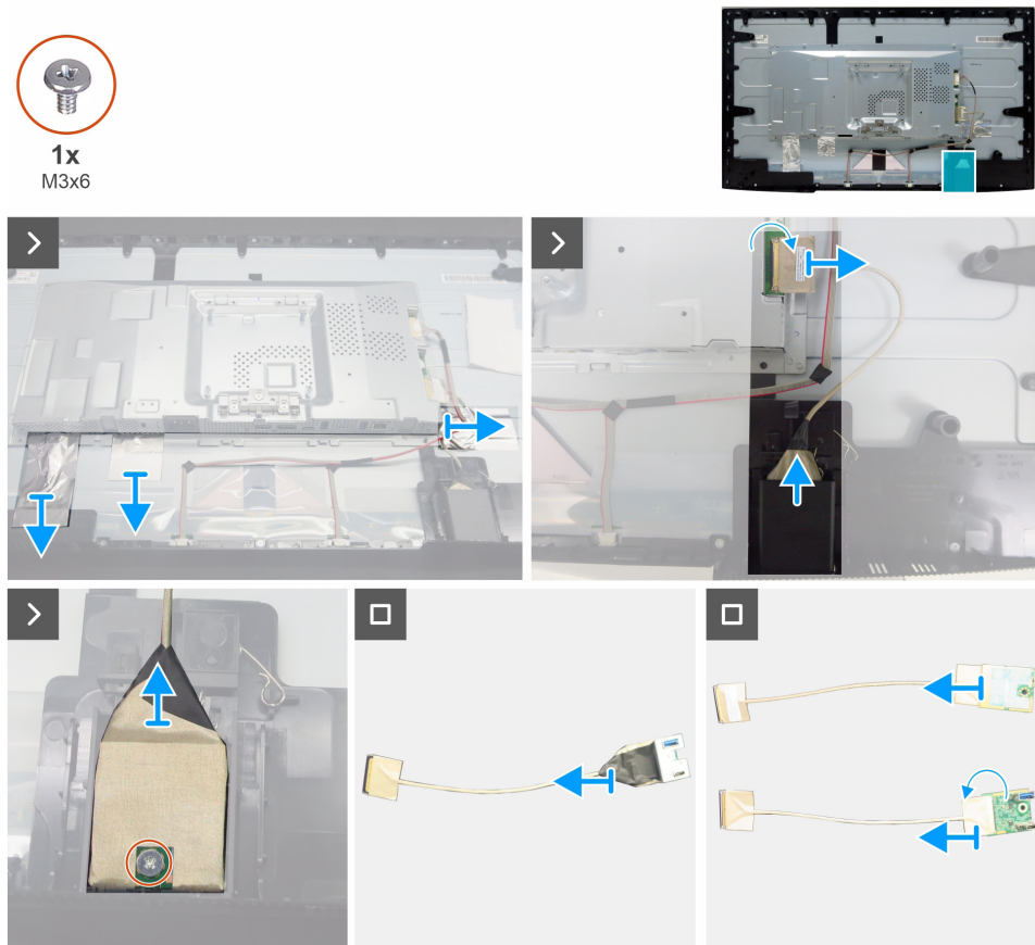
Figure 21. Removing the USB board
