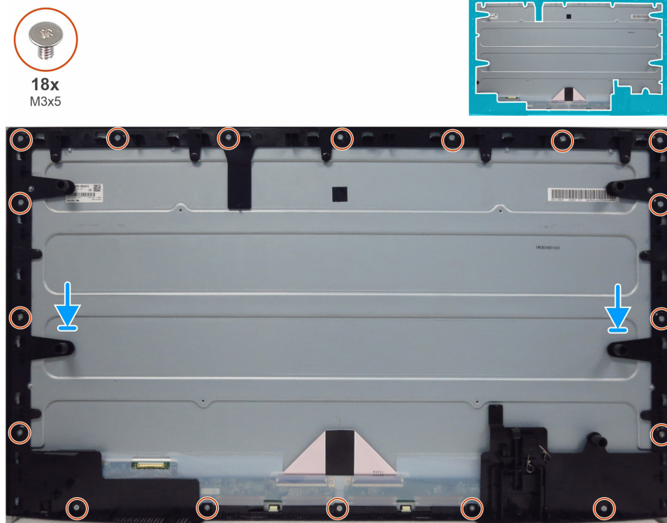
Figure 26. Installing the middle frame
