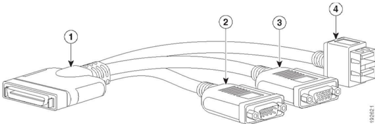
Figure 7 KVM Cable
