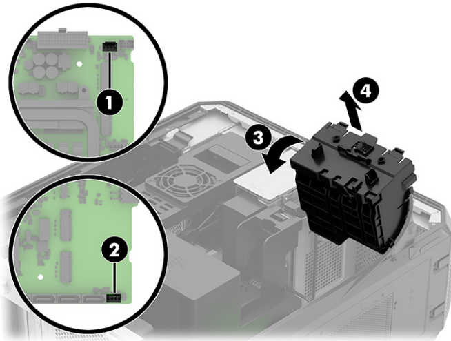
Lower card guide and fan assembly
