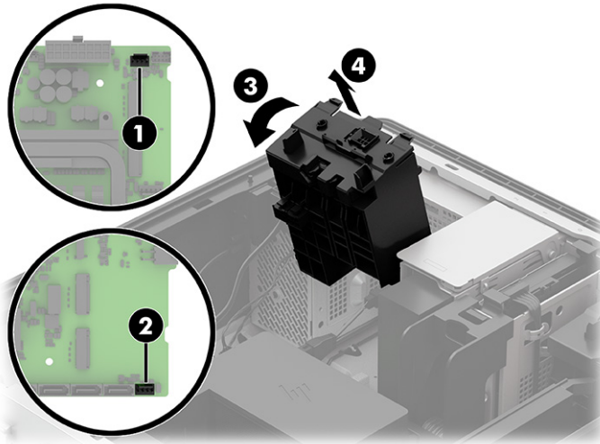
Lower card guide and fan assembly
