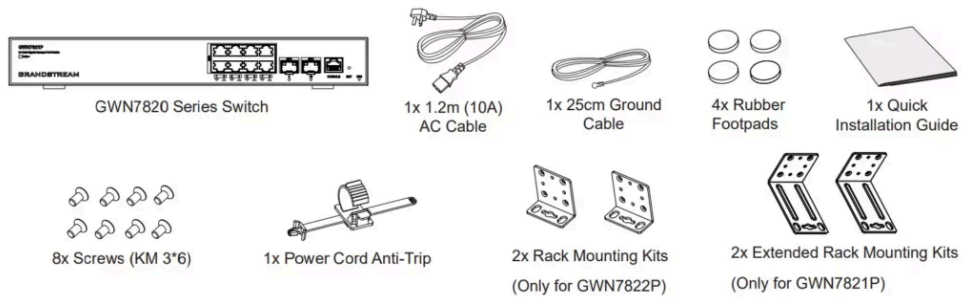
GWN782x Package Content
