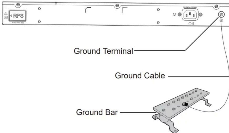
Grounding the Switch
