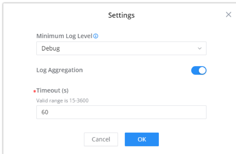
Log Diagnostics
