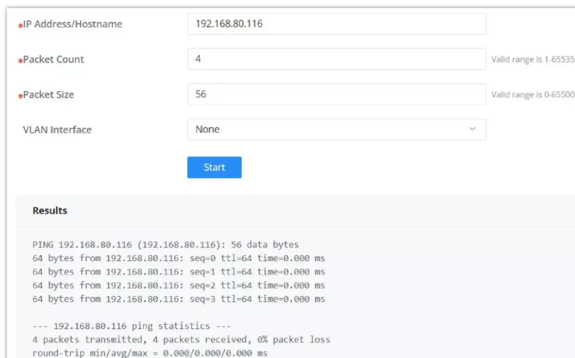
Ping
