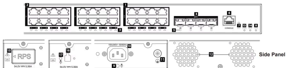
GWN782x Ports
