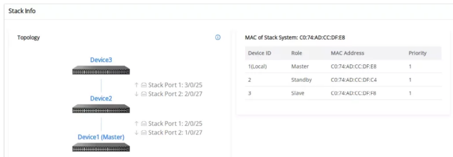
Stack Info
