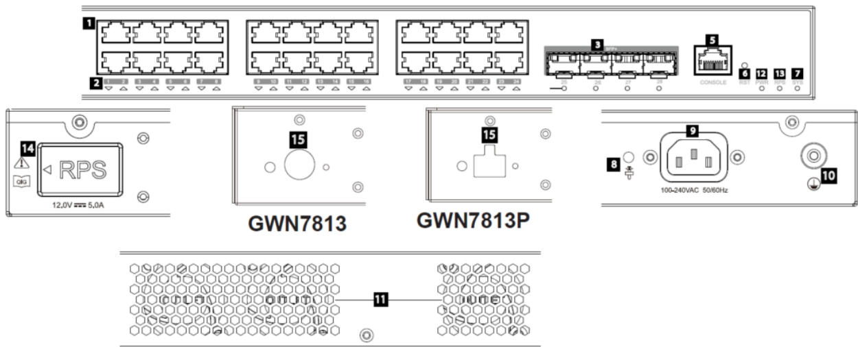
GWN7813GWN7813P Ports
