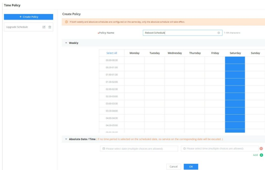
Time Policy
