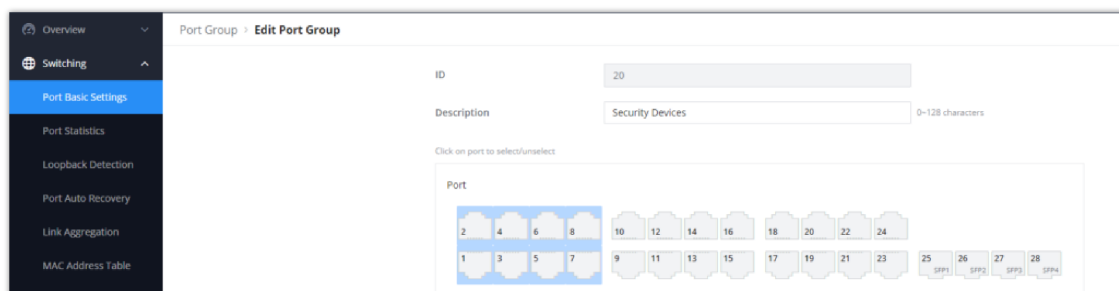
Port Group
