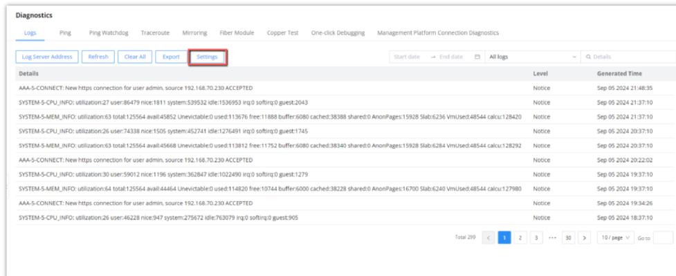
Log Diagnostics
