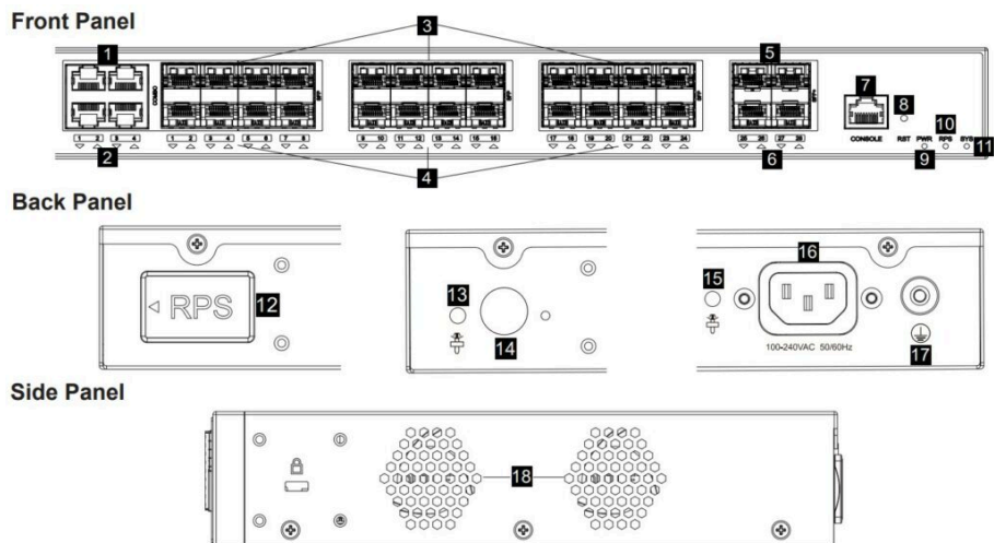
GWN7831 Ports
