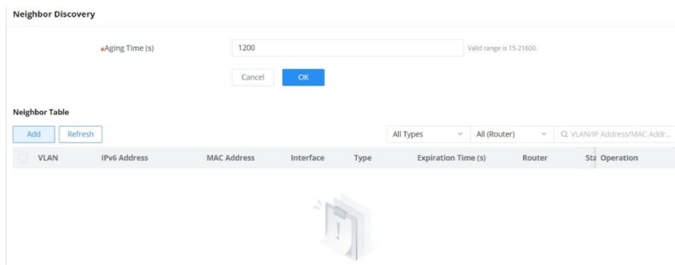
Neighbor Discovery
