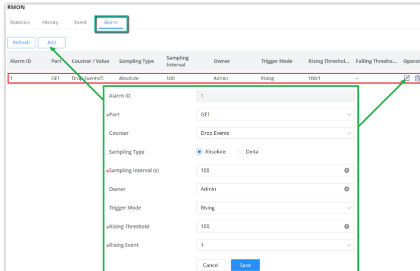
RMON Alarm
