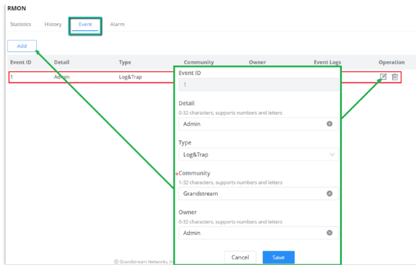
RMON Event
