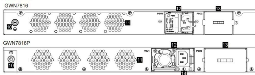
GWN7816GWN7816P Ports
