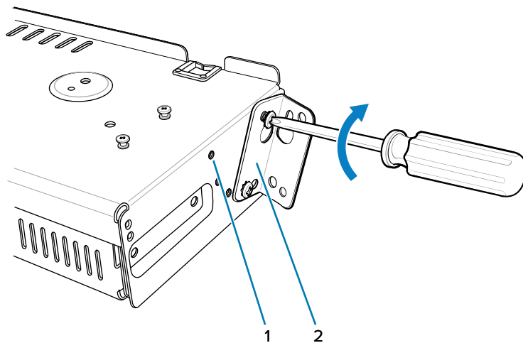
Figure 34 Flange 25° Position (4-Slot Battery Chargers)
