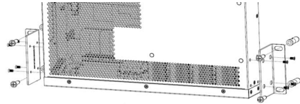
Figure 4 Wall Mount
