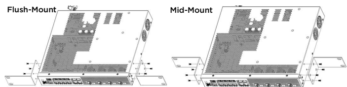
Figure 1 4220 Series: Attach Brackets
