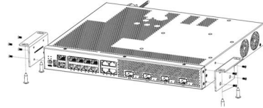
Figure 3 Under Table Mount
