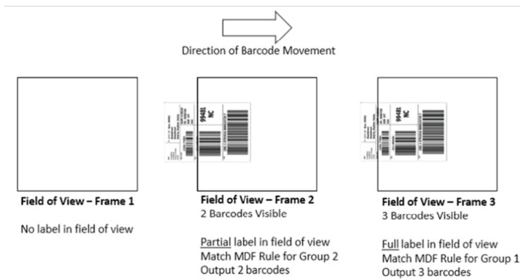
Figure 1 Scanning Label in a Horizontal Orientation
