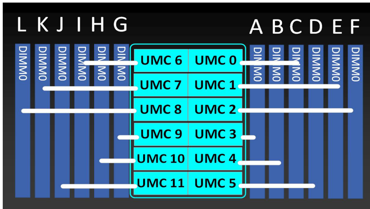
Figure 4 12-Channel Memory Organization
