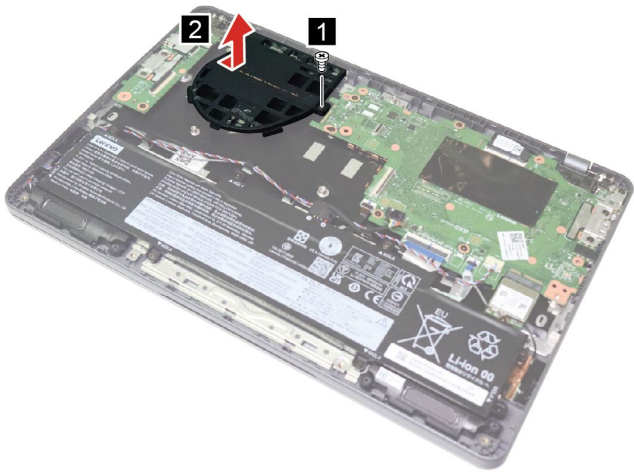
Figure 21. Remove one screw and the dummy fan
