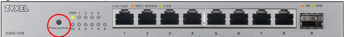
Figure 21 Flow Control Button (XMG-108)
