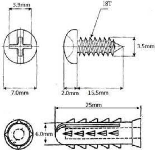
Figure 4 Screw Specifications for Wall Mounting
