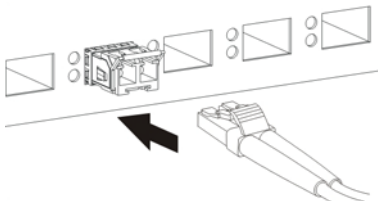
Figure 11 Connecting the Fiber Cables
