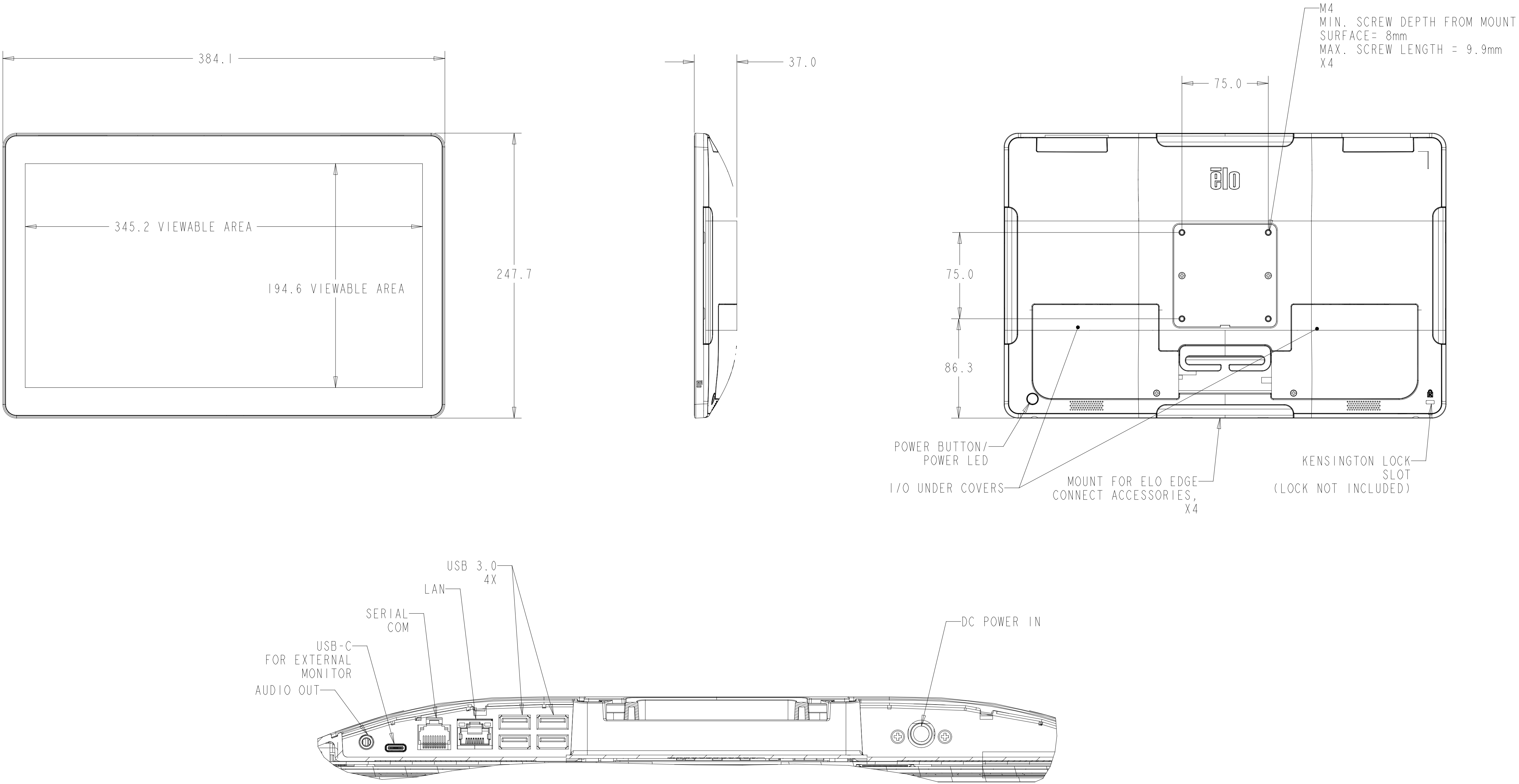
I/O FOR ALL MODELS WITHOUT STAND
