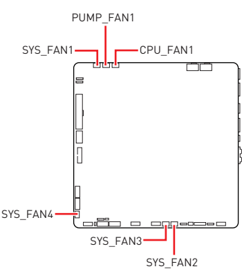
Fan connector specifications
