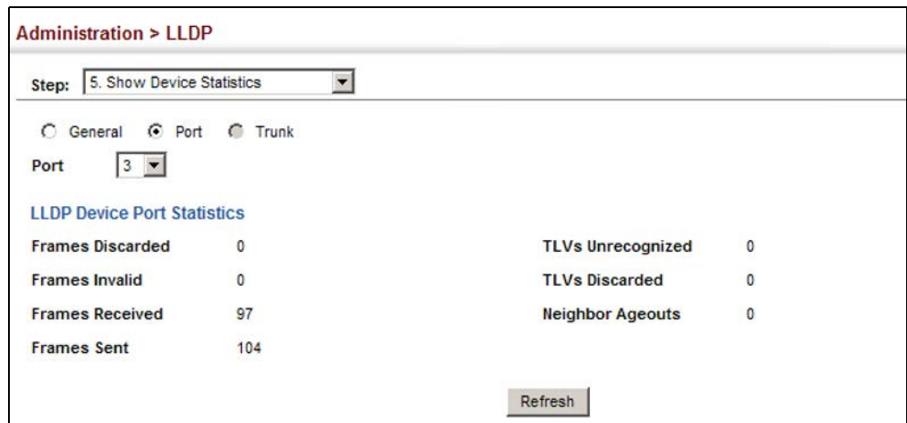
Figure 270: Displaying LLDP Device Statistics (Port)
