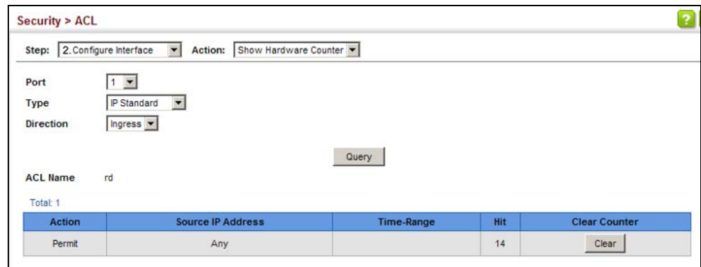
Figure 215: Showing ACL Statistics
