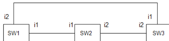
Figure 126: Determining the Root Port
