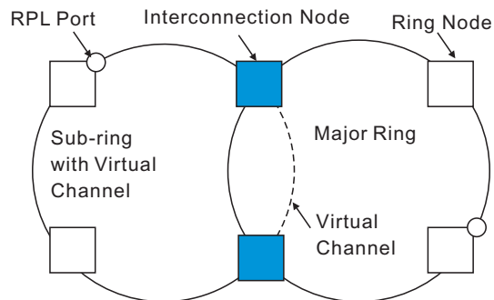
Figure 321: Sub-ring with Virtual Channel
