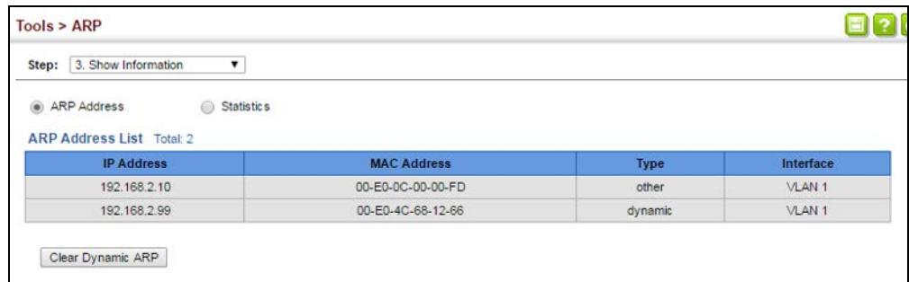
Figure 410: Displaying ARP Entries
