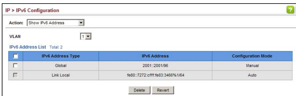
Figure 421: Showing Configured IPv6 Addresses
