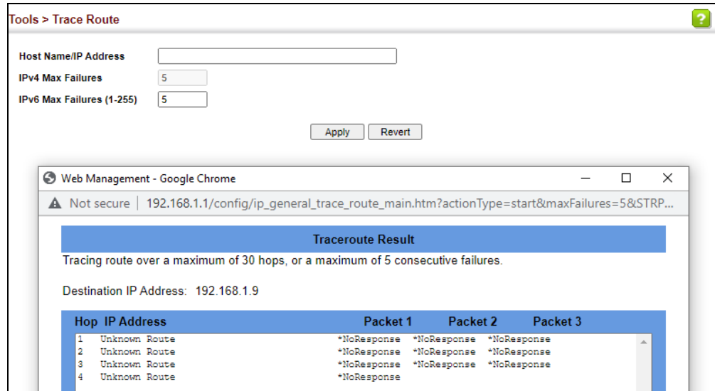
Figure 405: Tracing the Route to a Network Device
