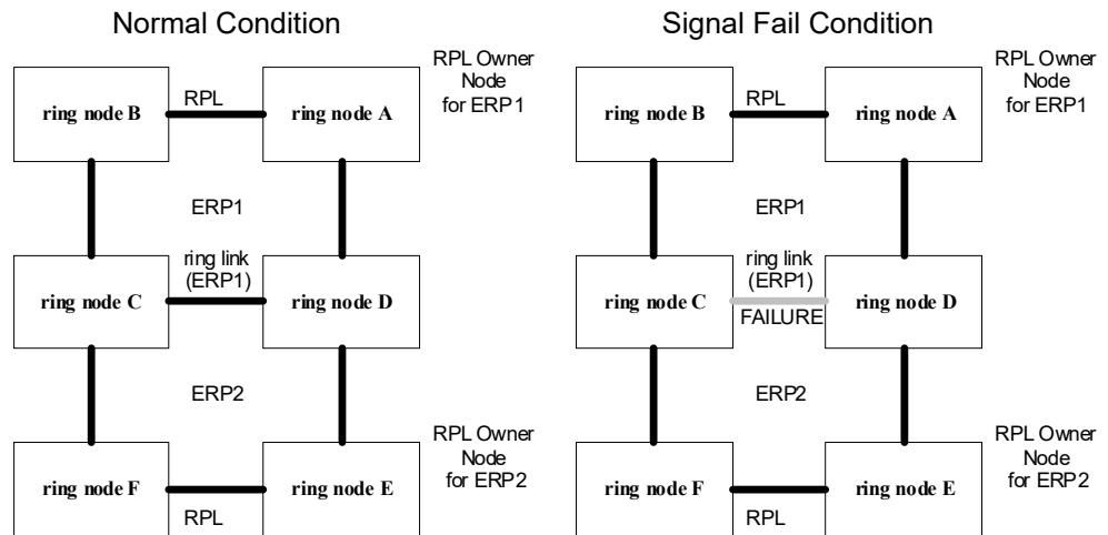
Figure 317: Ring Interconnection Architecture (Multi-ring/Ladder Network)
