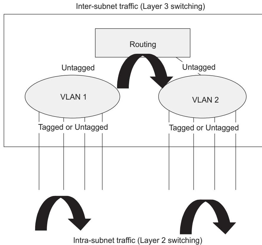
Figure 427: Virtual Interfaces and Layer 3 Routing
