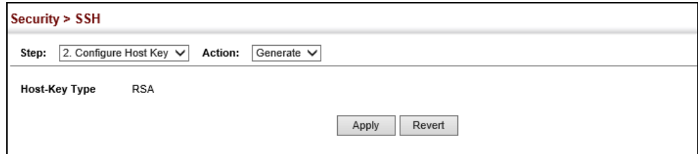
Figure 201: Generating the SSH Host Key Pair
