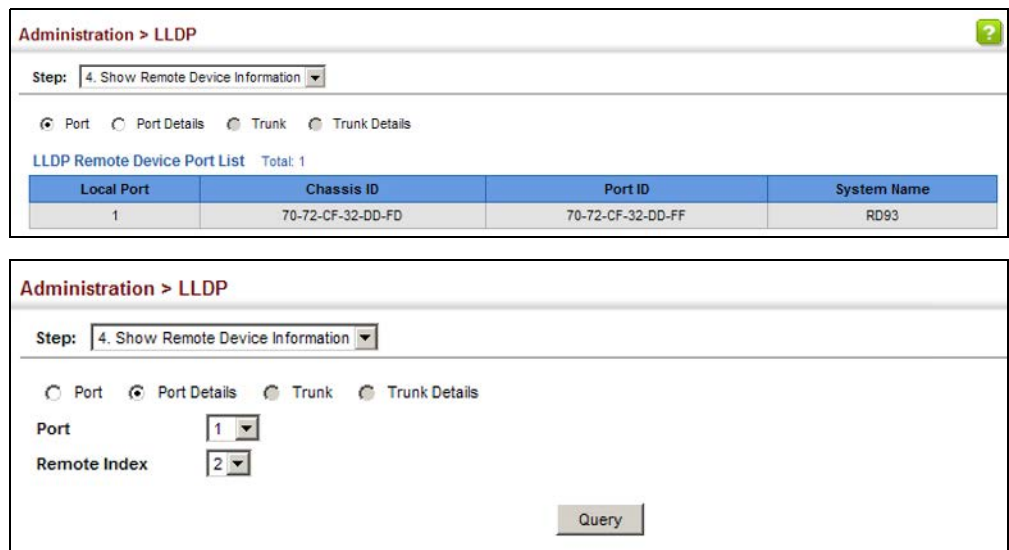
Figure 266: Displaying Remote Device Information for LLDP (Port)
