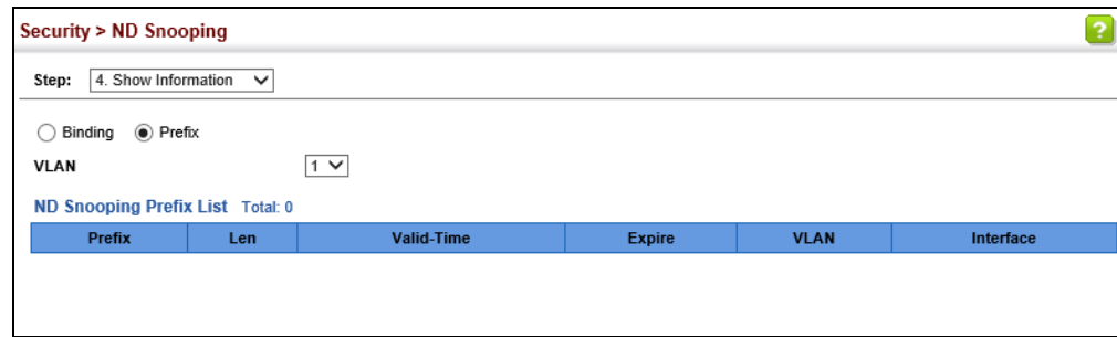
Figure 240: Displaying the Prefix List for ND Snooping
