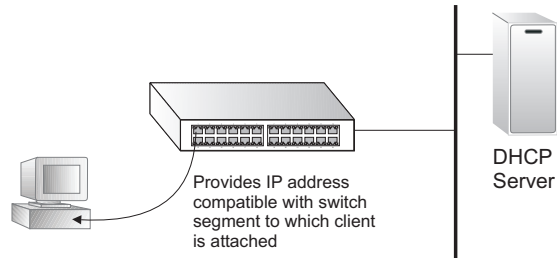
Figure 441: Layer 3 DHCP Relay Service
