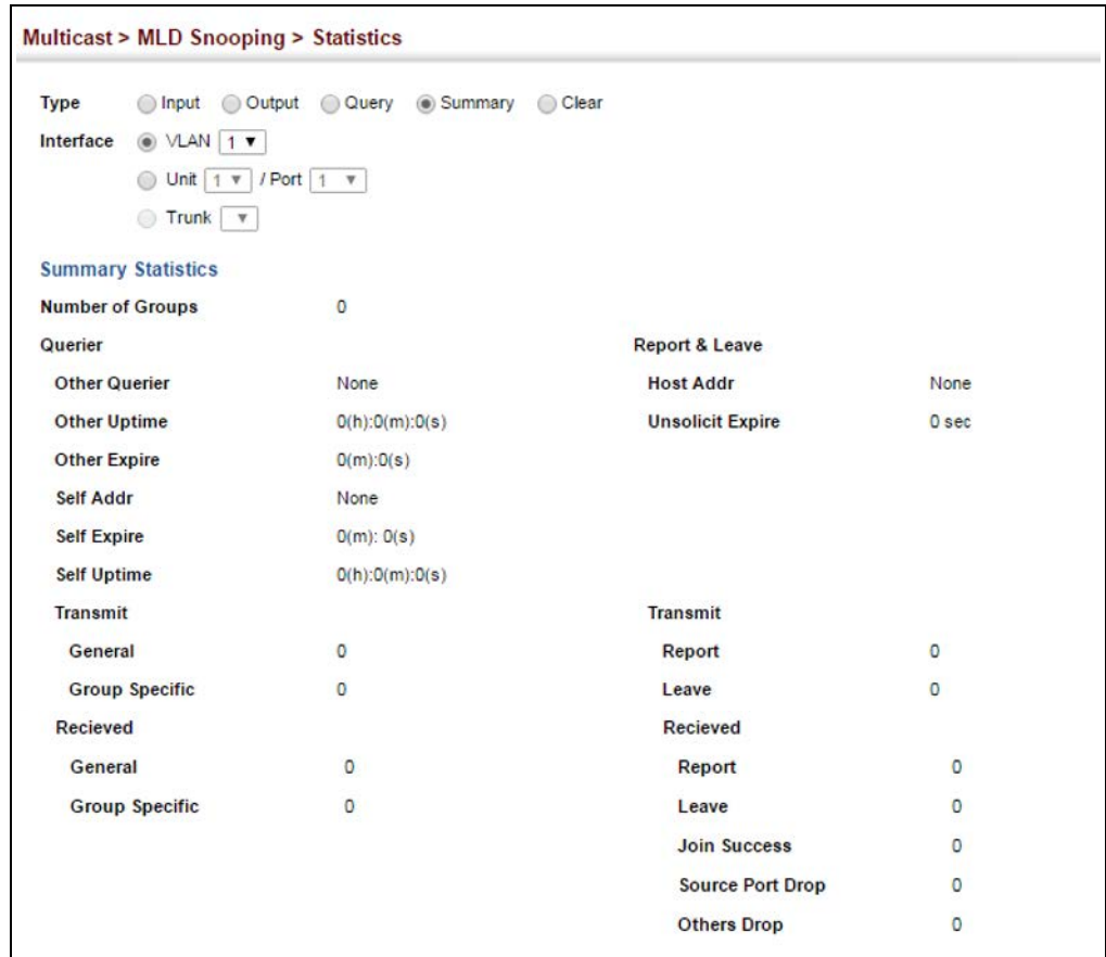
Figure 382: Displaying MLD Snooping Statistics – Summary (VLAN)
