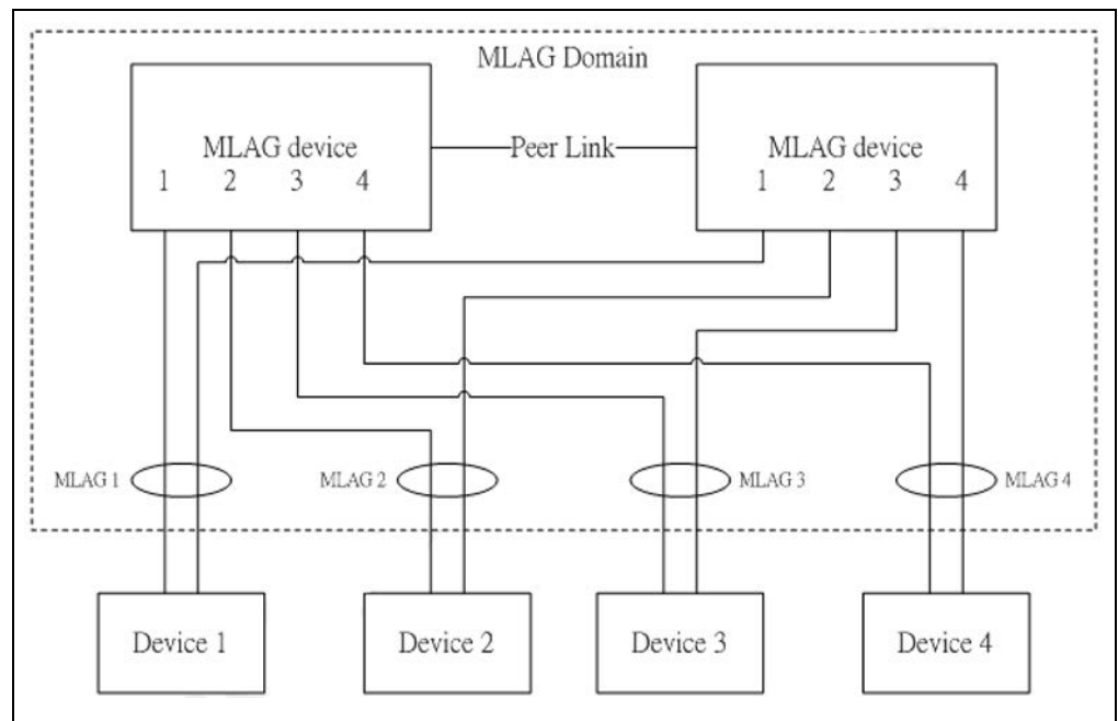
Figure 327: MLAG Domain Topology
