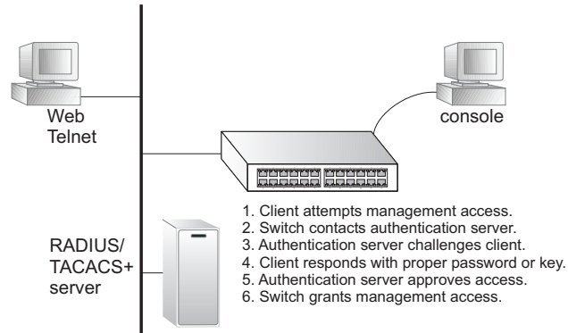
Figure 171: Authentication Server Operation
