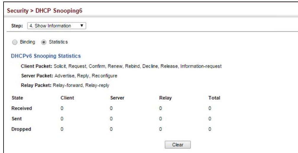
Figure 235: Displaying Statistics for DHCPv6 Snooping
