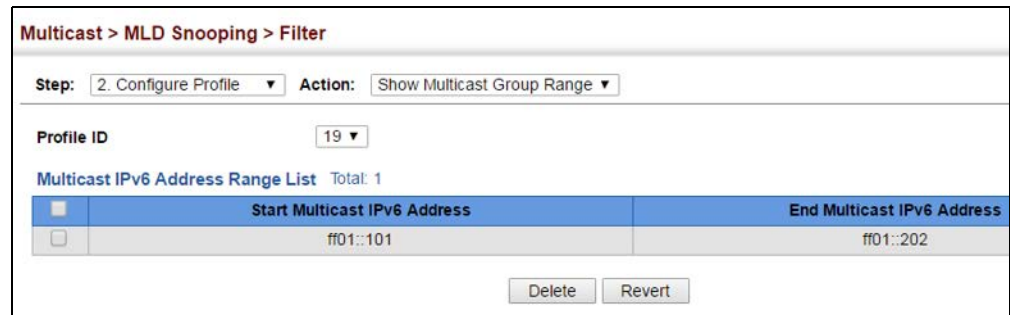
Figure 388: Showing the Groups Assigned to an MLD Filtering Profile
