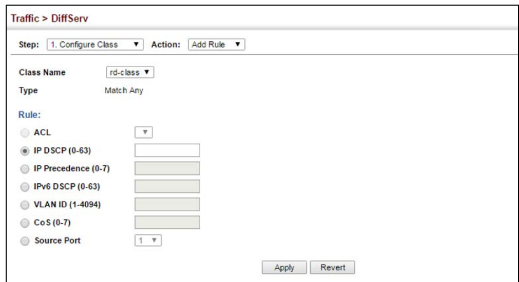
Figure 159: Adding Rules to a Class Map
