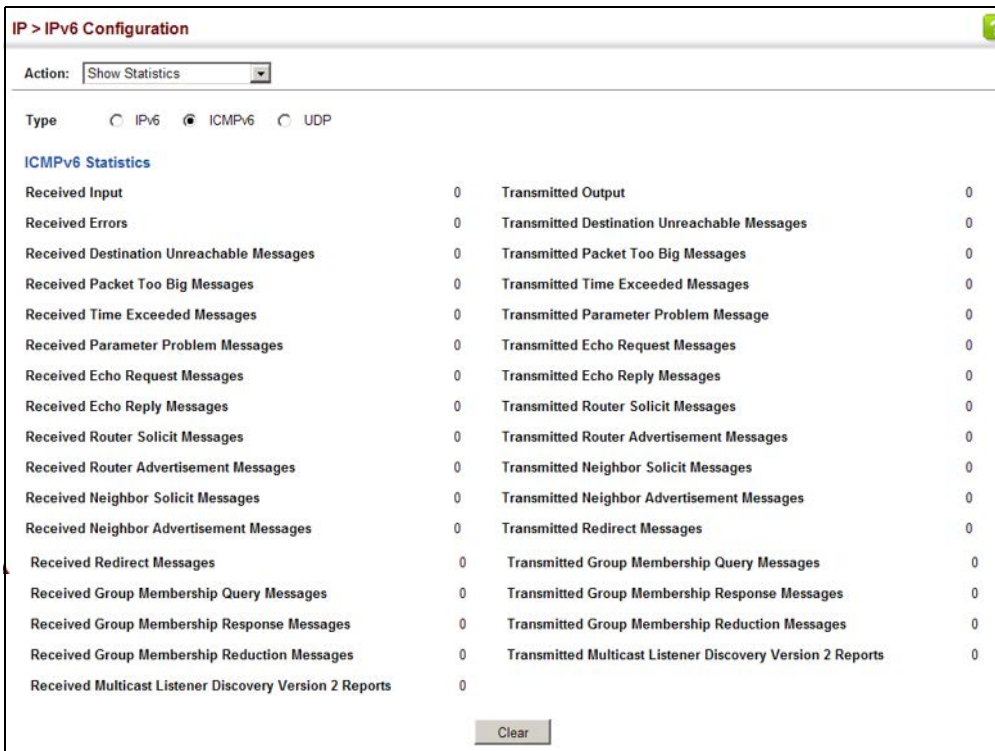
Figure 424: Showing IPv6 Statistics (ICMPv6)
