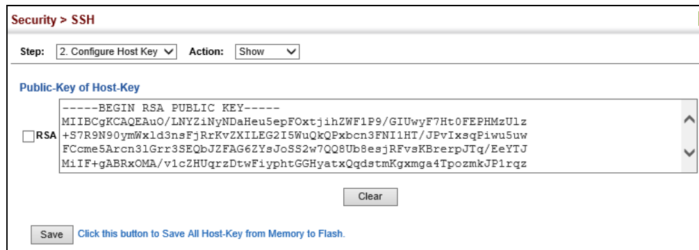
Figure 202: Showing the SSH Host Key Pair
