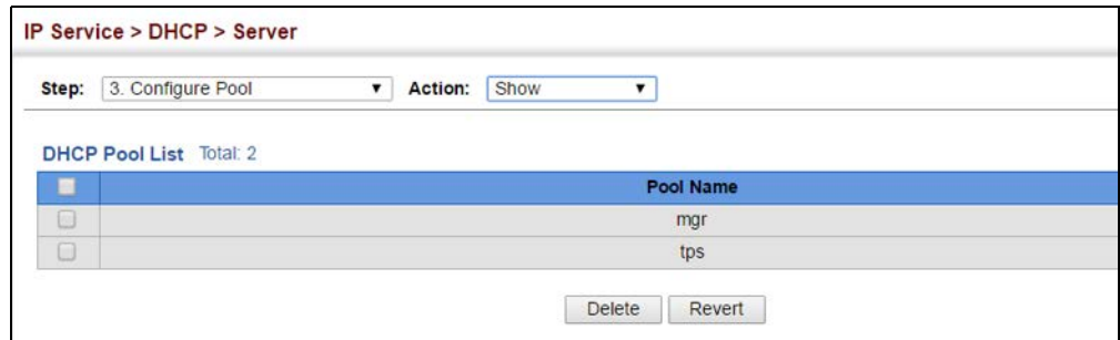
Figure 451: Showing Configured DHCP Server Address Pools
