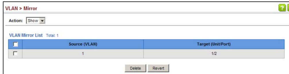
Figure 104: Showing the VLANs to Mirror
