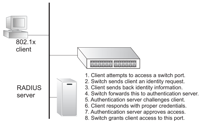
Figure 219: Configuring Port Authentication
