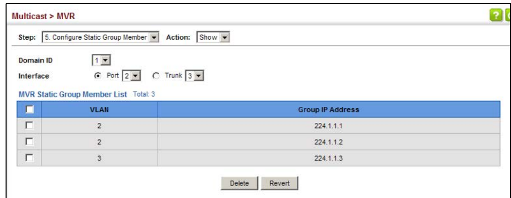
Figure 399: Showing the Static MVR Groups Assigned to a Port
