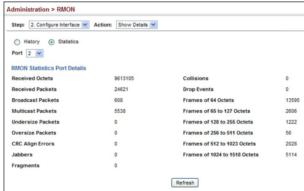
Figure 306: Showing Collected RMON Statistical Samples
