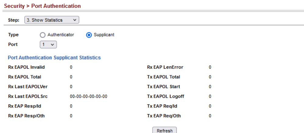
Figure 224: Showing Statistics for 802.1X Port Supplicant
