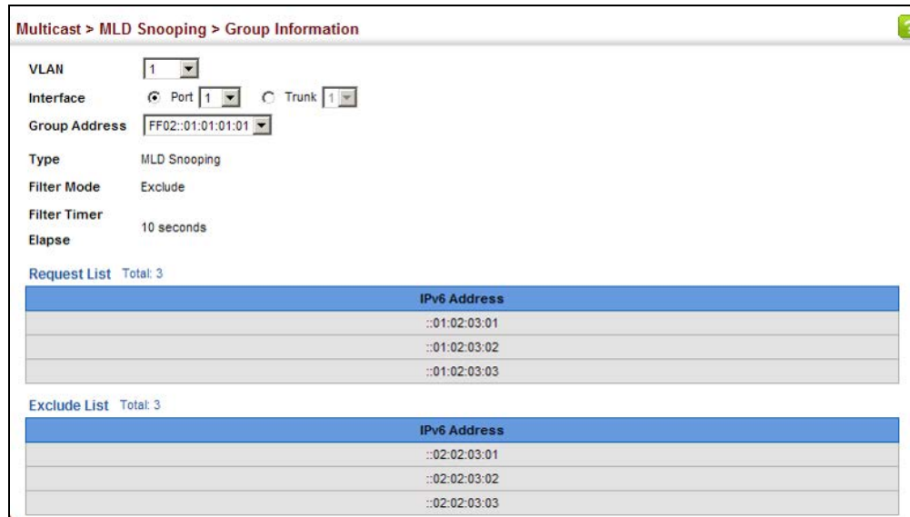
Figure 377: Showing IPv6 Multicast Services and Corresponding Sources
