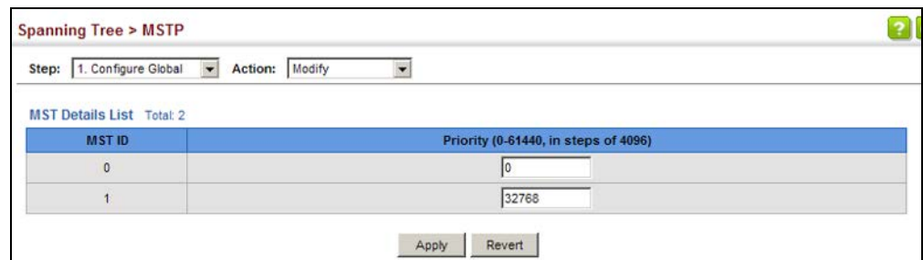
Figure 132: Modifying the Priority for an MST Instance
