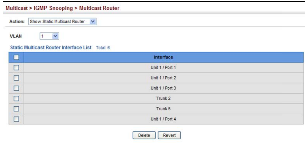
Figure 350: Showing Static Interfaces Attached a Multicast Router
