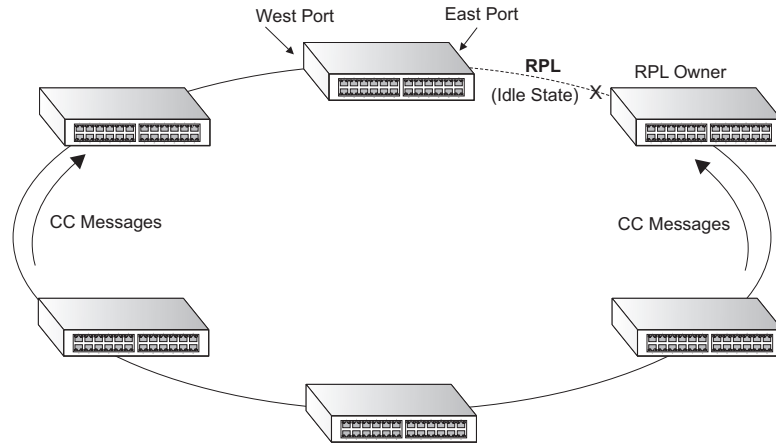
Figure 316: ERPS Ring Components
