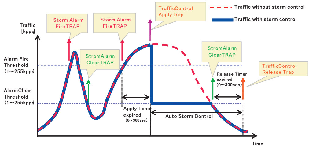
Figure 140: Storm Control by Limiting the Traffic Rate
