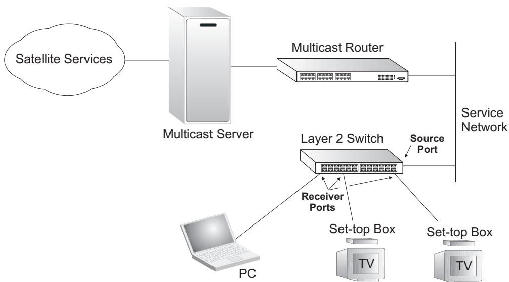
Figure 390: MVR Concept
