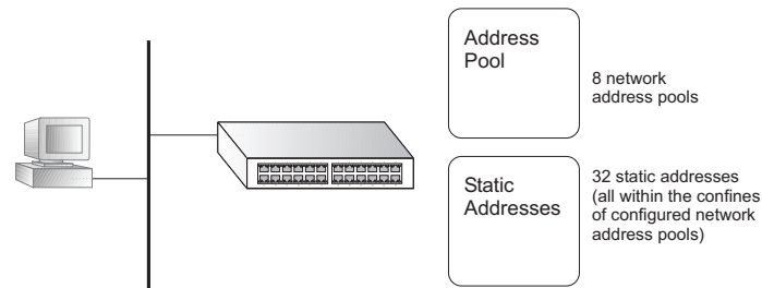
Figure 445: DHCP Server
