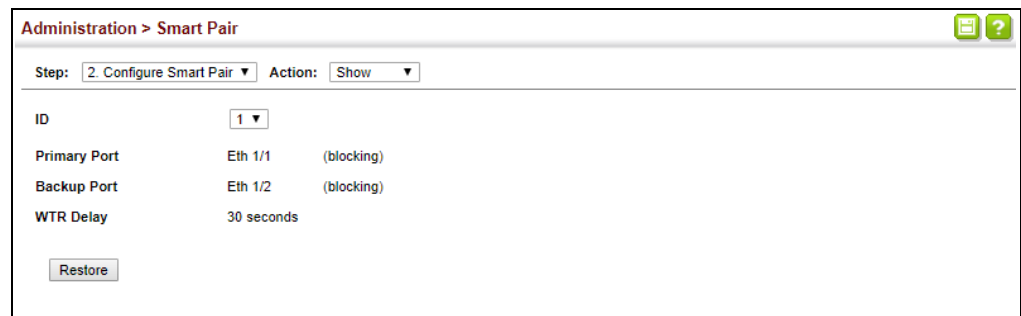
Figure 346: Displaying Port Members of a Smart Pair
