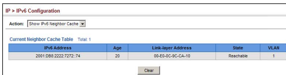
Figure 422: Showing IPv6 Neighbors
