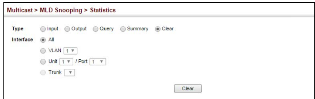
Figure 383: Clearing MLD Snooping Statistics
