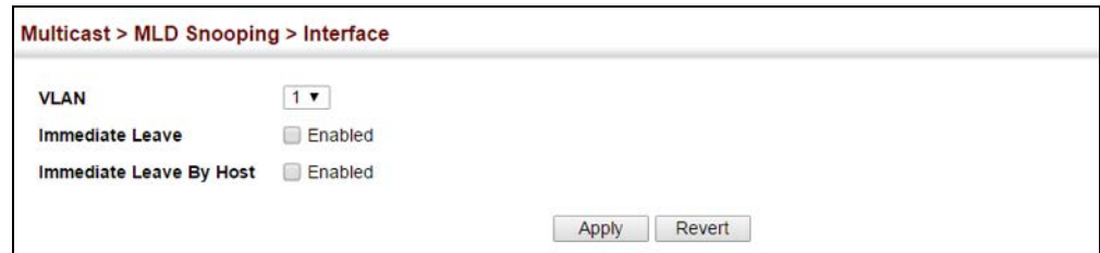
Figure 369: Configuring Immediate Leave for MLD Snooping
