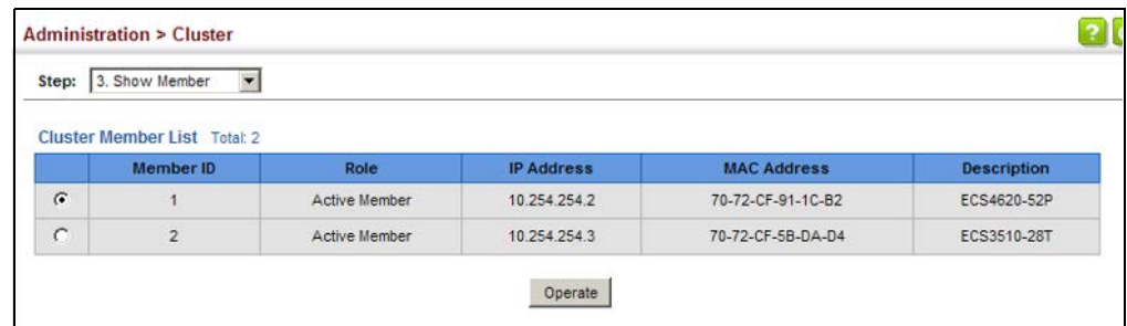
Figure 311: Managing a Cluster Member
