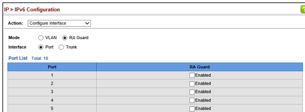
Figure 417: Configuring RA Guard for an IPv6 Interface
