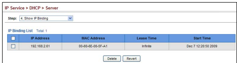
Figure 452: Shows Addresses Assigned by the DHCP Server
