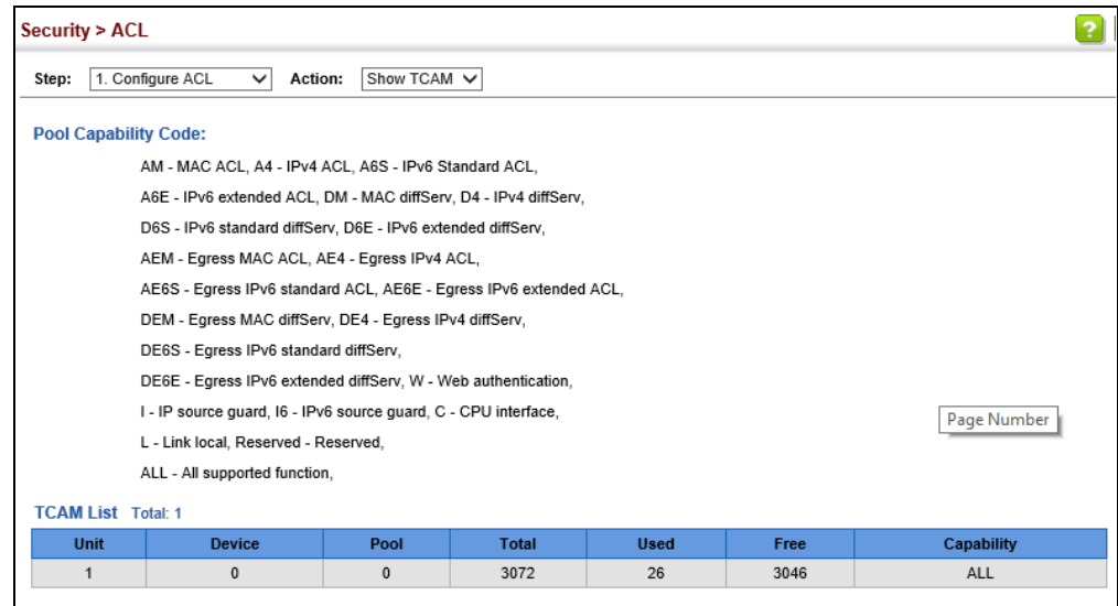
Figure 205: Showing TCAM Utilization
