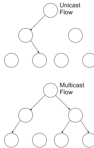
Figure 347: Multicast Filtering Concept
