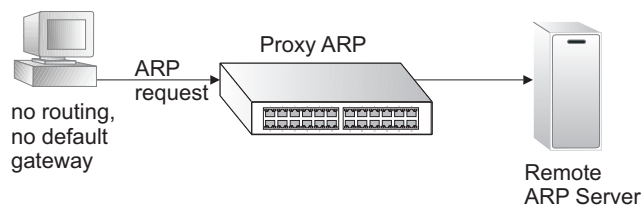
Figure 406: Proxy ARP
