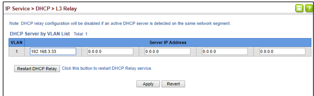
Figure 442: Configuring L3 DHCP Relay Service
