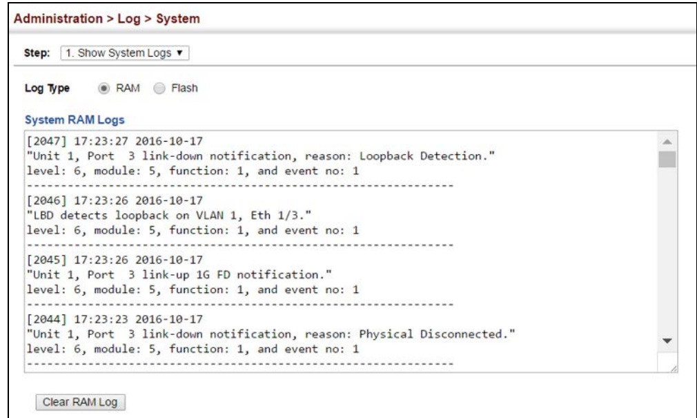
Figure 256: Showing Error Messages Logged to System Memory
