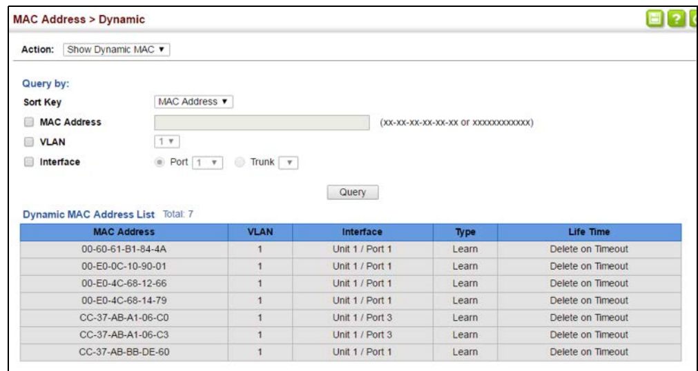
Figure 108: Displaying the Dynamic MAC Address Table
