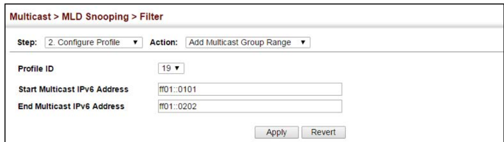
Figure 387: Adding Multicast Groups to an MLD Filtering Profile
