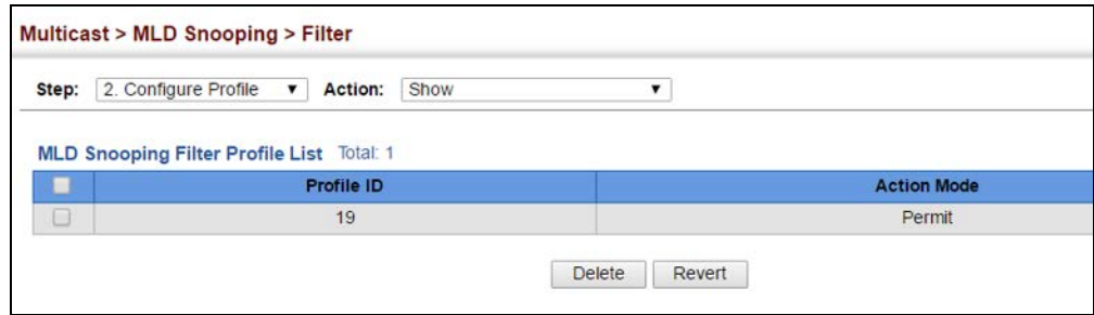
Figure 386: Showing the MLD Filtering Profiles Created
