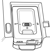
Figure 33 2-Slot USB/Ethernet Cradle Module Switch
