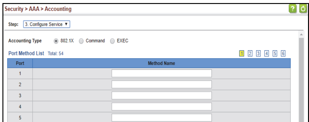
Figure 178: Configuring AAA Accounting Service for 802.1X Service
