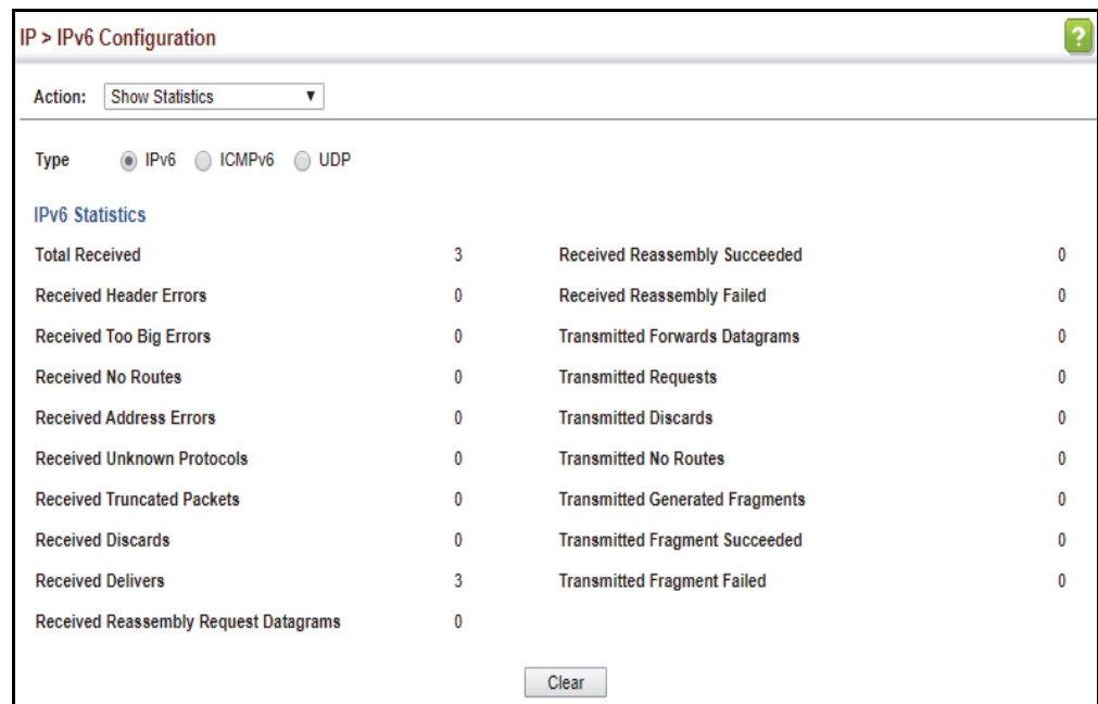
Figure 396: Showing IPv6 Statistics (IPv6)
