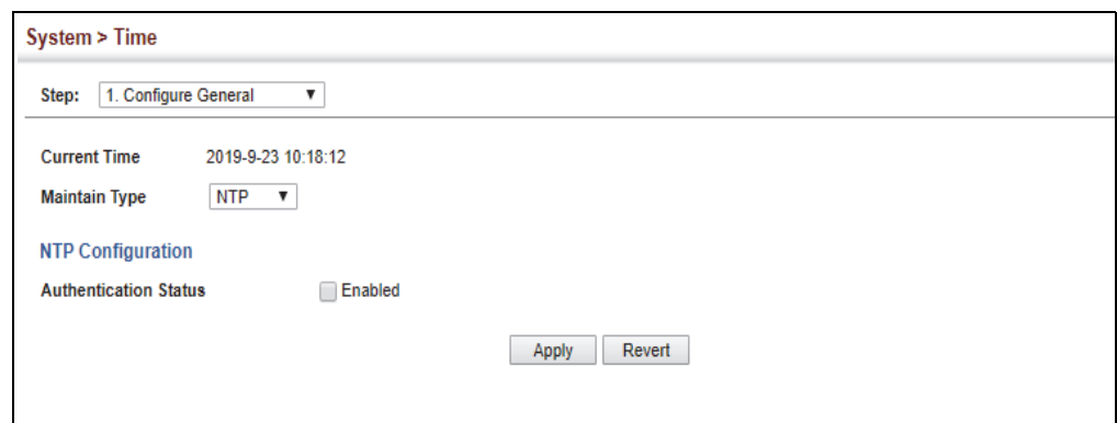
Figure 13: Configuring NTP
