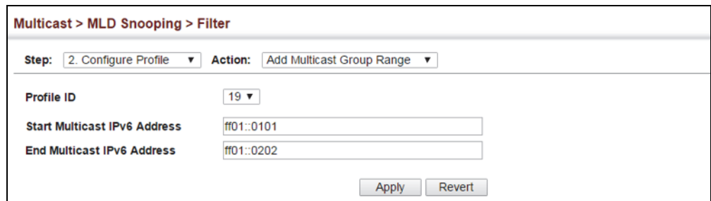
Figure 362: Adding Multicast Groups to an MLD Filtering Profile
