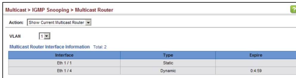
Figure 326: Showing Current Interfaces Attached a Multicast Router
