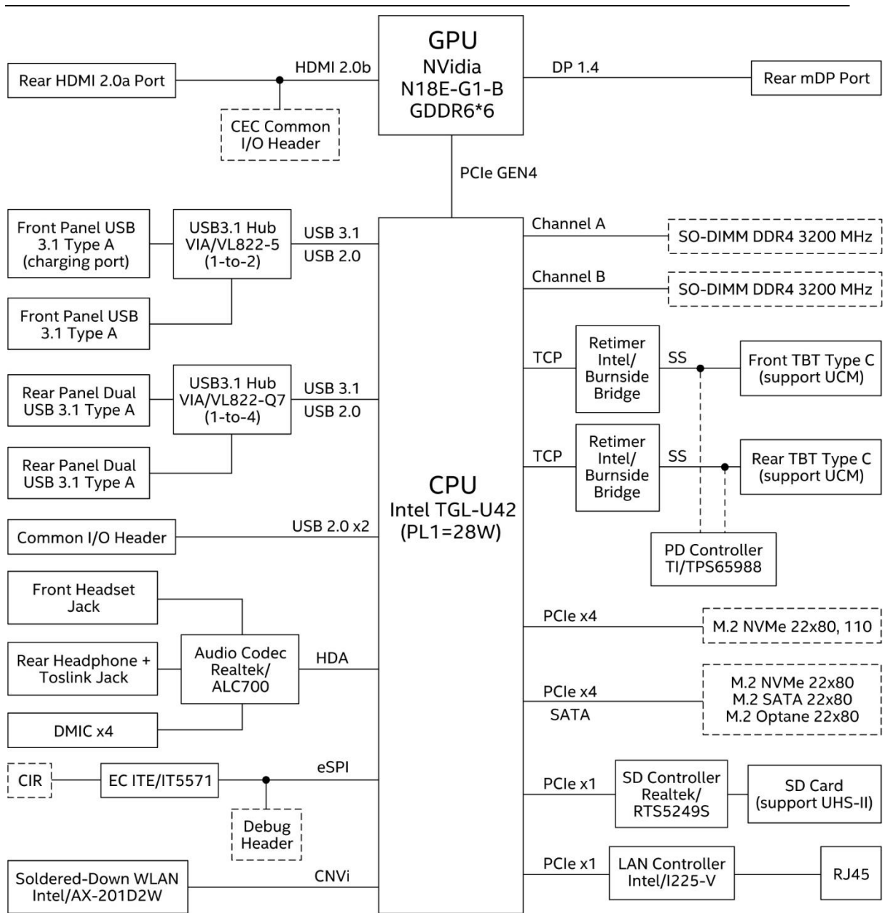
Figure 4. Block Diagram
