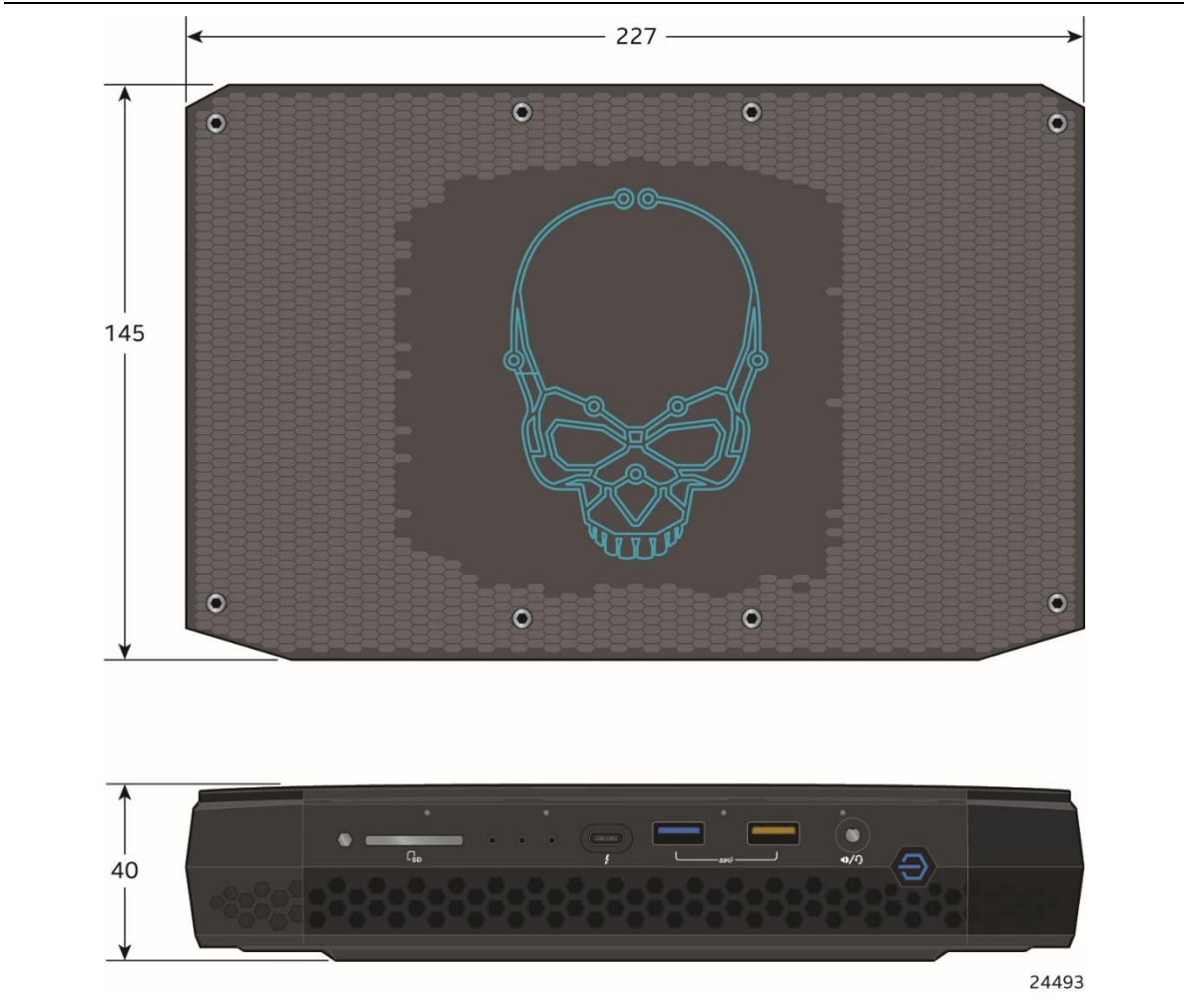
Figure 8. System Dimensions
