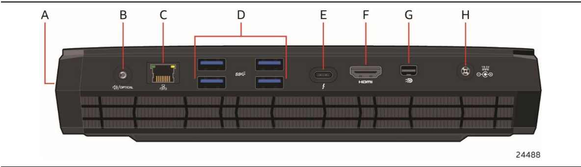
Figure 3. Back Panel Connectors
