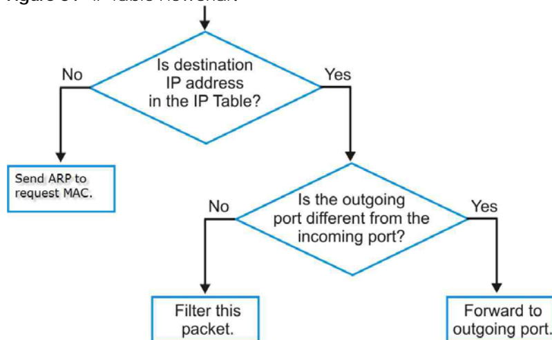
Figure 84 IP Table Flowchart
