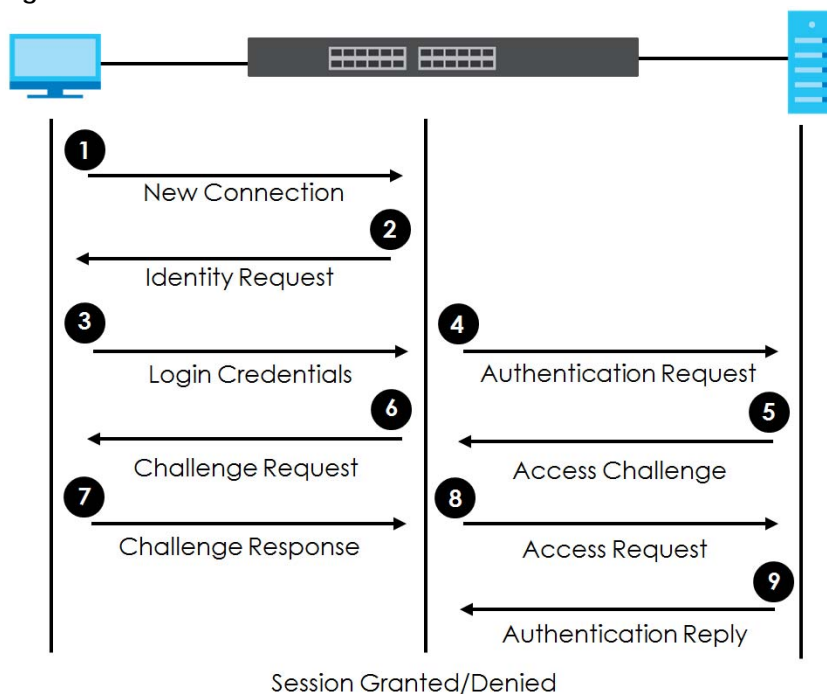
Figure 468 IEEE 802.1x Authentication Process
