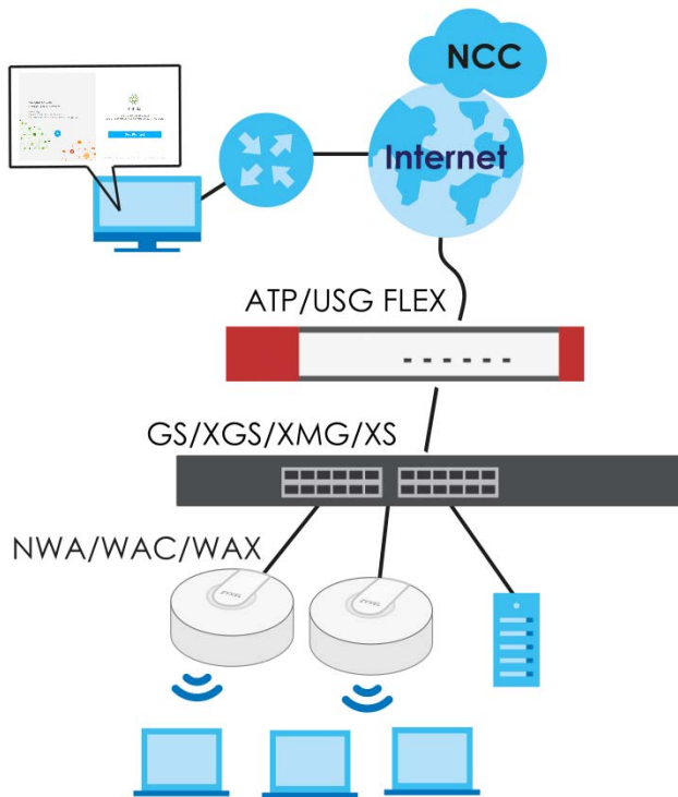
Figure 3 NCC Example Network Topology
