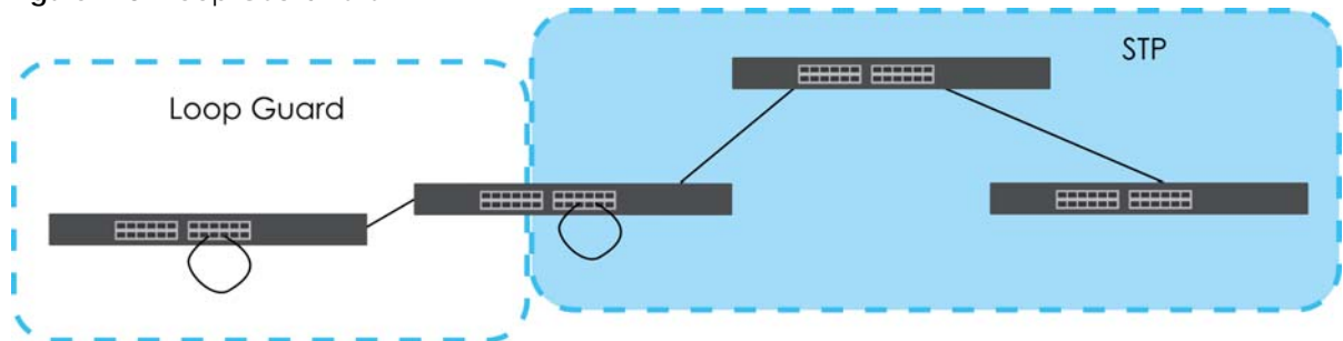
Figure 228 Loop Guard vs. STP
