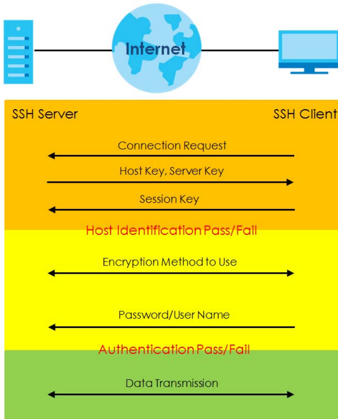
Figure 399 How SSH Works
