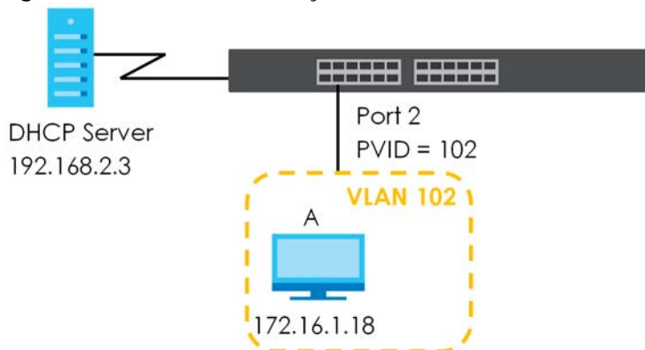
Figure 76 Tutorial: DHCP Relay Scenario
