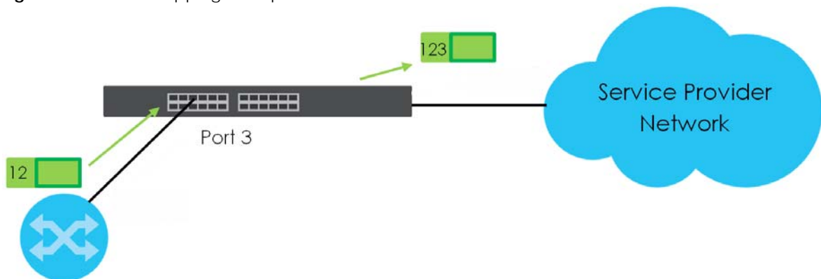
Figure 353 VLAN Mapping Example
