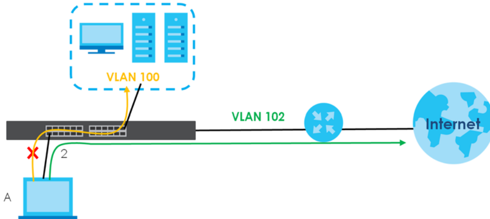
Figure 474 Guest VLAN Example
