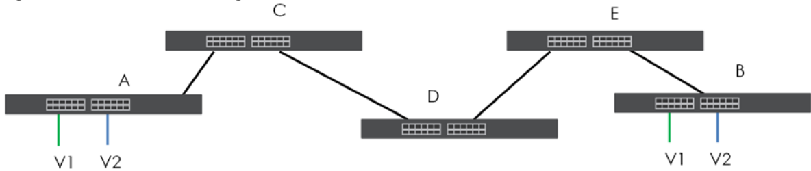
Figure 540 Port VLAN Trunking
