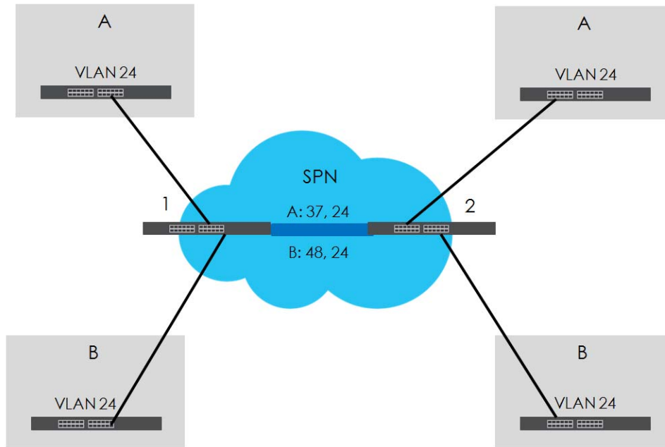
Figure 359 VLAN Stacking Example
