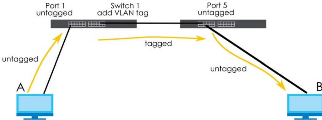
Figure 539 VLAN Forwarding Frame
