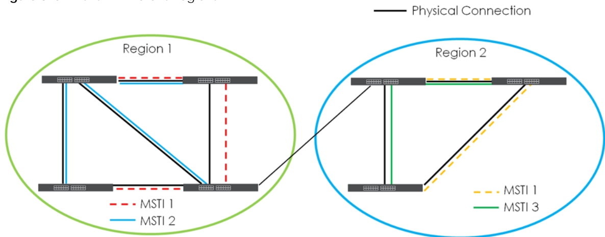
Figure 315 MSTIs in Different Regions
