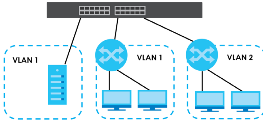
Figure 538 Shared Server Using VLAN Example
