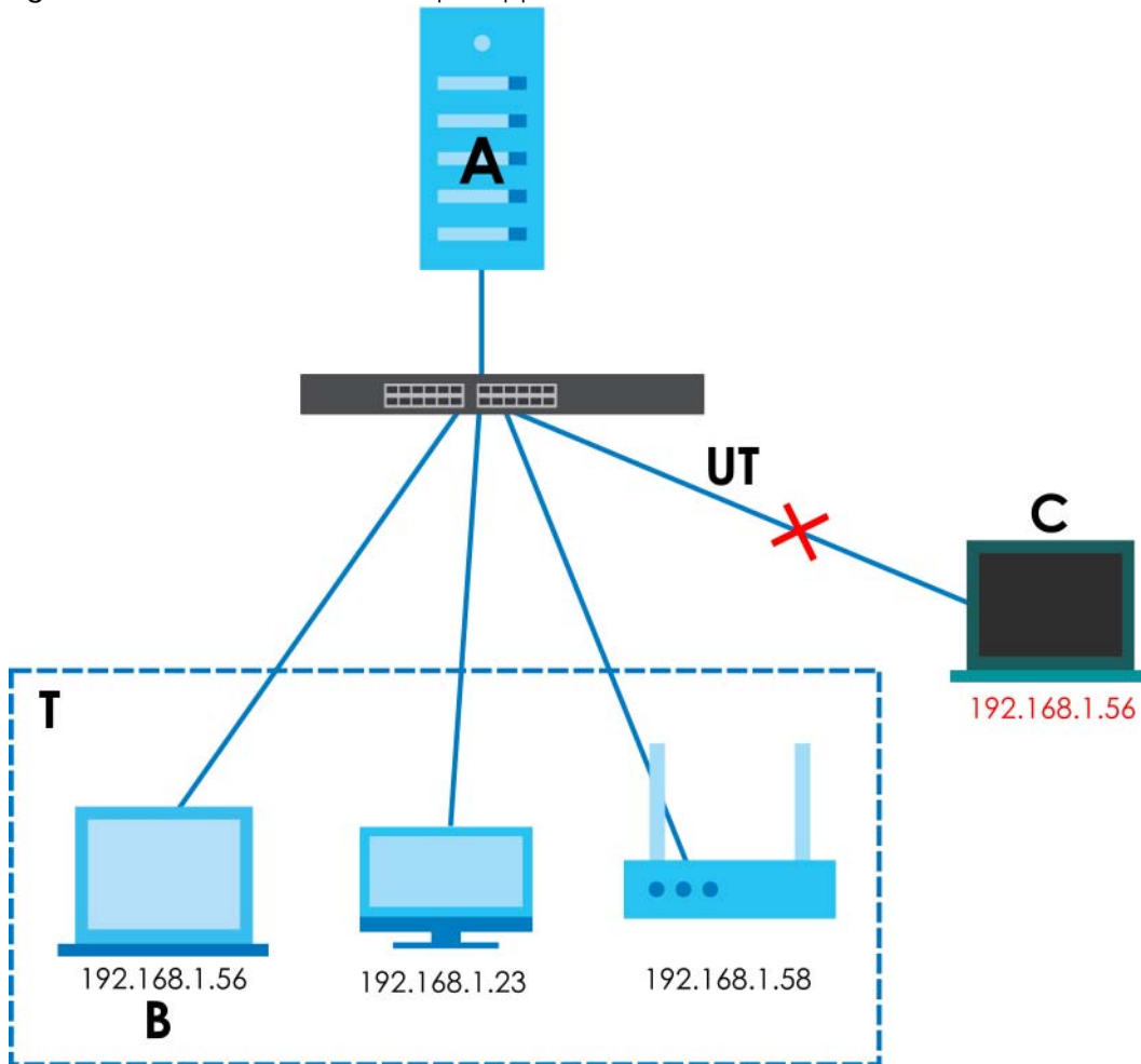
Figure 432 IP Source Guard Example Application
