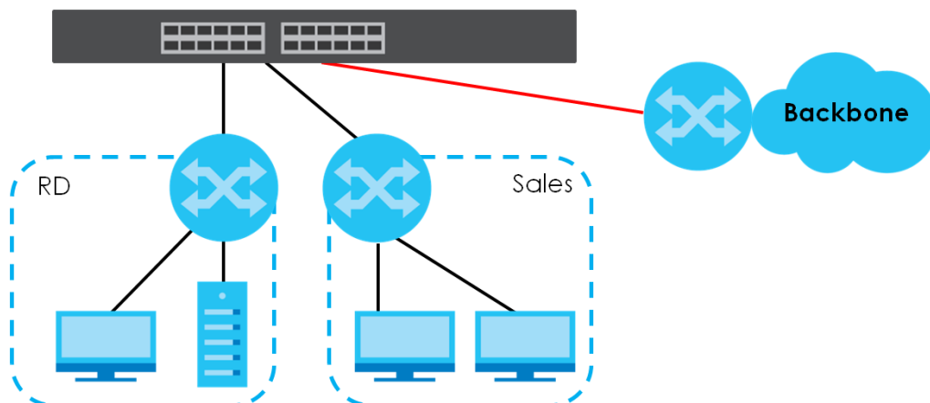
Figure 7 Bridging Application
