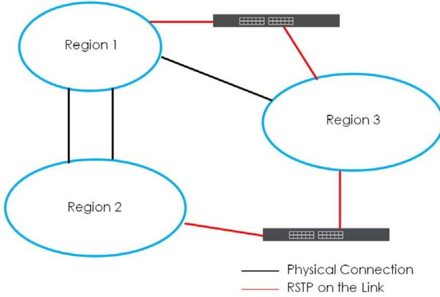
Figure 316 MSTP and Legacy RSTP Network Example
