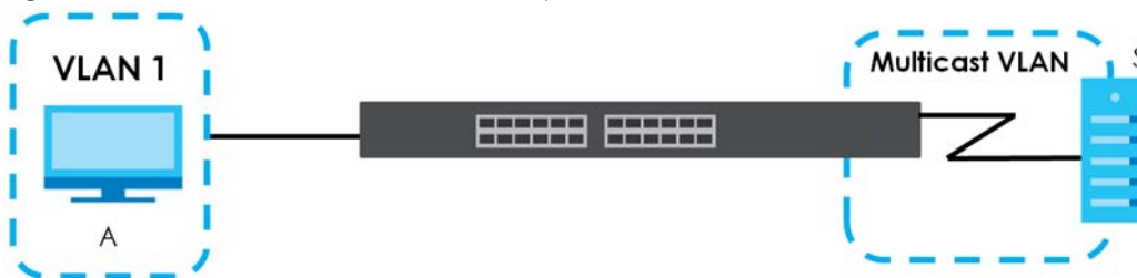
Figure 239 MVR Multicast Television Example
