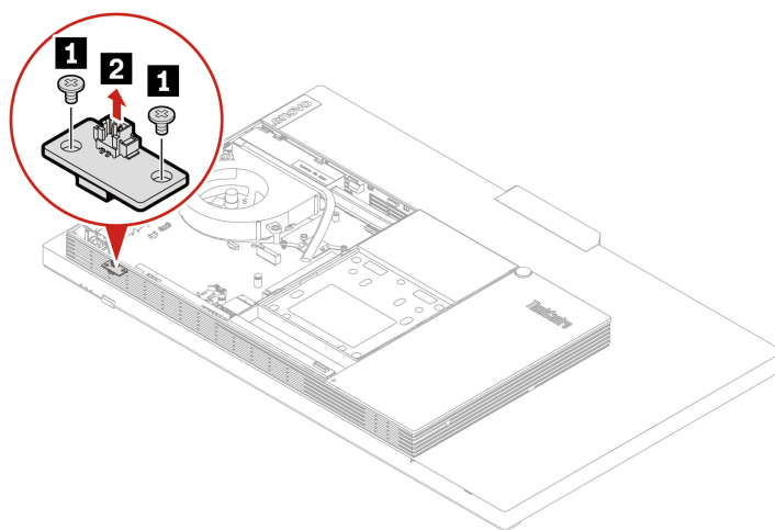
Figure 119. Removing the e-Privacy button board
