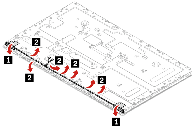
Figure 161. Releasing the Wi-Fi antennas and cables
