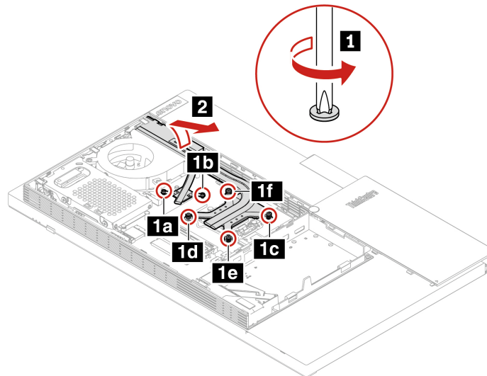
Figure 58. Removing the heat sink
