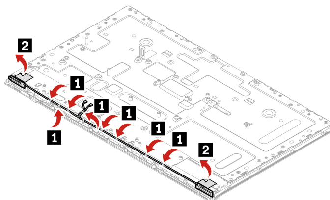
Figure 163. Installing the Wi-Fi antennas
