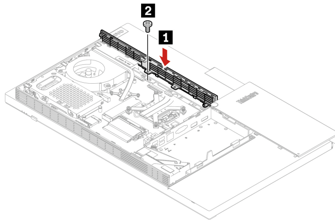
Figure 64. Installing the bump cover
