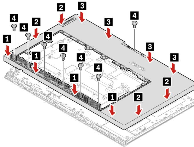
Figure 151. Removing the main frame
