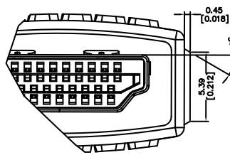
DETAIL A SCALE 8: 1
