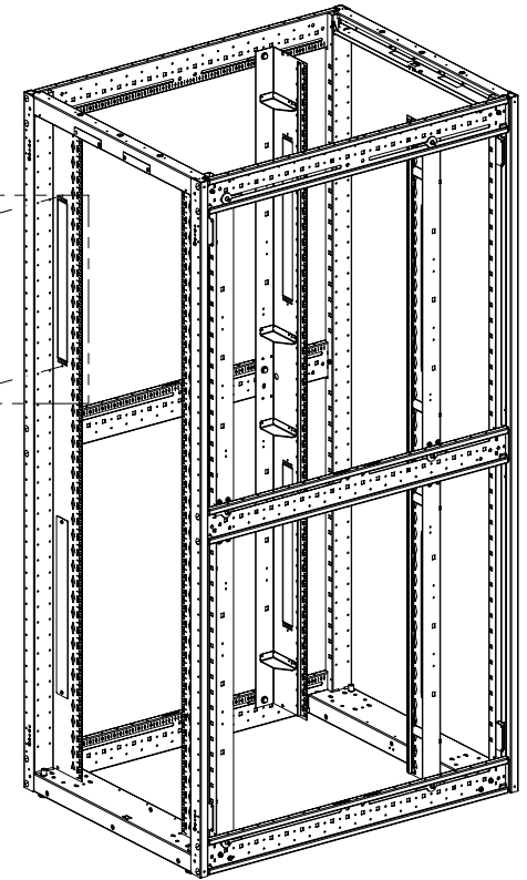
800mm E-RAIL ARRANGEMENT 4 PASS THRU OPENINGS FOR ALL RU SIZED CABINETS 19" X 1RU
