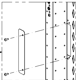
600mm E-RAIL ARRANGEMENT NO PASS THRU OPENINGS
