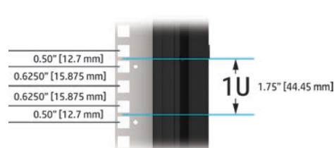
Figure 12. Rack mounting hole positioning in 1U rack space
