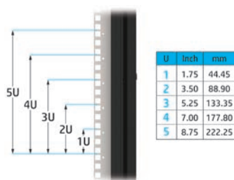
Figure 11. Layout and dimensions of a 5U rack space
