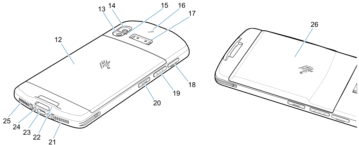
Figure 2 Rear View
