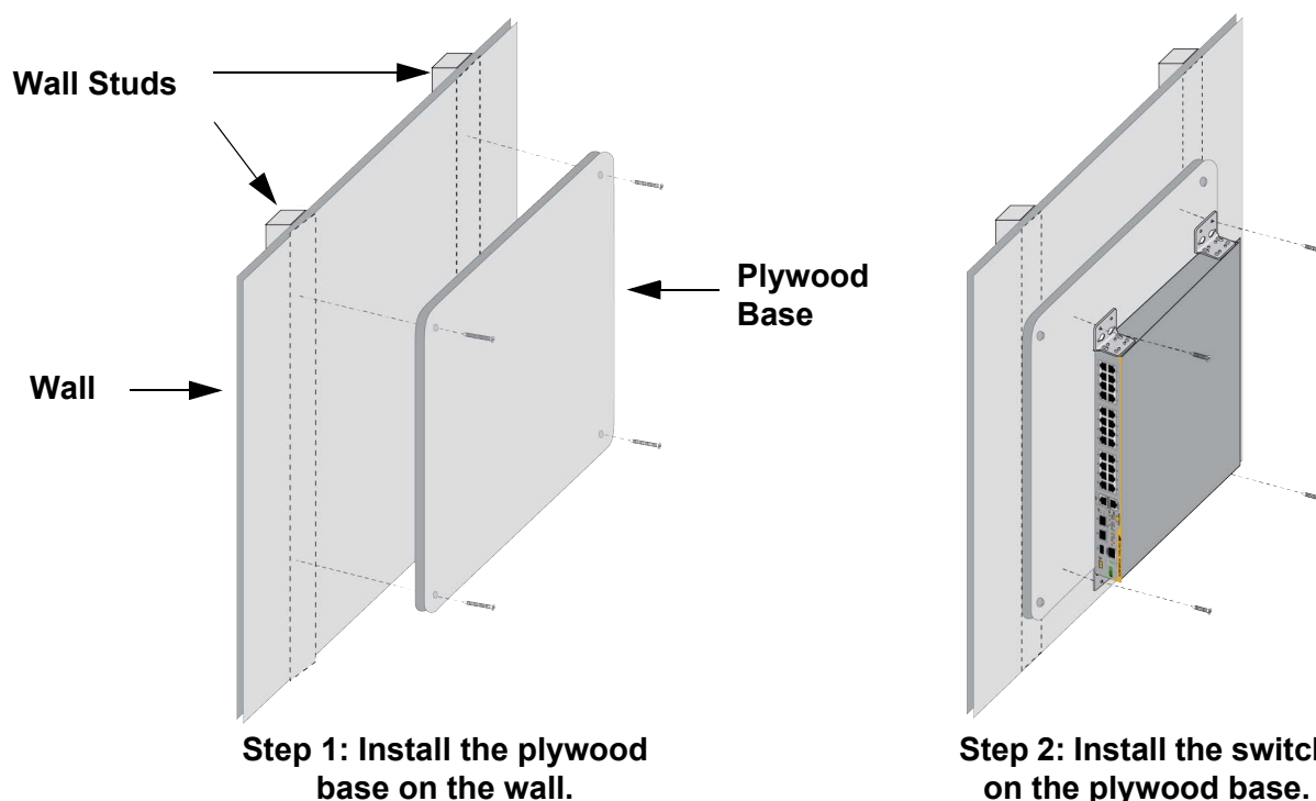
Figure 59. Steps to Installing x330 Switches on a Plywood Base
