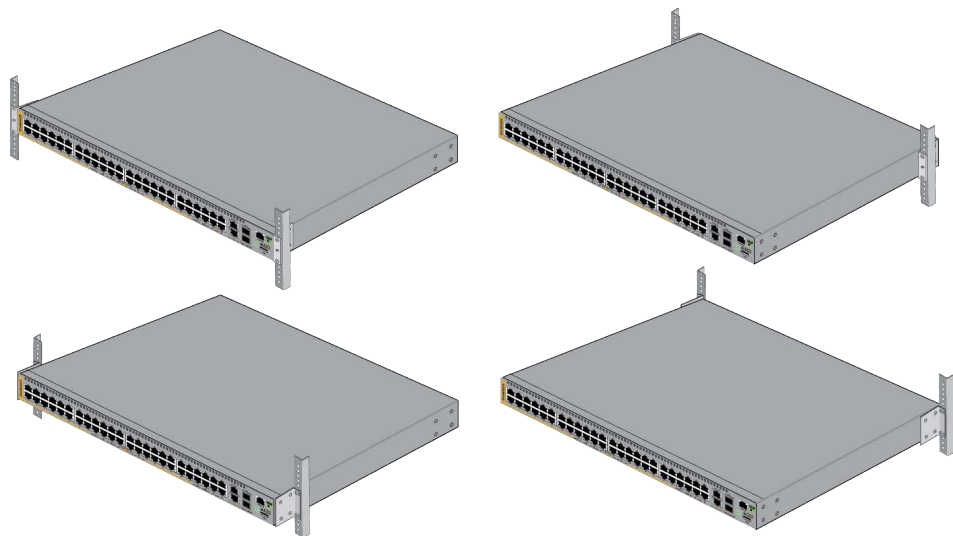
Figure 44. Equipment Rack Bracket Positions for the x330-52GTX Switch
