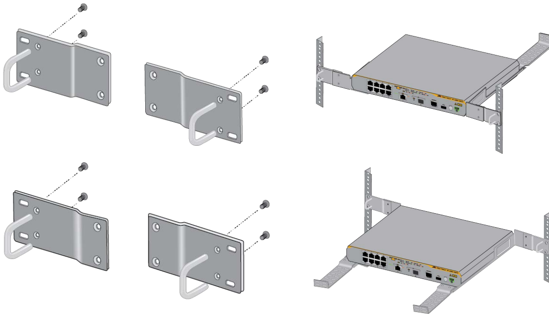
Figure 30. Attaching the RKMT-J05 Handles to the Short Brackets
