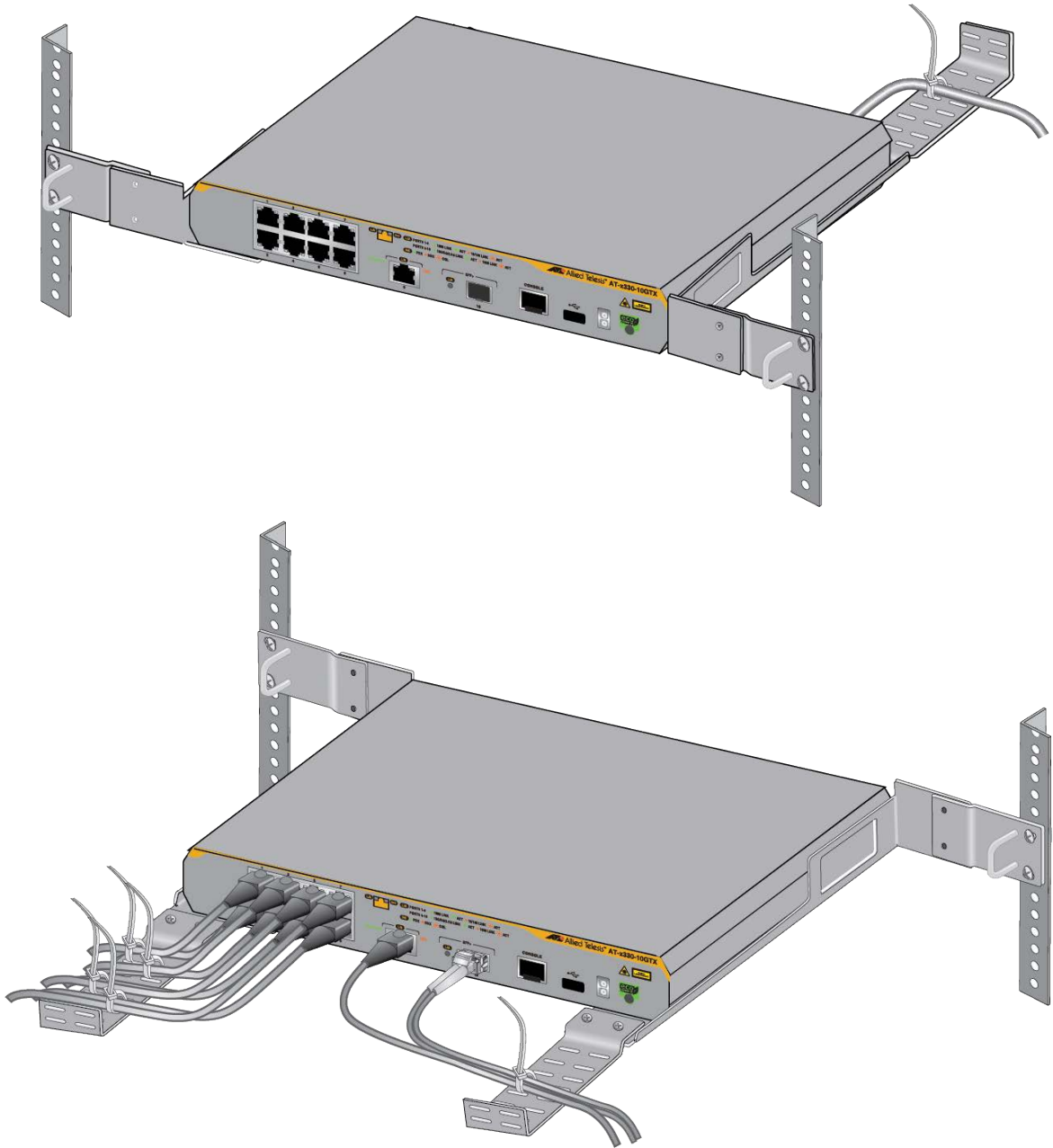
Figure 29. x330-10GTX Switch with RKMT-J05 Cable Trays
