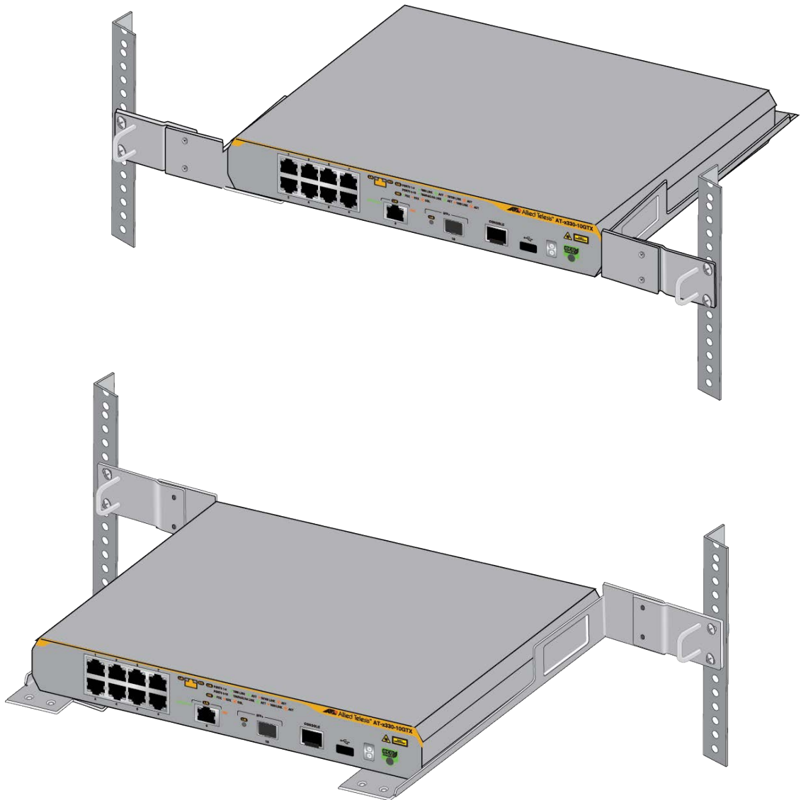
Figure 28. x330-10GTX Switch in an Equipment Rack with the RKMT-J05 Brackets Kit
