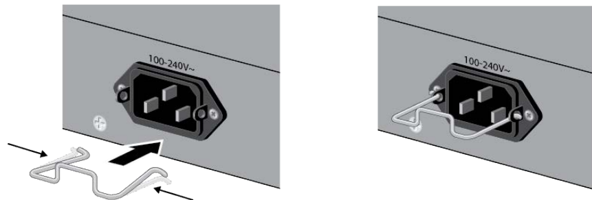
Figure 64. Installing the Power Cord Retaining Clip
