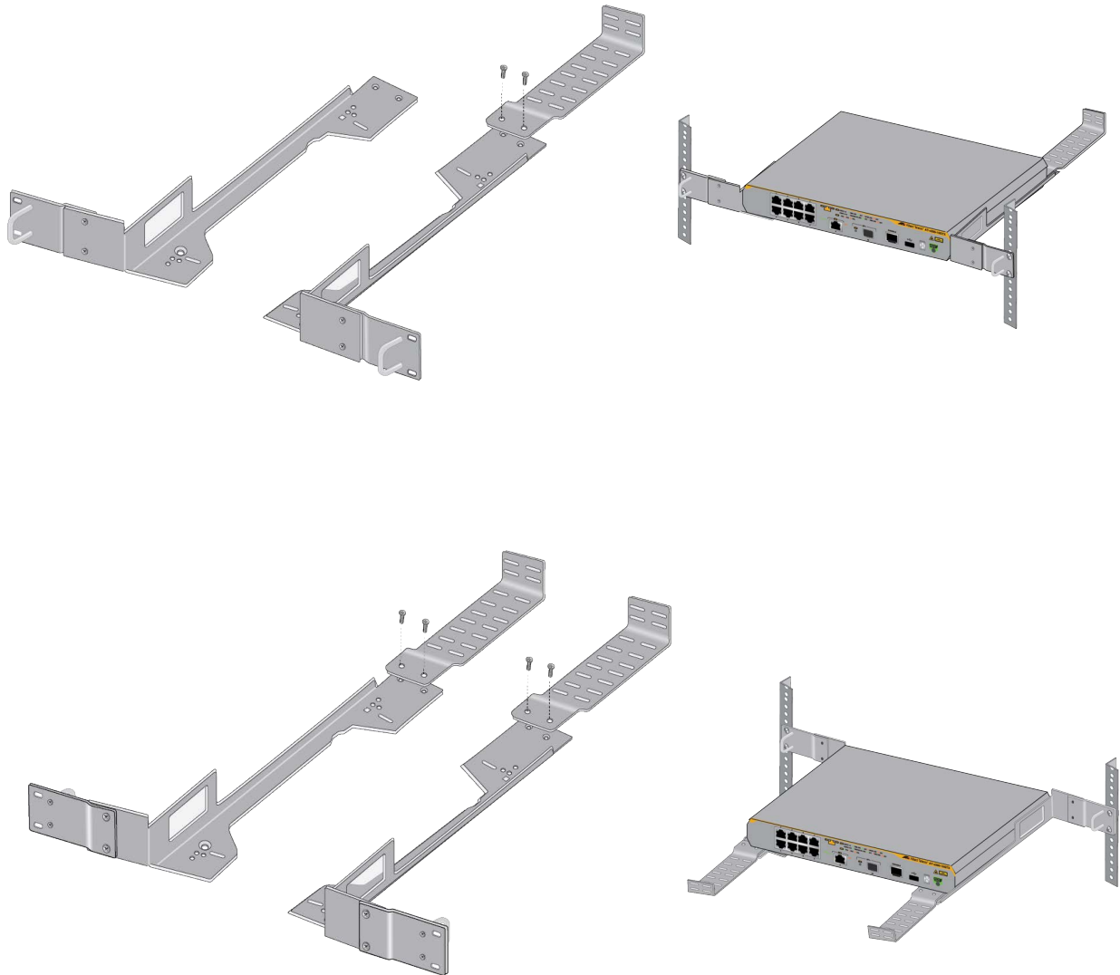
Figure 32. Attaching the RKMT-J05 Cord Trays to the Long Brackets
