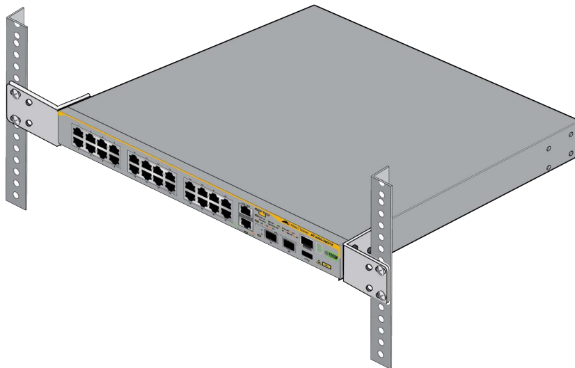
Figure 40. x330-28GTX Switch in Standard 19-inch Equipment Racks
