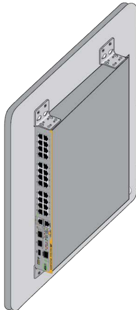
Figure 17. Installation Options for the x330-28GTX Switch
