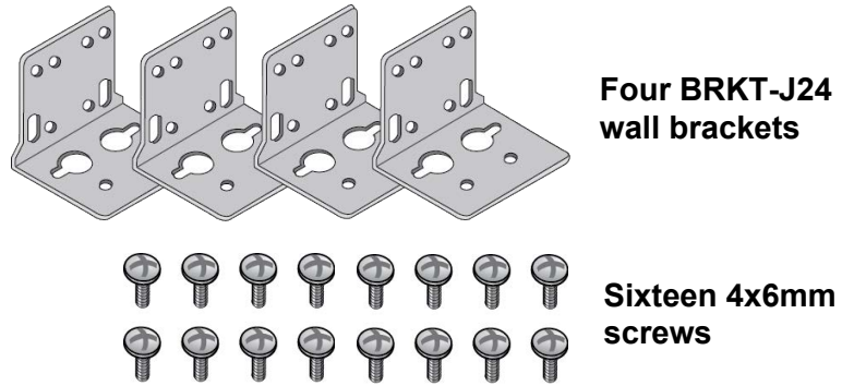
Figure 22. BRKT-J24 Wall Brackets Kit for the x330-20GTX and x330-28GTX Switches
