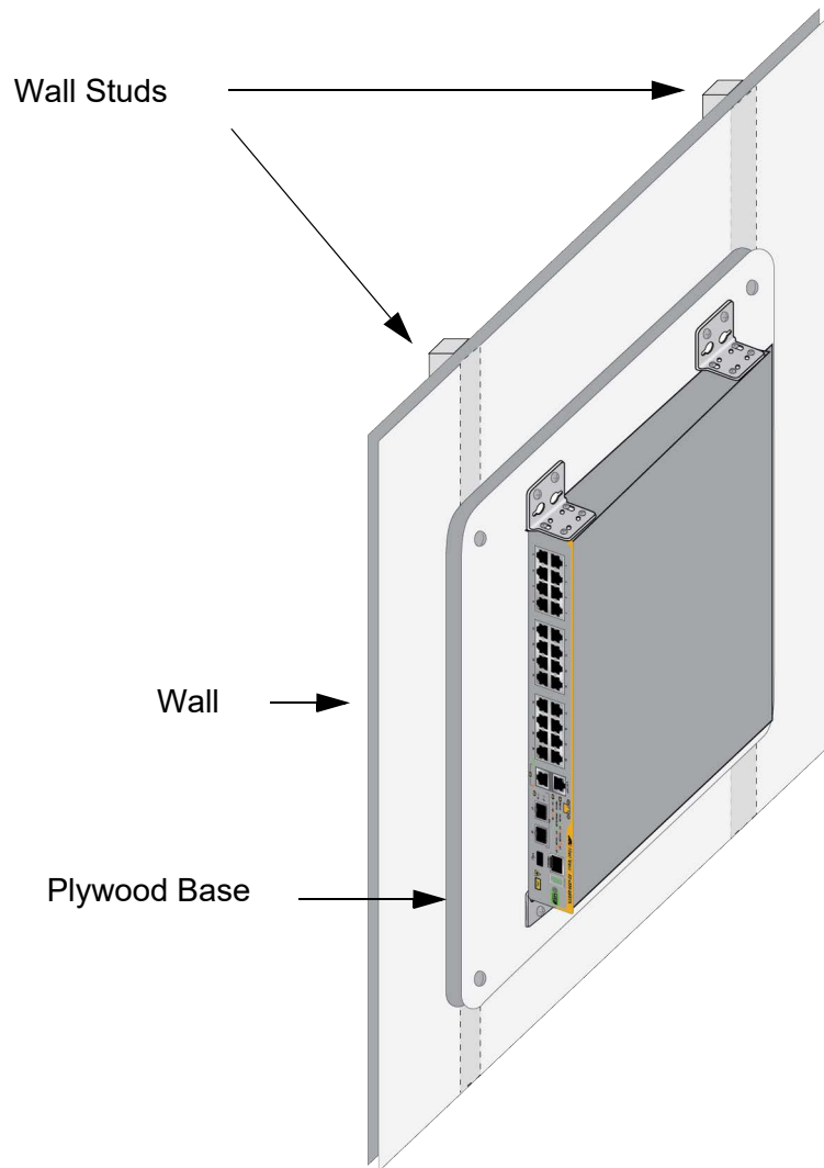
Figure 58. x330 Switch on a Wall with a Plywood Base
