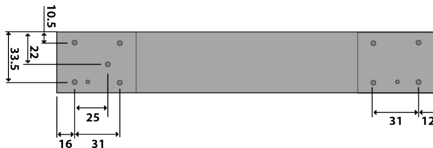
Figure 83. Bracket Screw Holes on the x330-20GTX and x330-28GTX Switches
