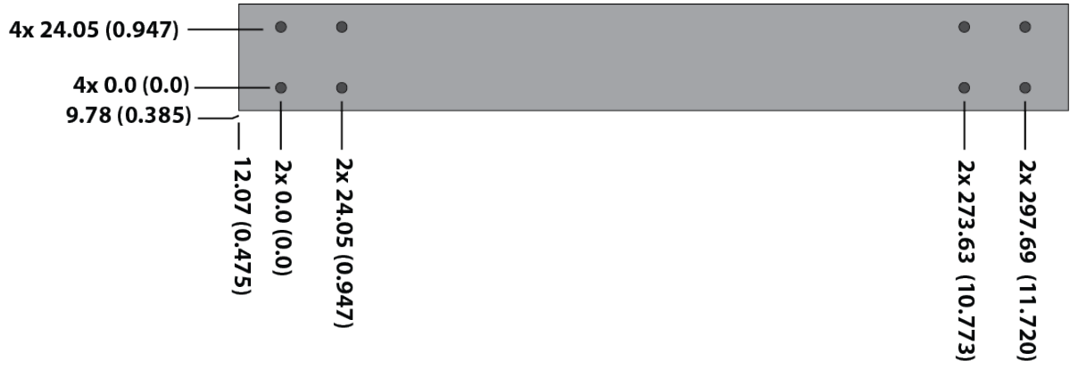
Figure 84. Bracket Screw Holes on the x330-52GTX Switch
