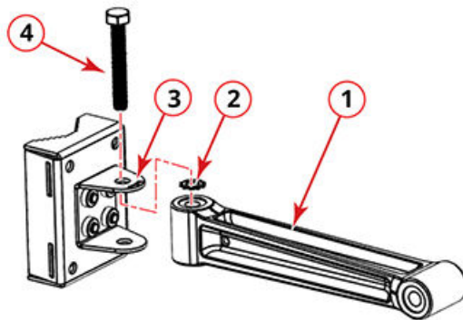
FIGURE 7 Attaching the linkage bracket to the U-joint bracket
