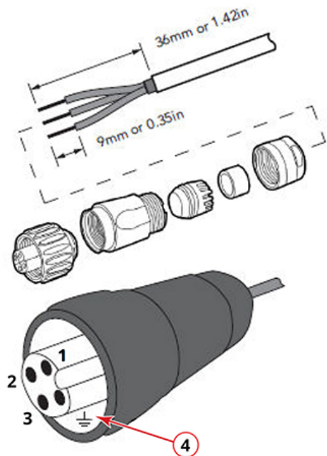
FIGURE 10 Assembling the AC power connector
