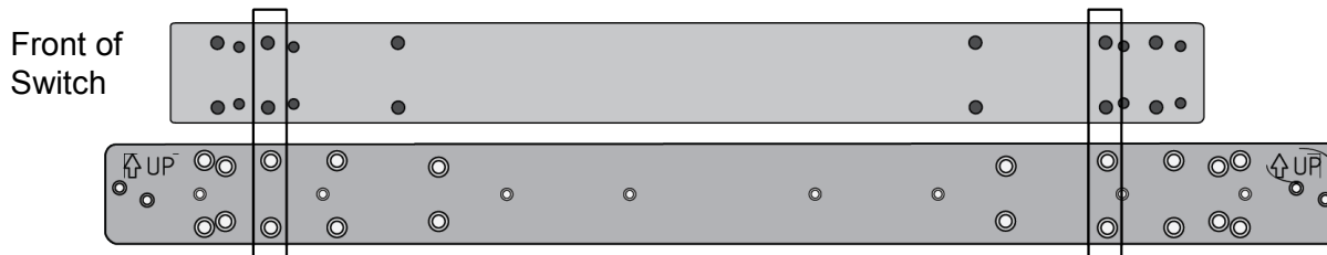
Figure 97. Inner Rail Screw Holes for the x950-52XSQ and x950-52XTQm Switches
