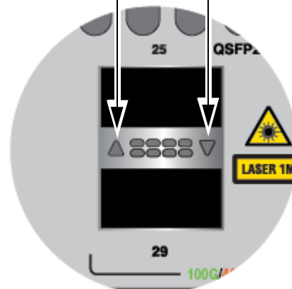
Figure 8. LEDs for Ports 25, 29, 33, and 37 on the x950-28XSQ and x950-28XTQm Switches
