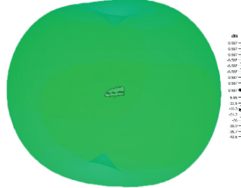
3D Pattern All Elements (2000MHz)
