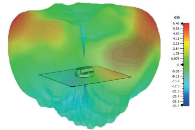
Typical 3D Pattern - 4G/5G Elements 2000MHz
