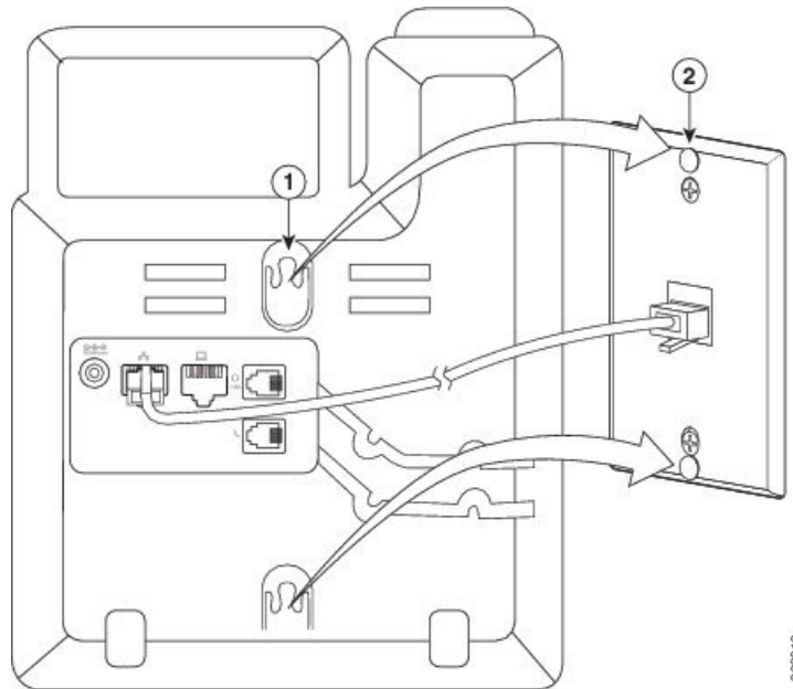
Figure 24: Mounting Holes
