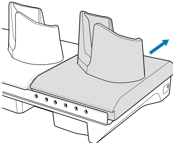
Figure 48 Remove Cup
